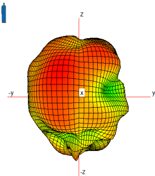
3D Antenna pattern
