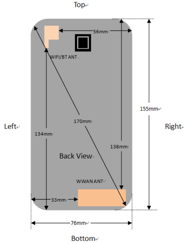
Fig.14.1 EUT Antenna Locations
