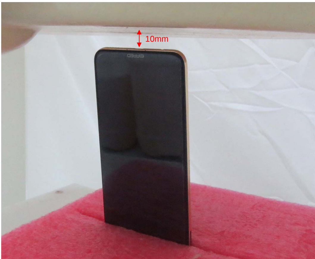
Picture 12: Bottom Side, the distance from handset to the bottom of the Phantom is 10mm
