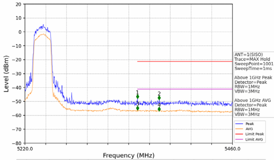
802.11ax(HEW20)_HCH_5240MHz_RU242_Left_Ant1_NTNV
