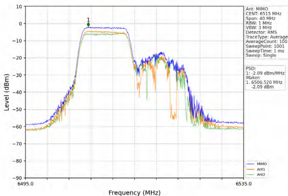
802.11ax(HEW20)_HCH_6515MHz_RU106_Right_MIMO_NTNV
