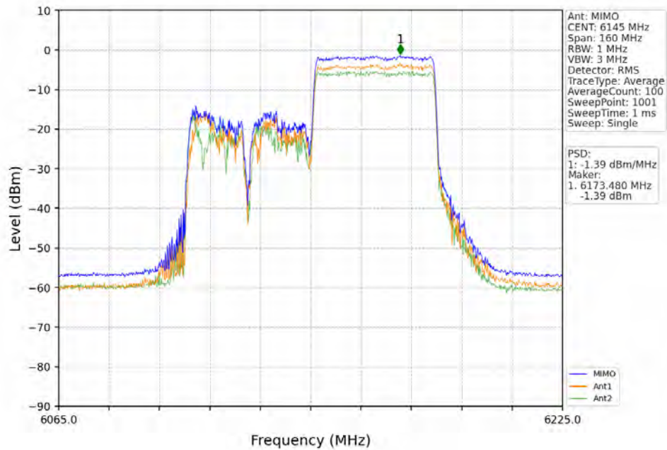
802.11ax(HEW80)_MCH_6145MHz_RU996_Left_MIMO_NTNV
