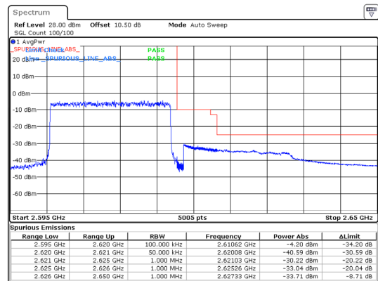
Band 38 15MHz/2577.5/Low 16QAM 75@0
