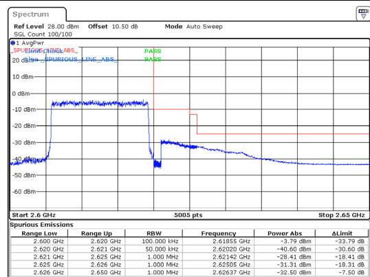
Band 38 15MHz/2612.5/High QPSK 75@0
