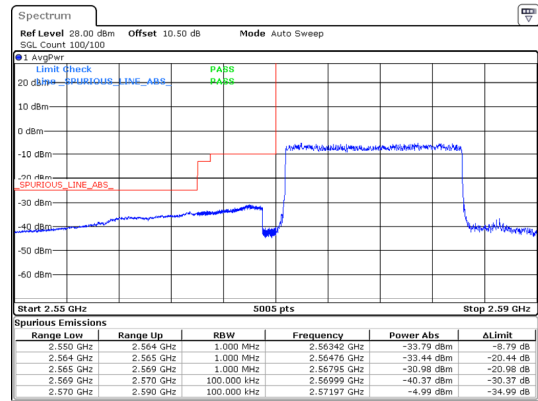
Band 38 15MHz/2577.5/Low QPSK 75@0
