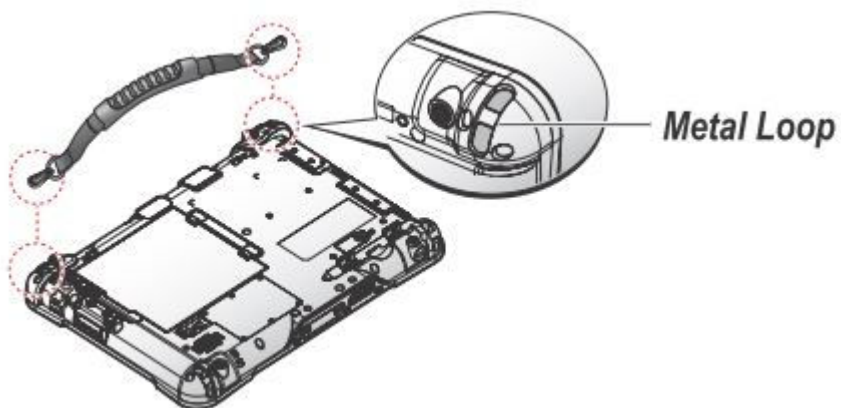
Figure 38. Removing the Carrying Handle
