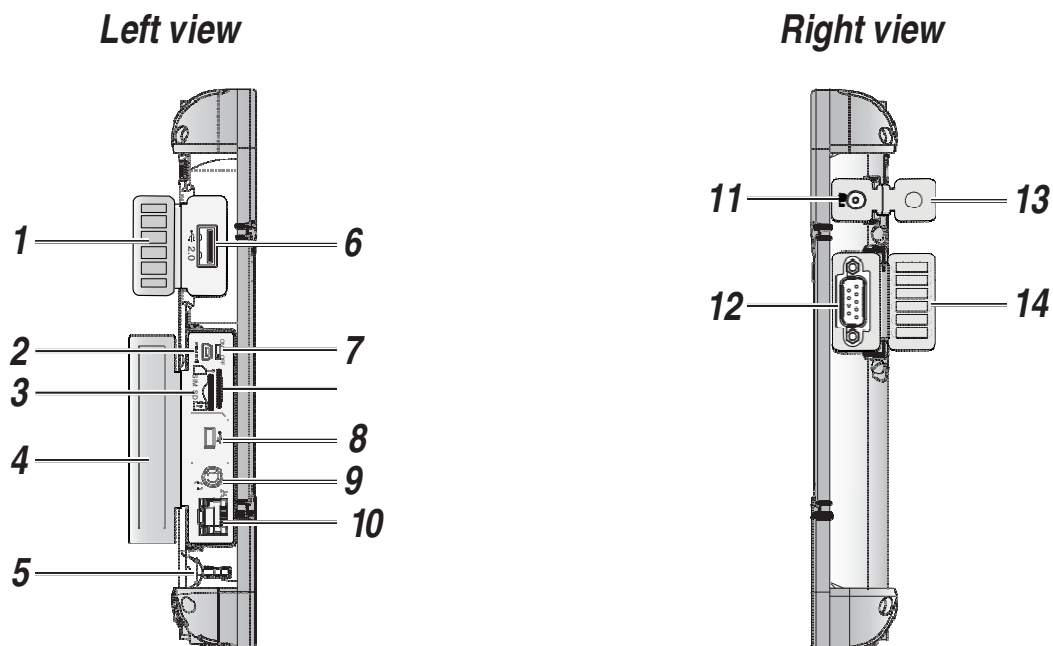
Figure 4. Side Views
