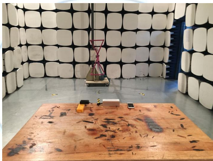
Radiated Emission
