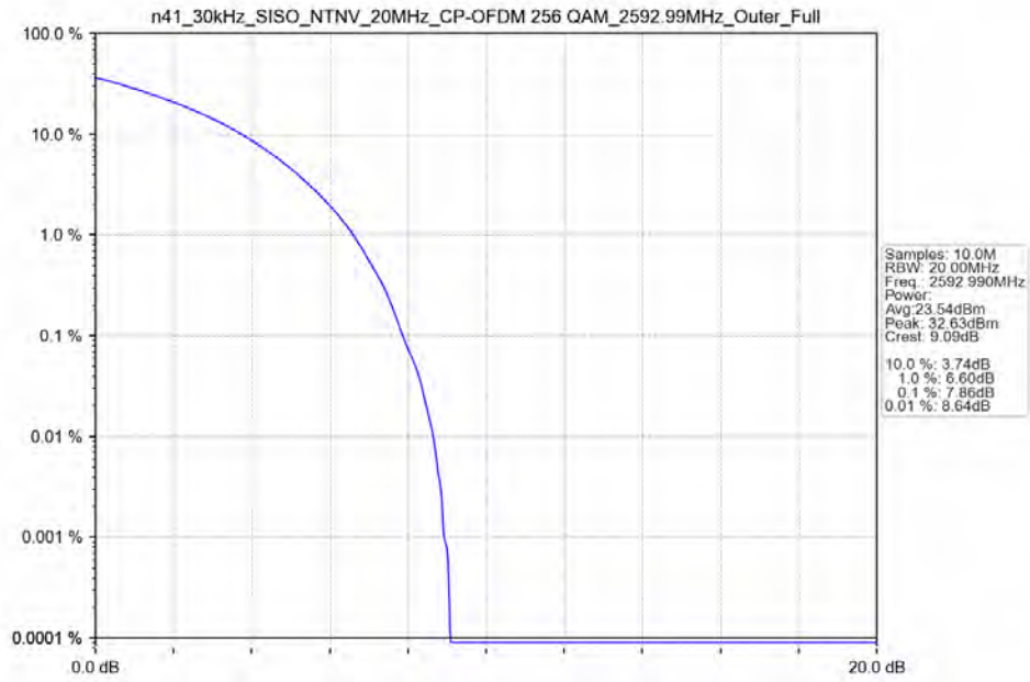
n41_30kHz_SISO_NTNV_20MHz_CP-OFDM_256_QAM_2592.99MHz_Outer_Full_Ant41
