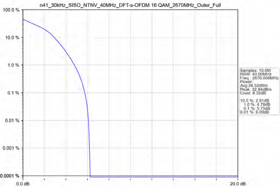
n41_30kHz_SISO_NTNV_40MHz_DFT-s-OFDM_16_QAM_2670MHz_Outer_Full_Ant41
