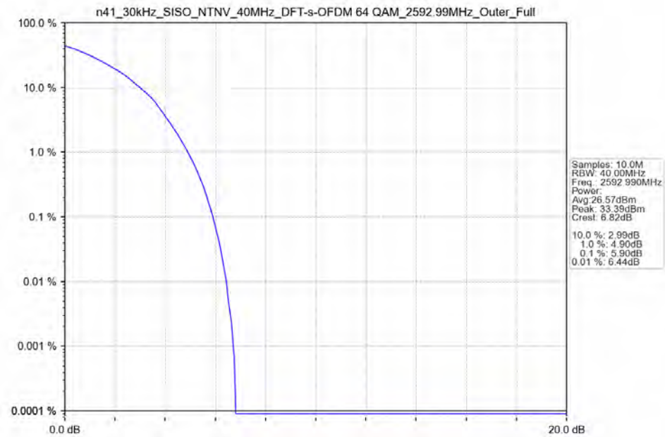
n41_30kHz_SISO_NTNV_40MHz_DFT-s-OFDM_64_QAM_2592.99MHz_Outer_Full_Ant41
