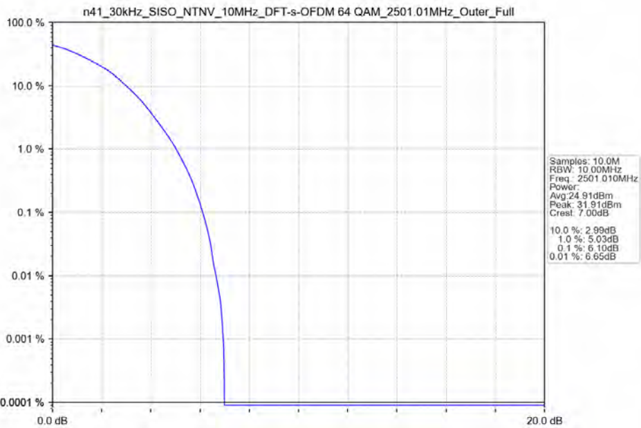
n41_30kHz_SISO_NTNV_10MHz_DFT-s-OFDM_64_QAM_2501.01MHz_Outer_Full_Ant41
