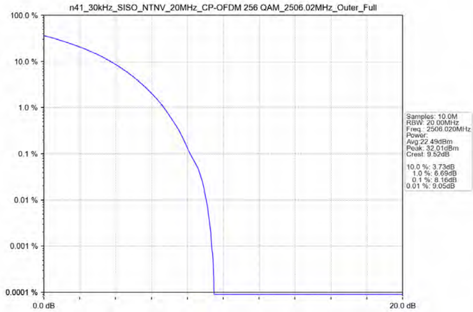
n41_30kHz_SISO_NTNV_20MHz_CP-OFDM_256_QAM_2506.02MHz_Outer_Full_Ant41
