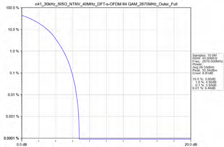
n41_30kHz_SISO_NTNV_40MHz_DFT-s-OFDM_64_QAM_2670MHz_Outer_Full_Ant41
