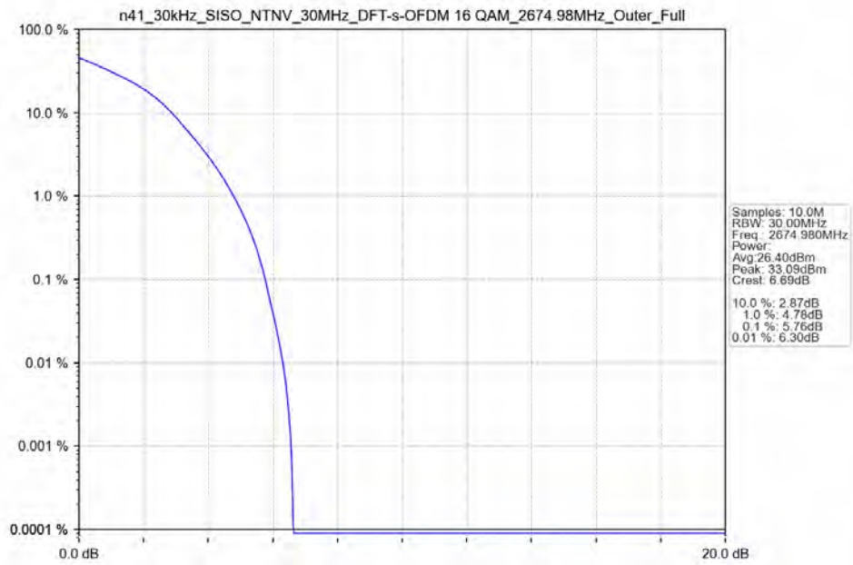
n41_30kHz_SISO_NTNV_30MHz_DFT-s-OFDM_16_QAM_2674.98MHz_Outer_Full_Ant41
