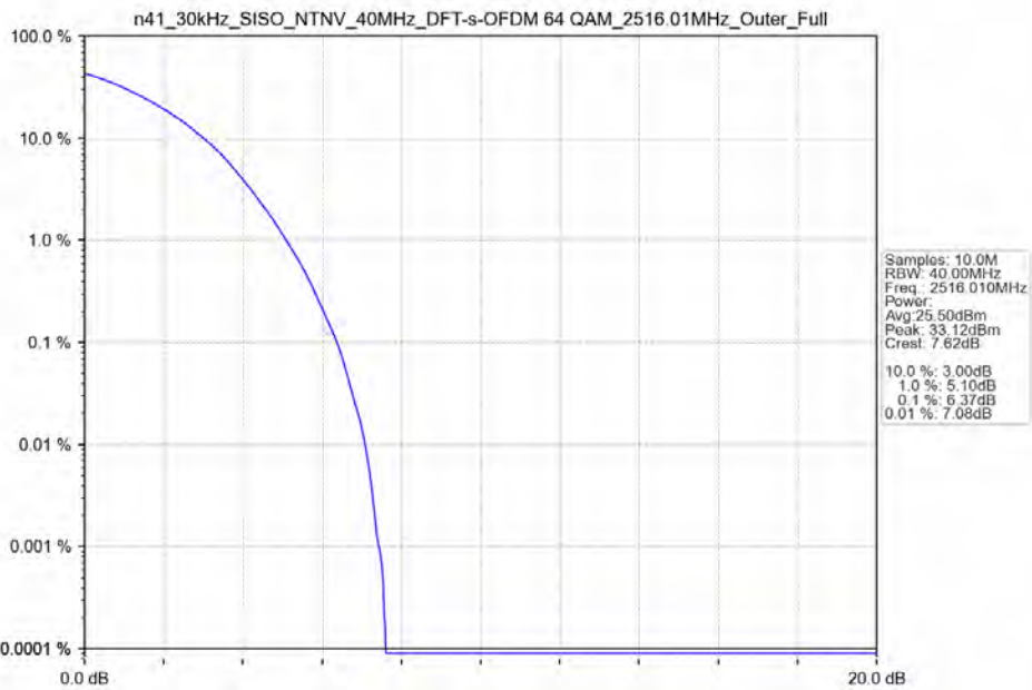
n41_30kHz_SISO_NTNV_40MHz_DFT-s-OFDM_64_QAM_2516.01MHz_Outer_Full_Ant41
