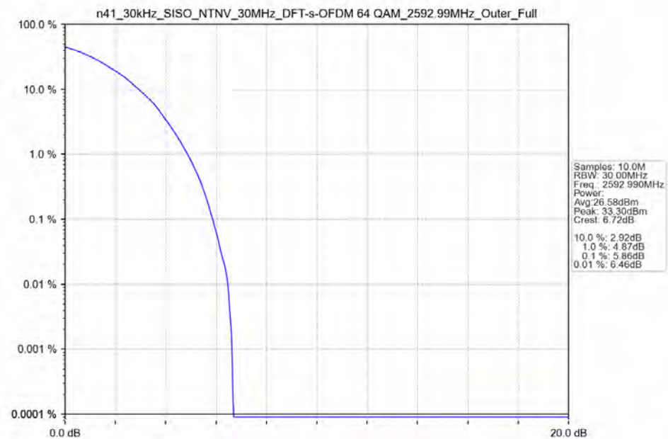
n41_30kHz_SISO_NTNV_30MHz_DFT-s-OFDM_64_QAM_2592.99MHz_Outer_Full_Ant41
