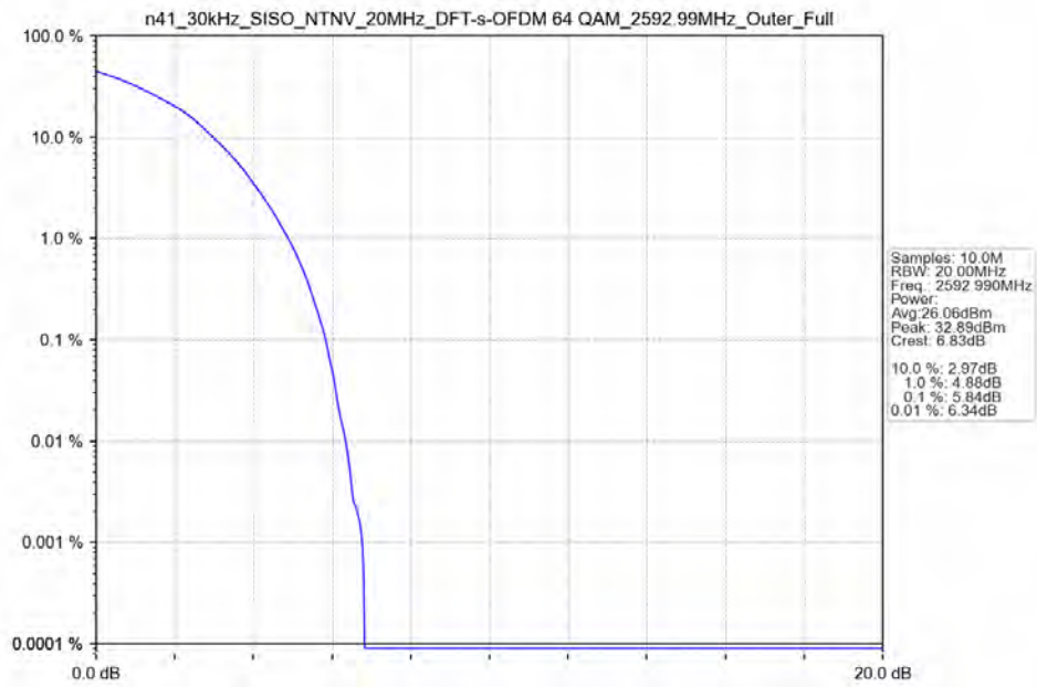
n41_30kHz_SISO_NTNV_20MHz_DFT-s-OFDM_64_QAM_2592.99MHz_Outer_Full_Ant41
