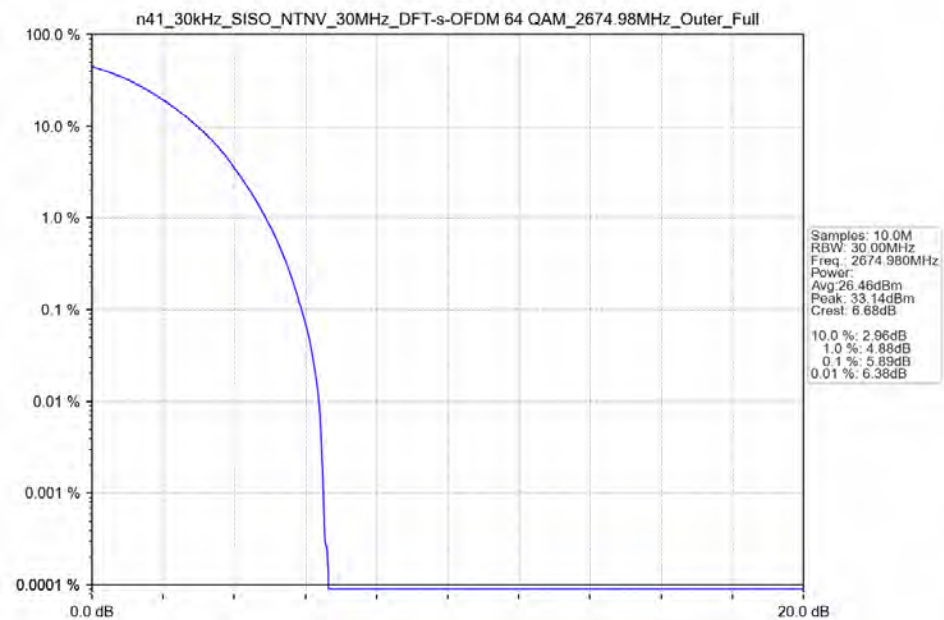
n41_30kHz_SISO_NTNV_30MHz_DFT-s-OFDM_64_QAM_2674.98MHz_Outer_Full_Ant41
