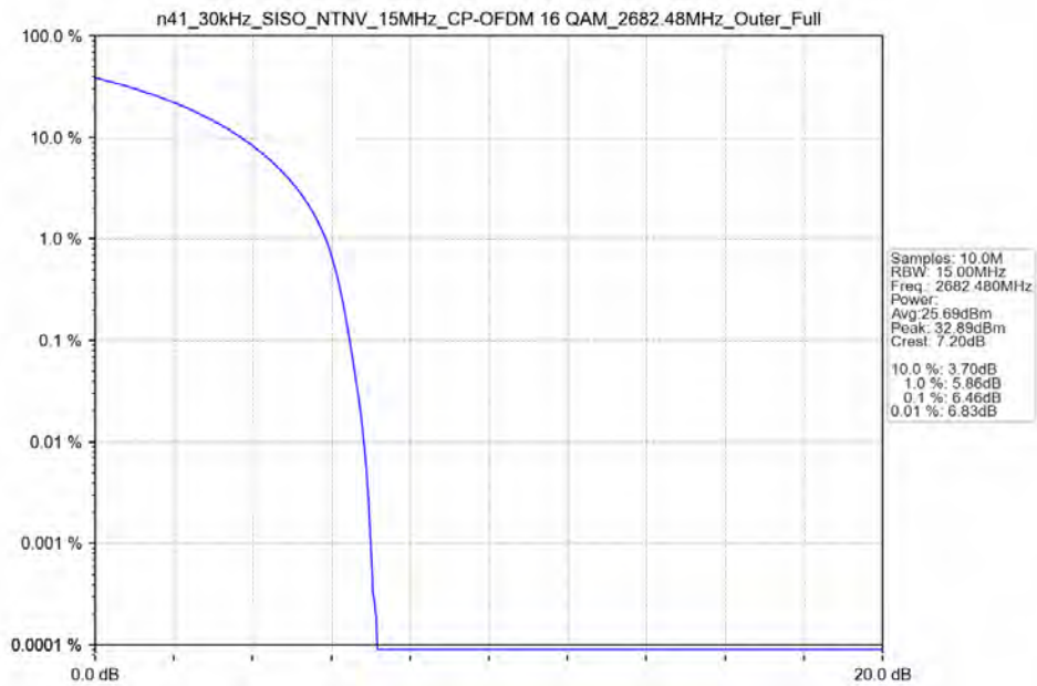
n41_30kHz_SISO_NTNV_15MHz_CP-OFDM 16 QAM 2682.48MHz_Outer_Full_Ant41
