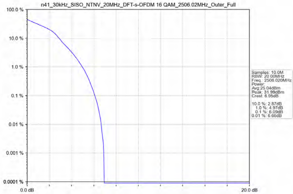
n41_30kHz_SISO_NTNV_20MHz_DFT-s-OFDM_16_QAM_2506.02MHz_Outer_Full_Ant41
