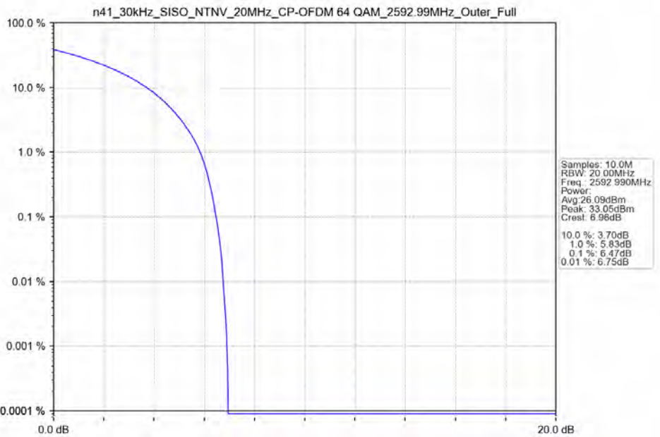
n41_30kHz_SISO_NTNV_20MHz_CP-OFDM 64 QAM 2592.99MHz_Outer_Full_Ant41
