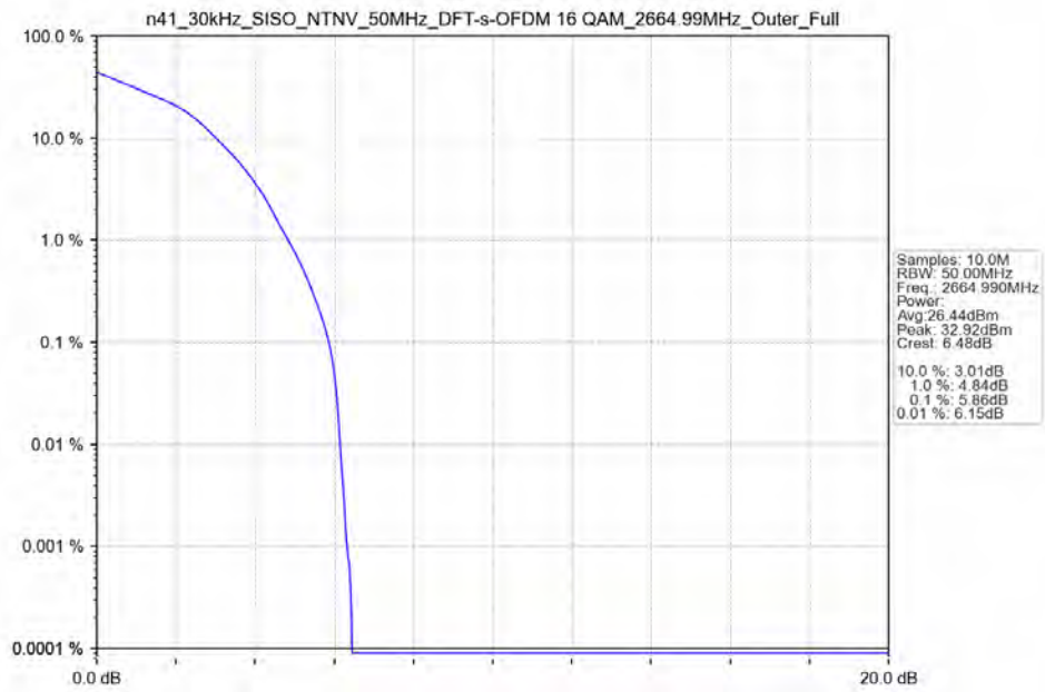
n41_30kHz_SISO_NTNV_50MHz_DFT-s-OFDM_16_QAM_2664.99MHz_Outer_Full_Ant41
