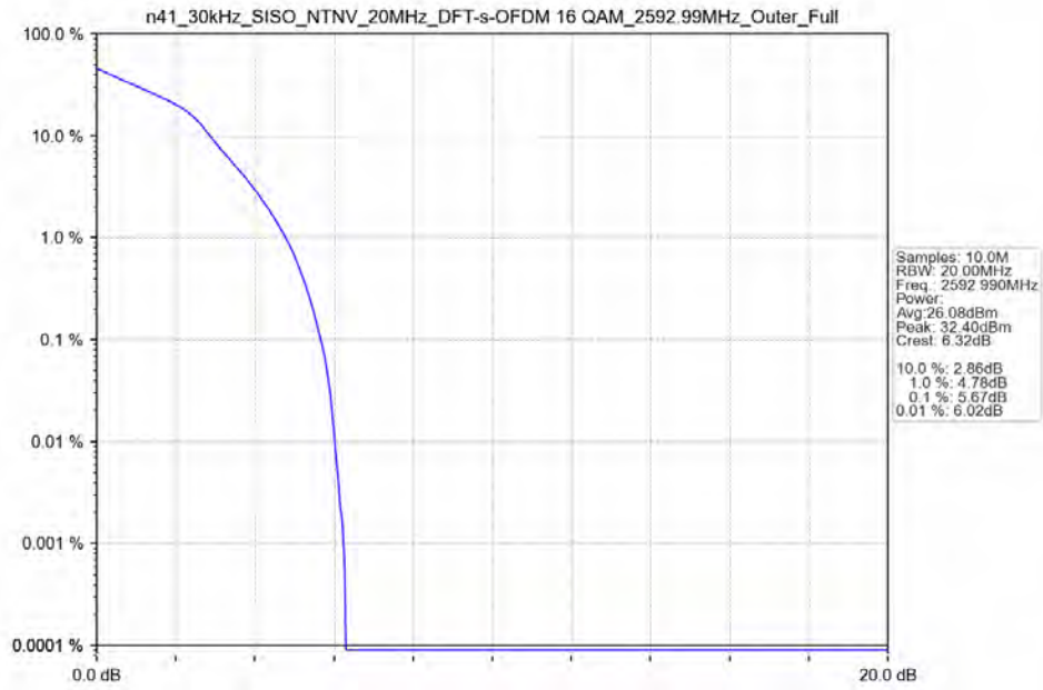
n41_30kHz_SISO_NTNV_20MHz_DFT-s-OFDM_16_QAM_2592.99MHz_Outer_Full_Ant41
