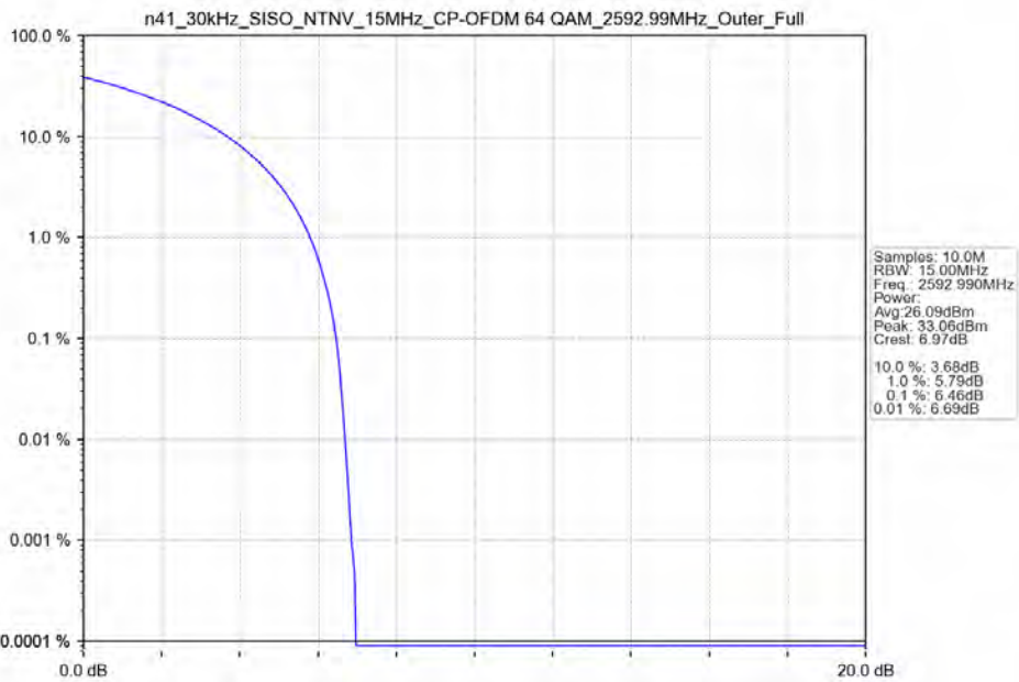
n41_30kHz_SISO_NTNV_15MHz_CP-OFDM_64_QAM_2592.99MHz_Outer_Full_Ant41
