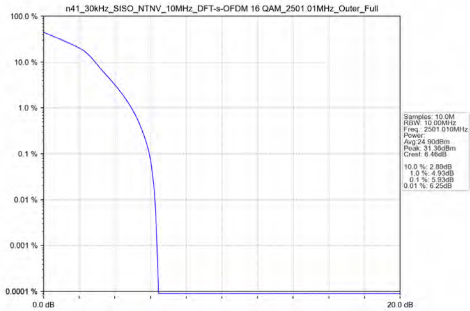
n41_30kHz_SISO_NTNV_10MHz_DFT-s-OFDM_16_QAM_2501.01MHz_Outer_Full_Ant41
