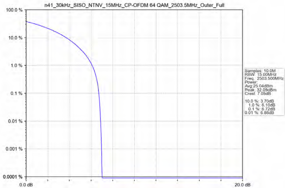
n41_30kHz_SISO_NTNV_15MHz_CP-OFDM 64 QAM 2503.5MHz_Outer_Full_Ant41
