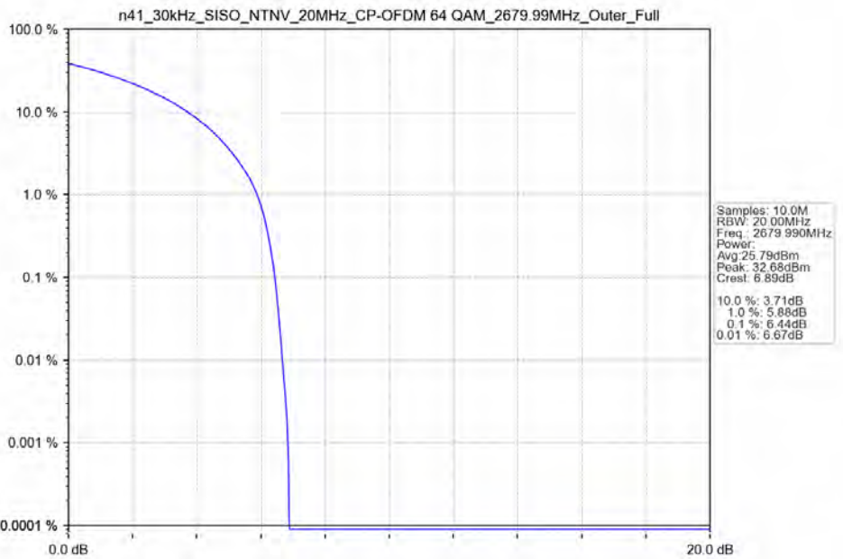
n41_30kHz_SISO_NTNV_20MHz_CP-OFDM 64 QAM 2679.99MHz_Outer_Full_Ant41
