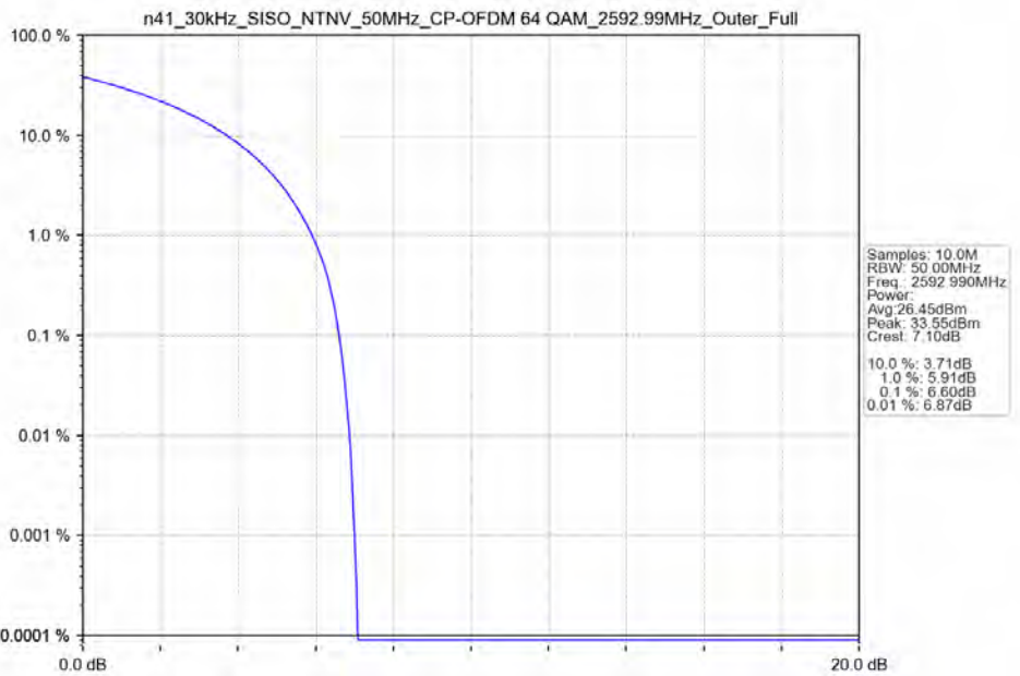
n41_30kHz_SISO_NTNV_50MHz_CP-OFDM_64_QAM_2592.99MHz_Outer_Full_Ant41
