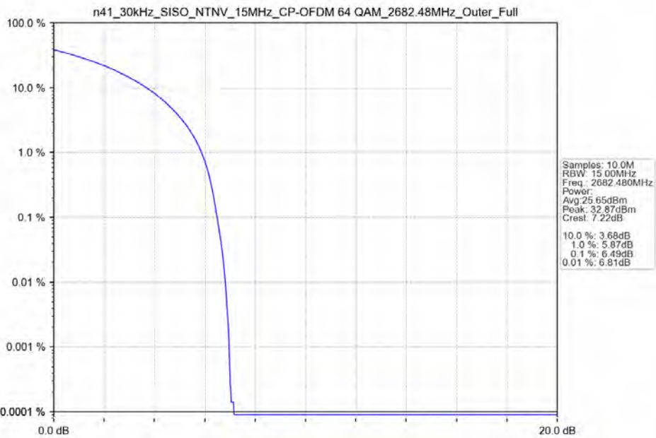
n41_30kHz_SISO_NTNV_15MHz_CP-OFDM_64_QAM_2682.48MHz_Outer_Full_Ant41
