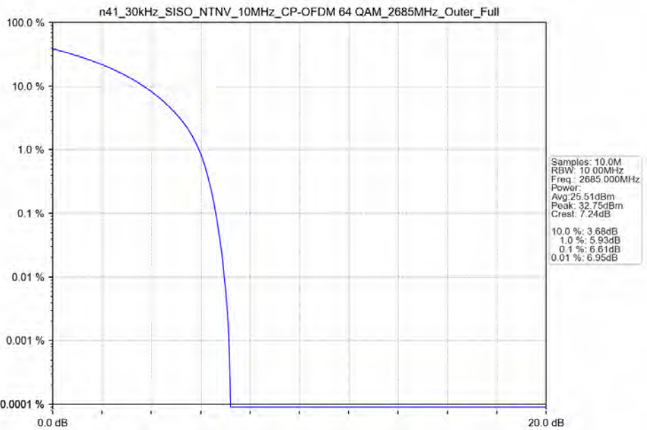
n41_30kHz_SISO_NTNV_10MHz_CP-OFDM 64 QAM_2685MHz_Outer_Full_Ant41
