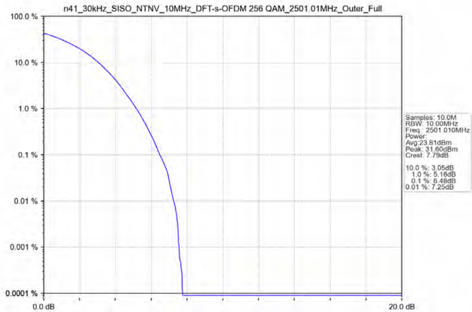
n41_30kHz_SISO_NTNV_10MHz_DFT-s-OFDM_256_QAM_2501.01MHz_Outer_Full_Ant41
