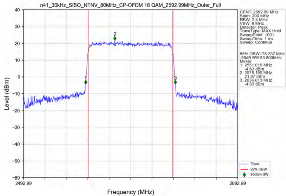
n41_30kHz_SISO_NTNV_80MHz_CP-OFDM_16QAM_2592.99MHz_Outer_Full_Ant41
