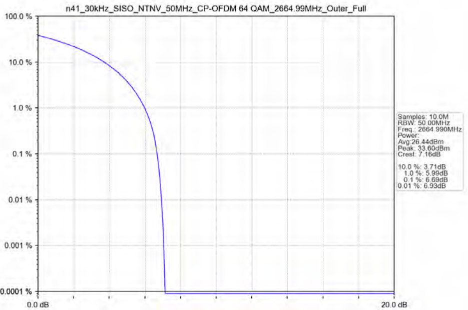
n41_30kHz_SISO_NTNV_50MHz_CP-OFDM_64_QAM_2664.99MHz_Outer_Full_Ant41
