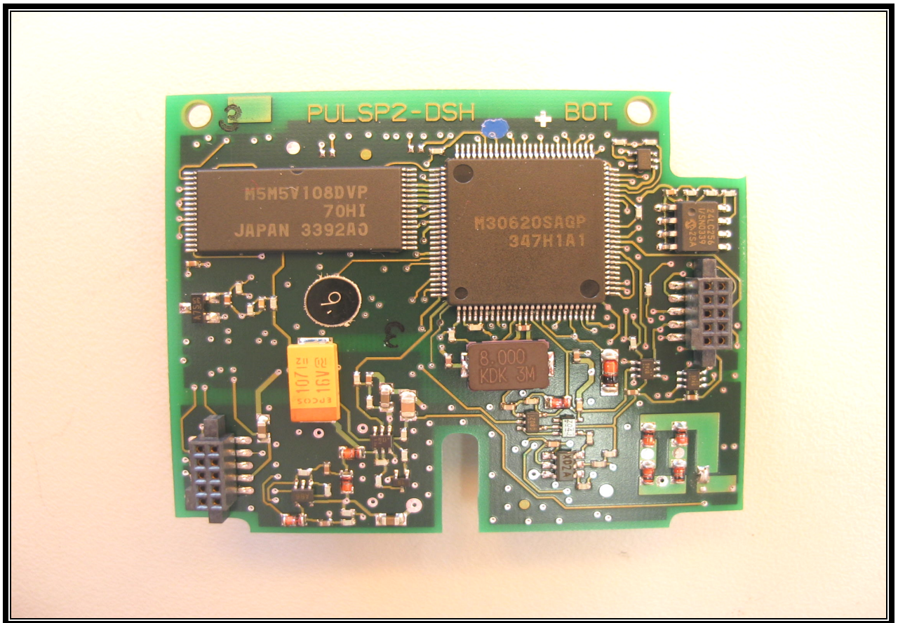
PHOTOGRAPH 33: EUT MODULE PCB2 DIGITAL PART BOTTOM VIEW
