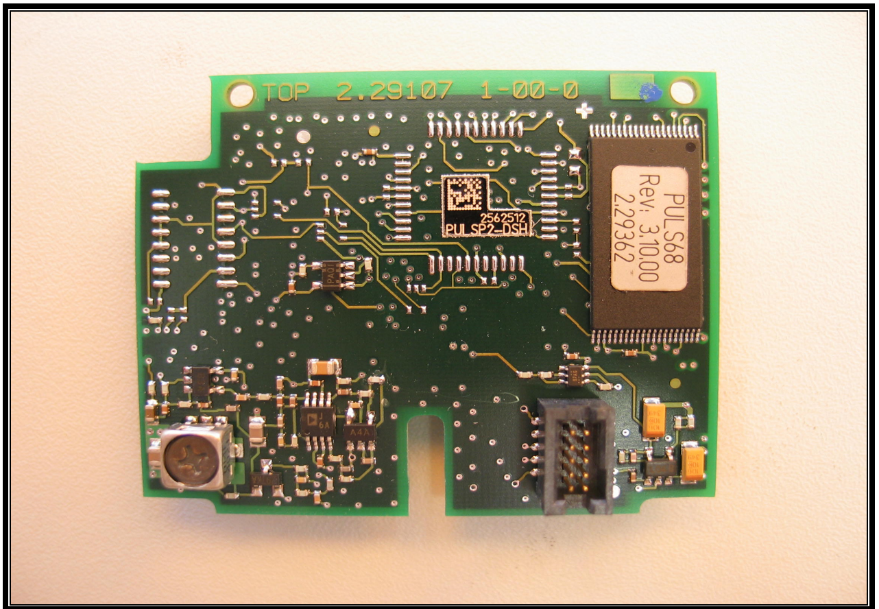
PHOTOGRAPH 32: EUT MODULE PCB2 DIGITAL PART TOP VIEW
