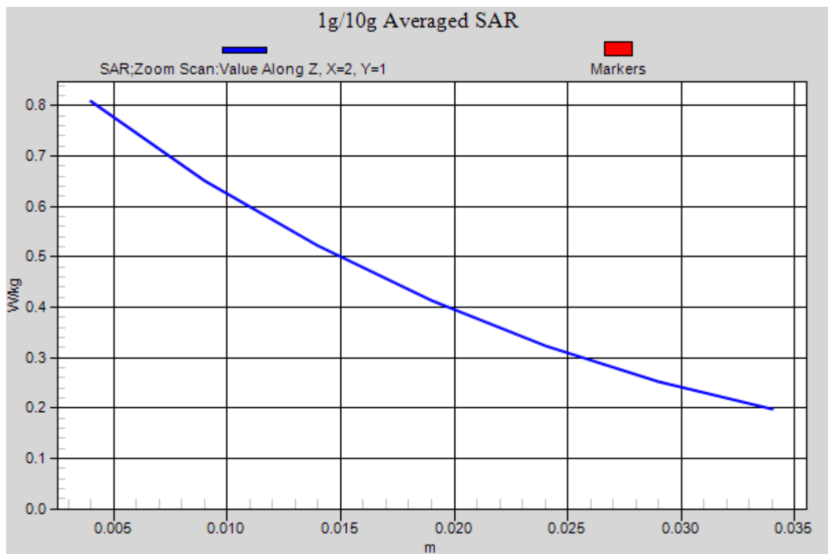
Figure 23 Righ Hand Touch Cheek UMTS Band V Channel 4233
