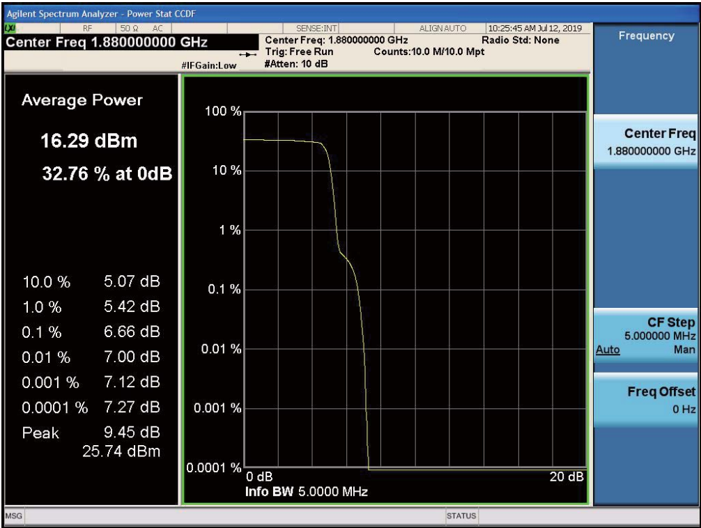
Band2-CH18900-1880MHz-QPSK
