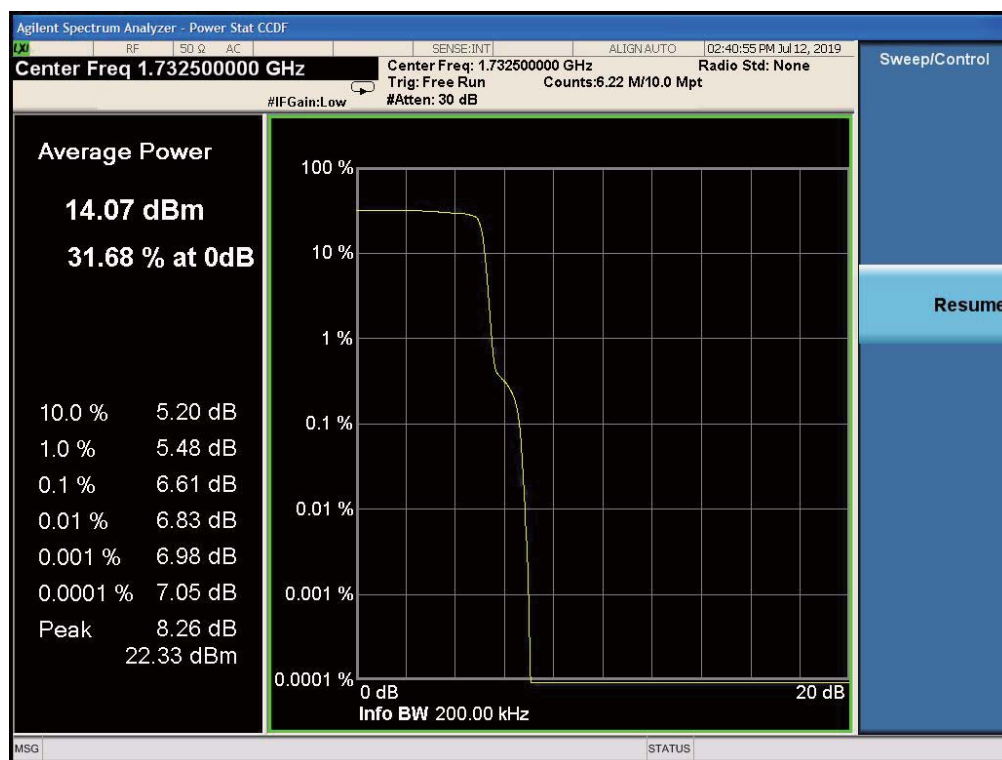
Band4-CH20175-1732.5MHz-QPSK
