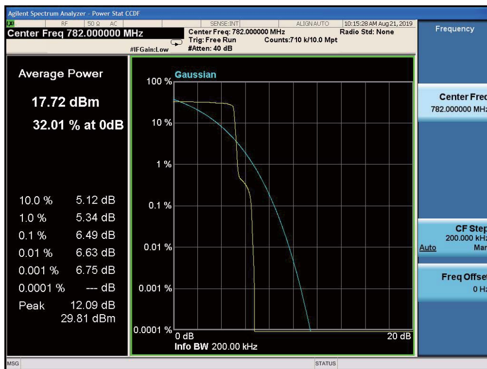
Band13-CH23230-782MHz-QPSK
