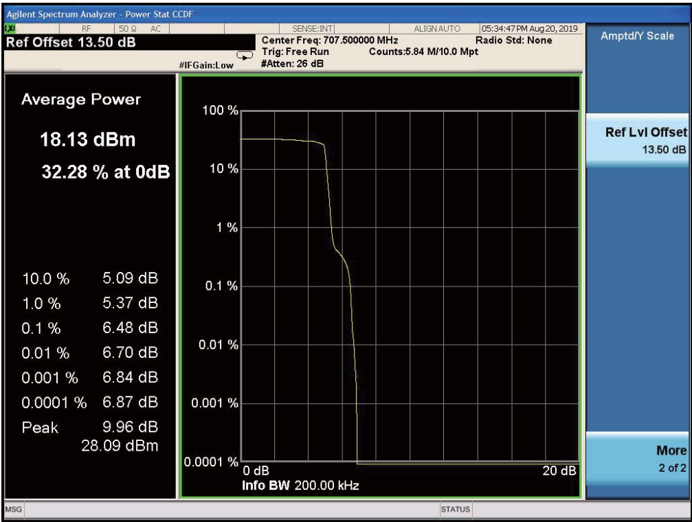
Band12-CH23095-707.5MHz-QPSK
