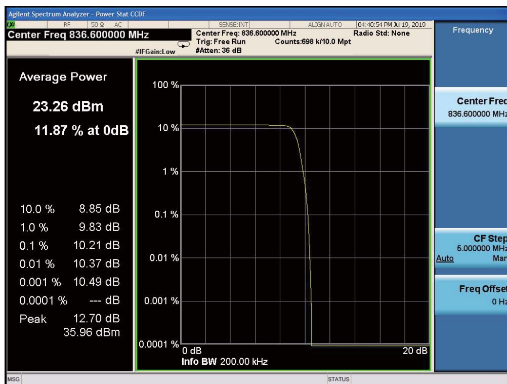
836.6MHz-CH190-GMSK
