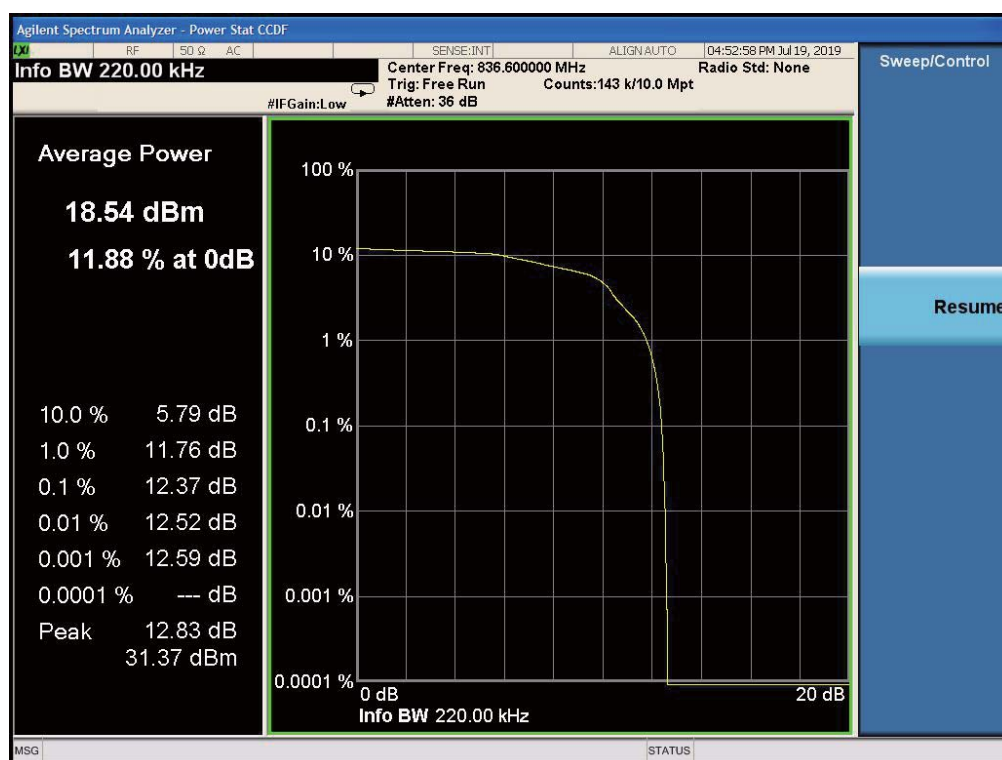
836.6MHz-CH190-8PSK
