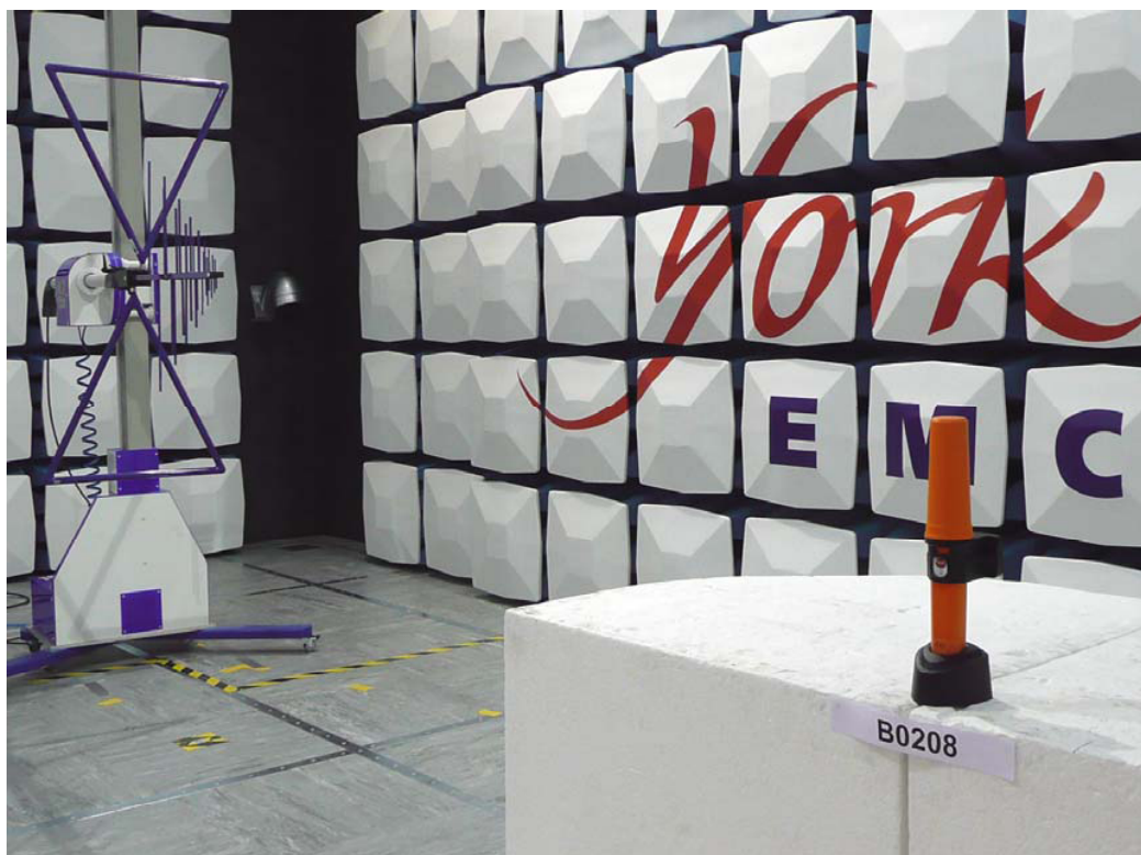
Figure 5.6.2 Radiated Emissions 30MHz to 1000MHz Testing
