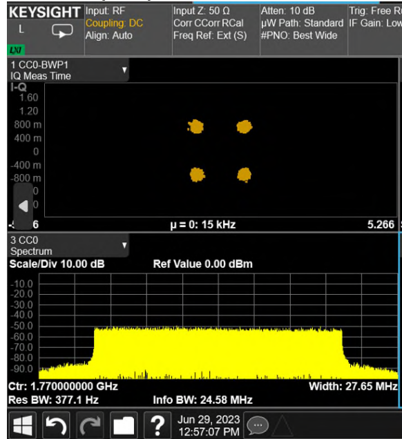
Center Frequency 1770 MHz, QPSK, 20MHz BW
