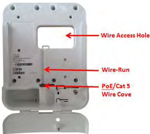
Figure 38: DLC-200C Mounting Plate Wire Runs
