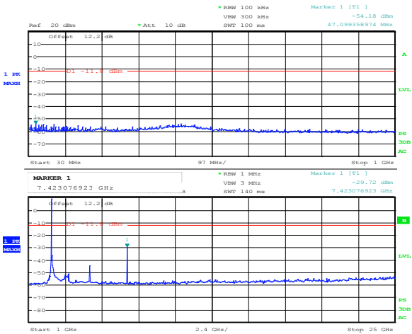
Figure 8.3-5: Conducted spurious emissions, Low channel
