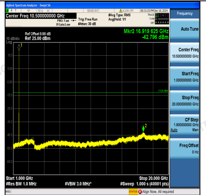
Band4-1312-1000~20000MHz-PASS
