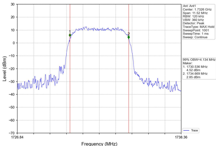
Band4_HSUPA_MCH_1732.6MHz_Subtest 1_NTNV
