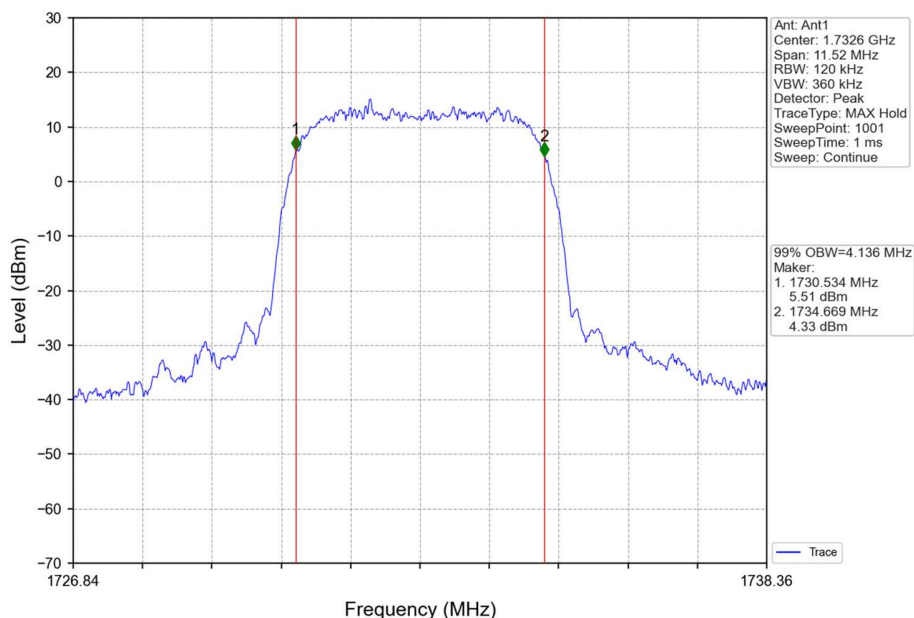
Band4_RMC_MCH_1732.6MHz_12.2kbps RMC_NTNV
