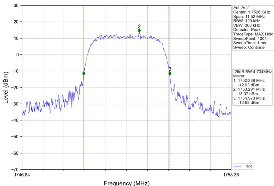
Band4_HSUPA_HCH_1752.6MHz_Subtest 1_NTNV
