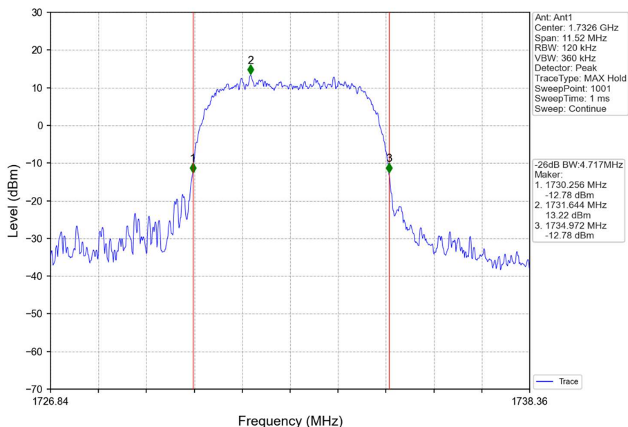
Band4_HSDPA_MCH_1732.6MHz_Subtest 1_NTNV
