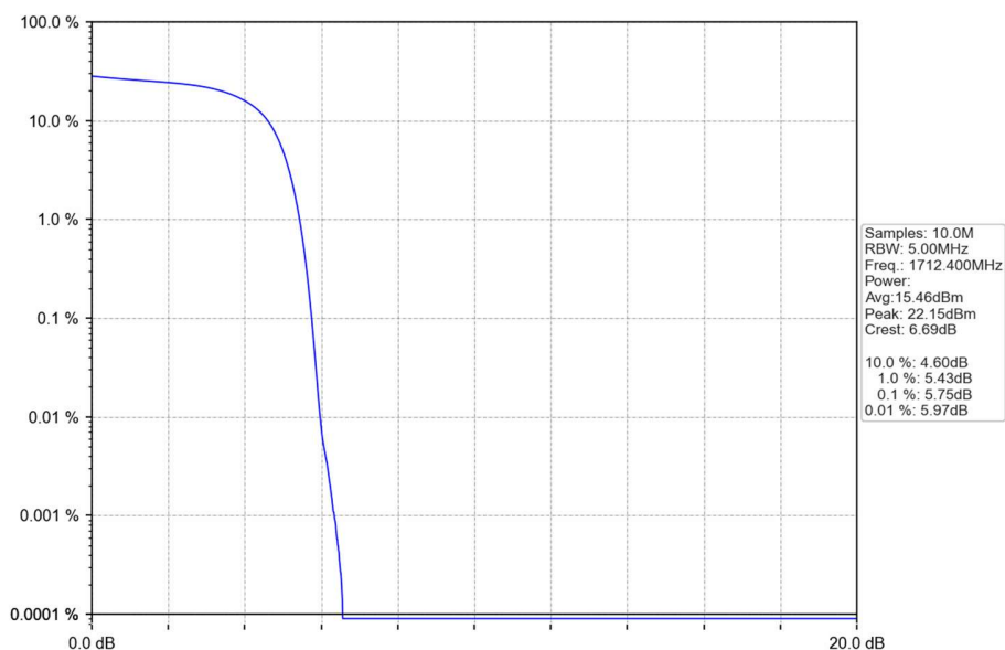
Band4_HSDPA_LCH_1712.4MHz_Subtest 1_NTNV
