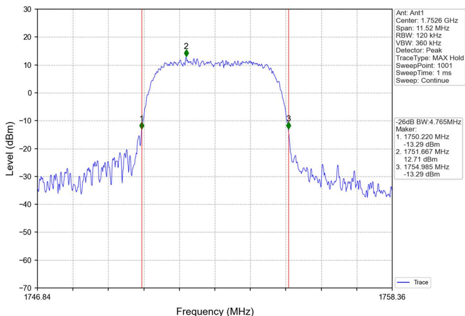
Band4_HSDPA_HCH_1752.6MHz_Subtest 1_NTNV
