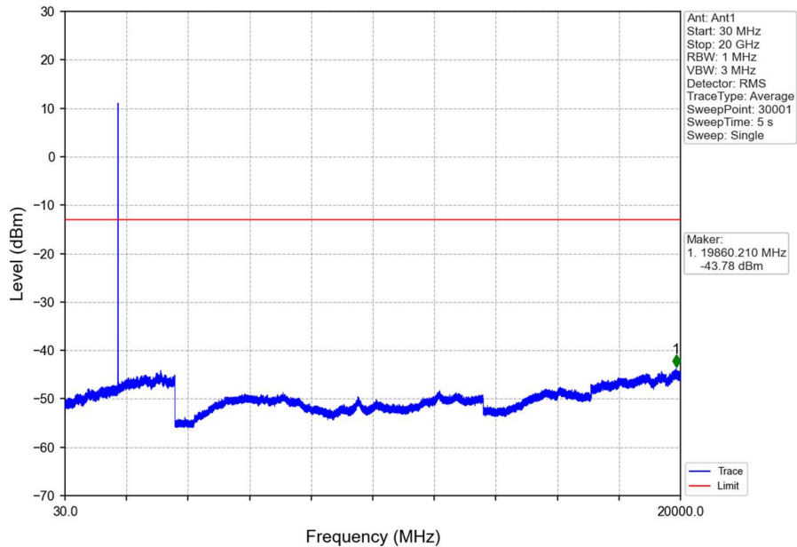
Band4_HSDPA_HCH_1752.6MHz_Subtest 1_NTNV
