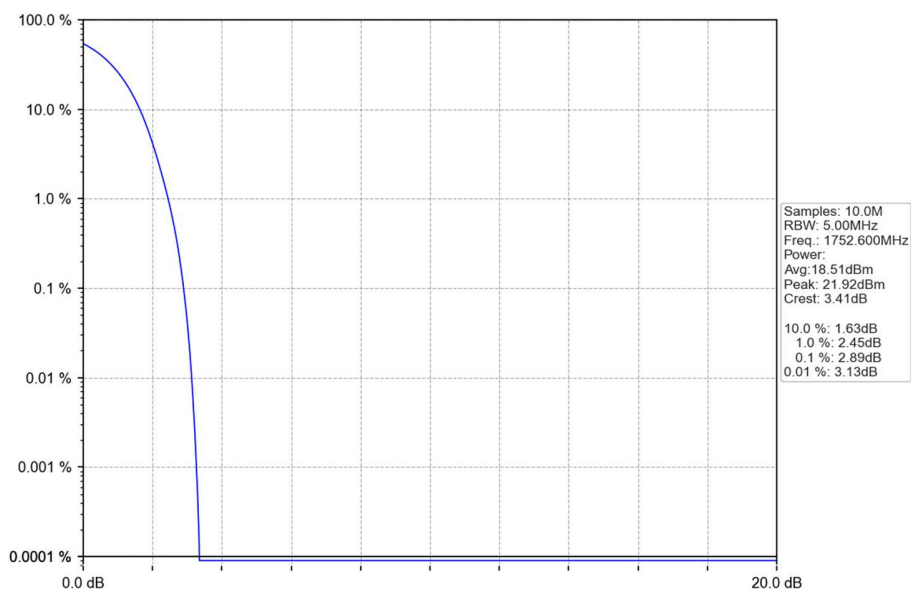
Band4_RMC_HCH_1752.6MHz_12.2kbps RMC_NTNV
