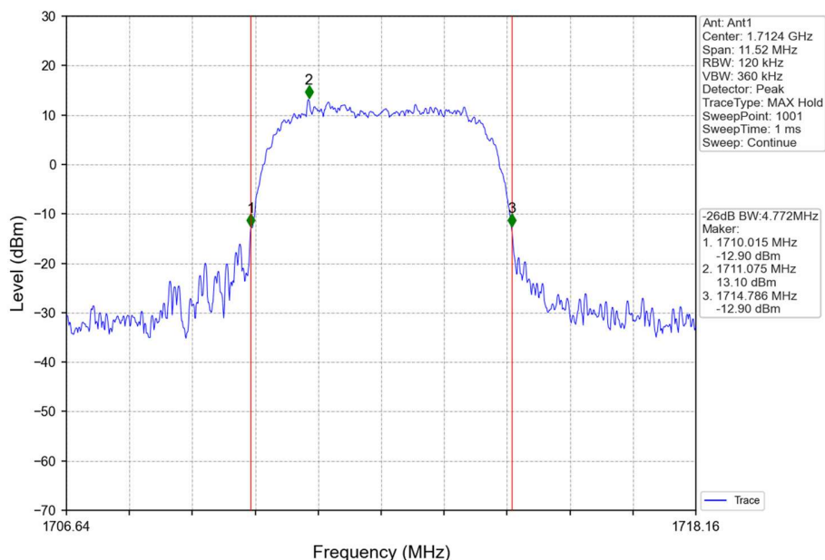
Band4_HSDPA_LCH_1712.4MHz_Subtest 1_NTNV
