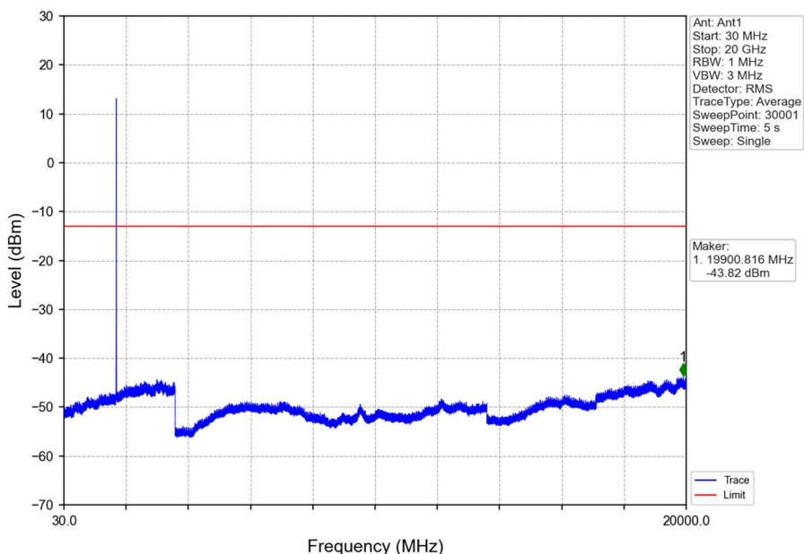
Band4_RMC_LCH_1712.4MHz_12.2kbps RMC_NTNV
