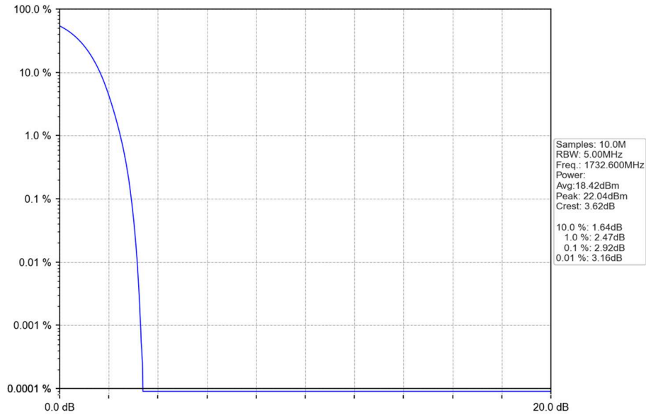
Band4_RMC_MCH_1732.6MHz_12.2kbps RMC_NTNV
