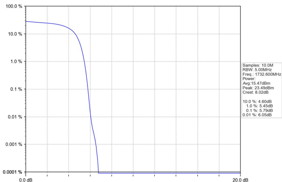
Band4_HSUPA_MCH_1732.6MHz_Subtest 1_NTNV
