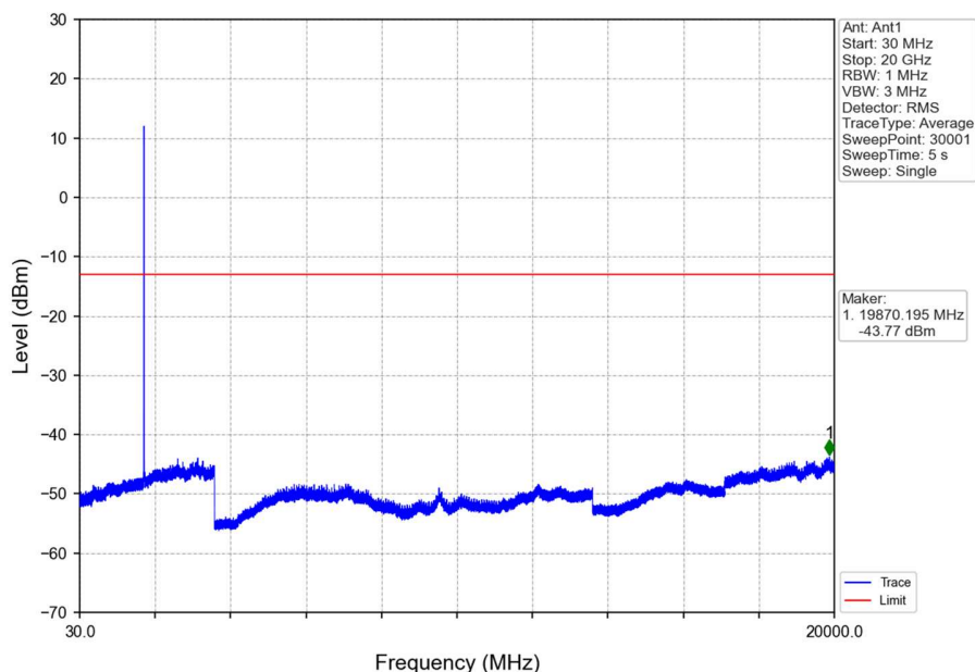
Band4_HSDPA_MCH_1732.6MHz_Subtest 1_NTNV
