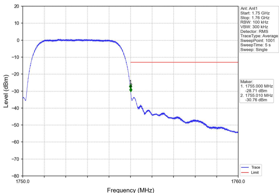
Band4_HSDPA_HCH_1752.6MHz_Subtest 1_NTNV
