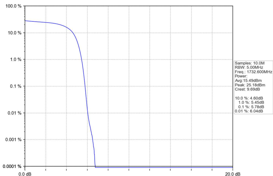
Band4_HSDPA_MCH_1732.6MHz_Subtest 1_NTNV
