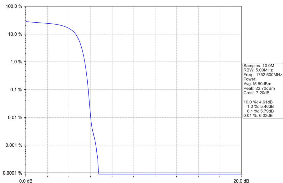
Band4_HSDPA_HCH_1752.6MHz_Subtest 1_NTNV
