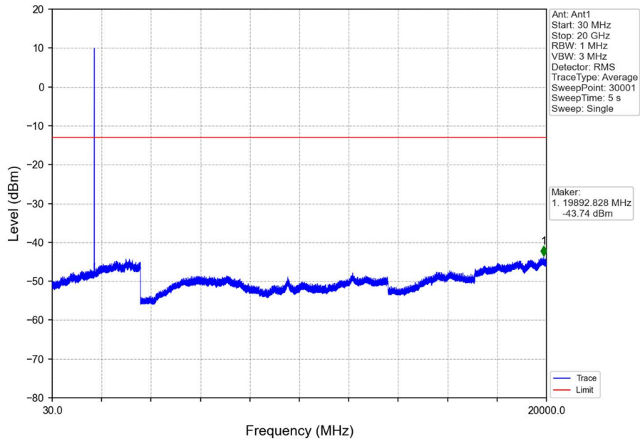
Band4_HSUPA_MCH_1732.6MHz_Subtest 1_NTNV
