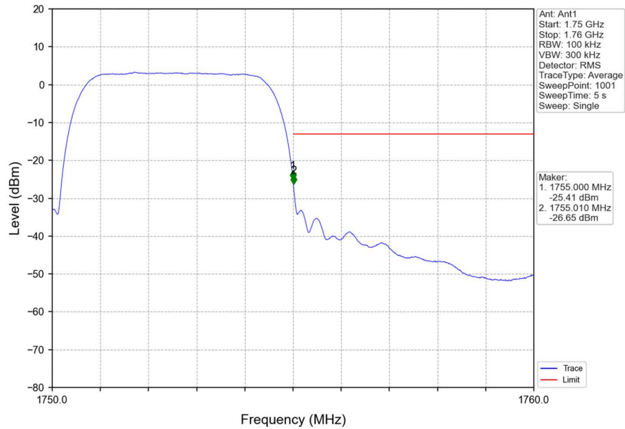
Band4_RMC_HCH_1752.6MHz_12.2kbps RMC_NTNV
