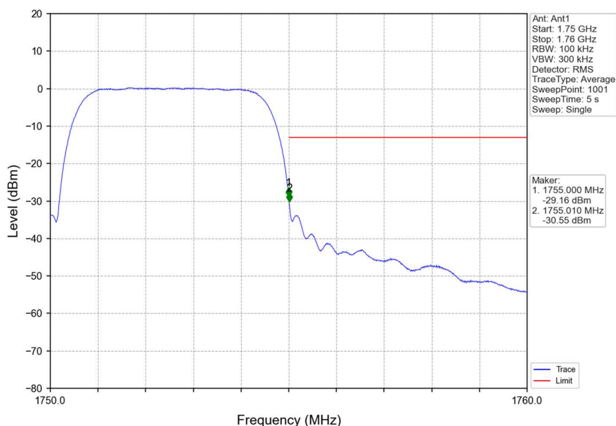
Band4_HSUPA_HCH_1752.6MHz_Subtest 1_NTNV
