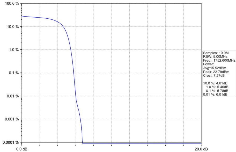
Band4_HSUPA_HCH_1752.6MHz_Subtest 1_NTNV
