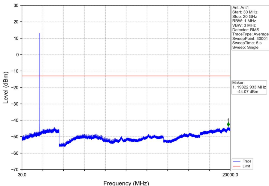
Band4_RMC_MCH_1732.6MHz_12.2kbps RMC_NTNV
