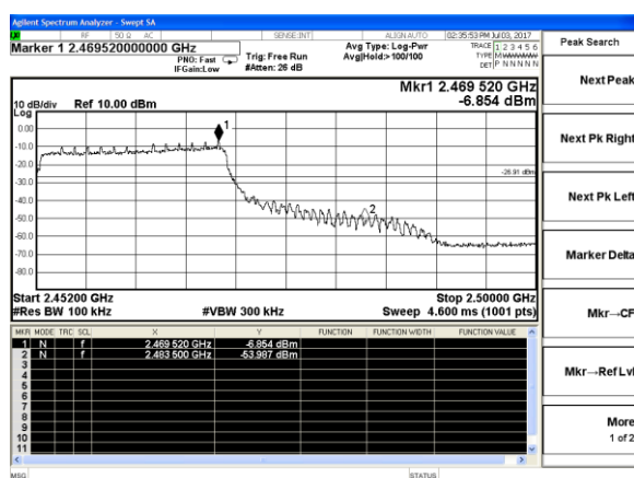
802.11n(HT40)-High channel
