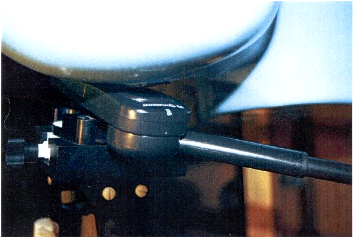
Photo 9 – SAR set-up: Bottom view, right side of head, incorrect antenna position
