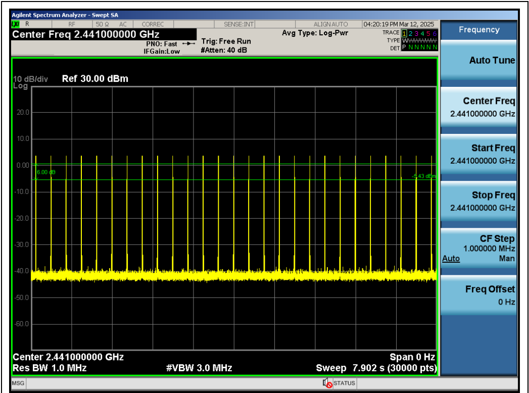
Test_Graph_BR_HOP_ANT1_NA_1Mbps_2441_Number of Busr
