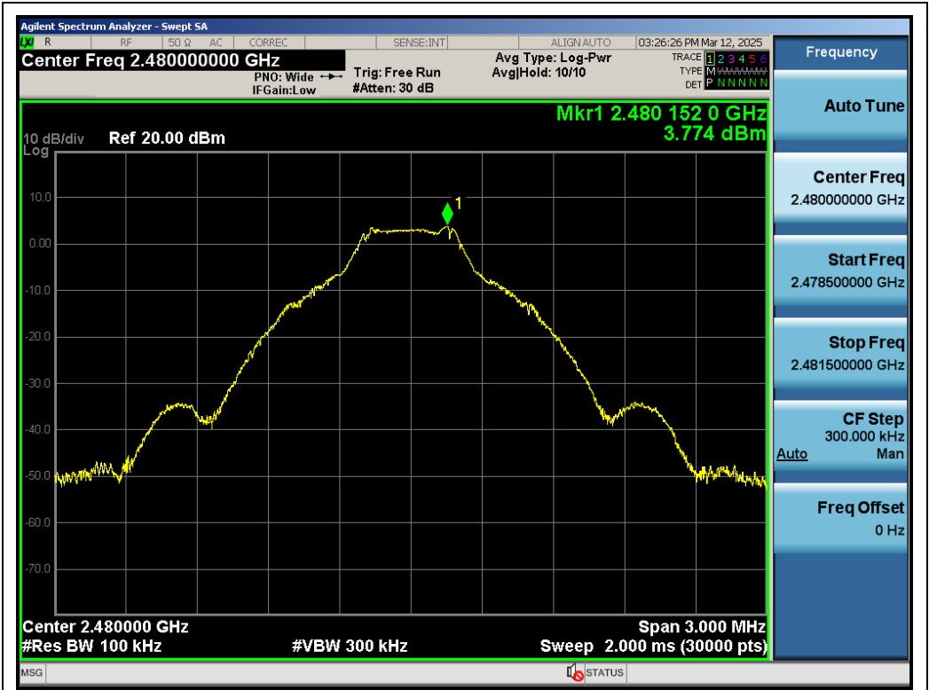
Test_Graph_BR_ANT1_2480_1Mbps_Reference Level
