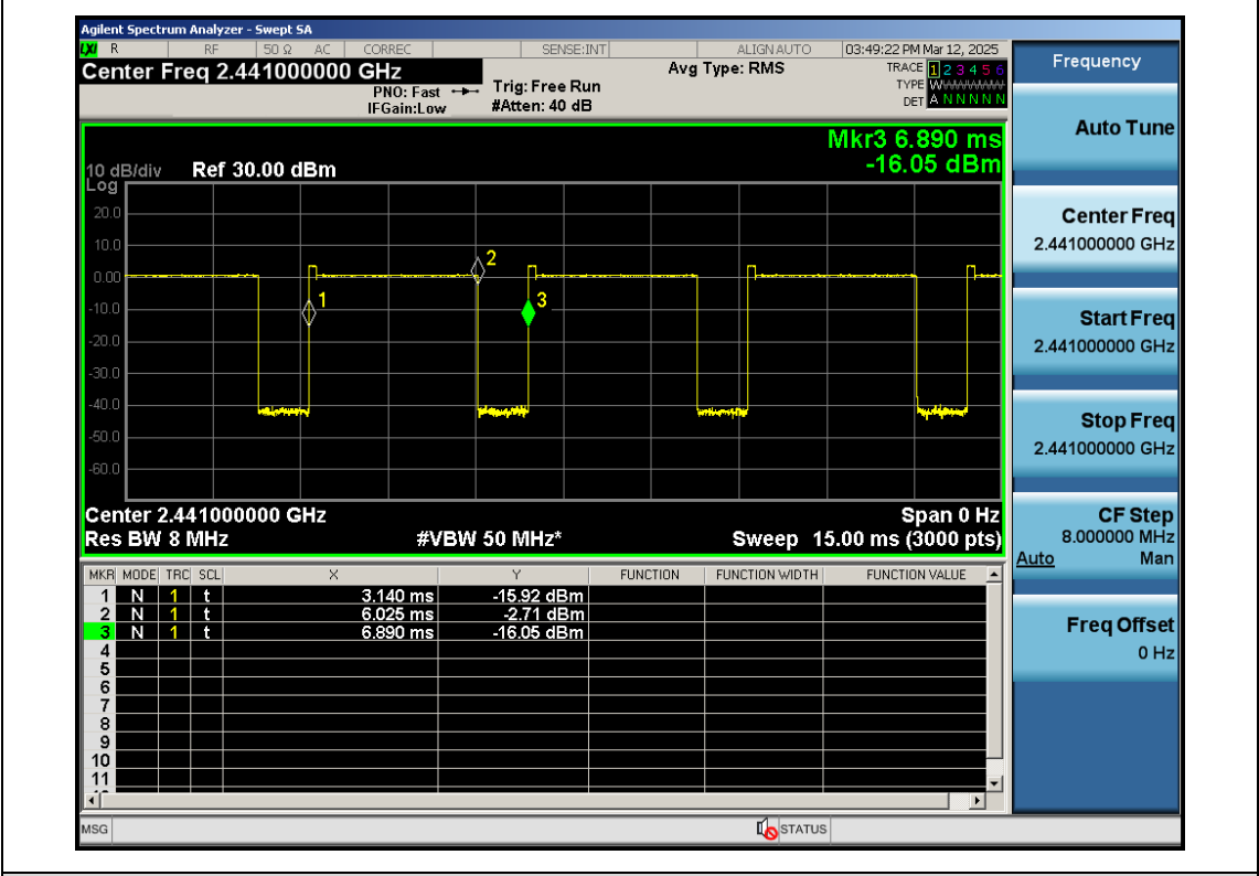
EDR-8DPSK-ANT1-2441
