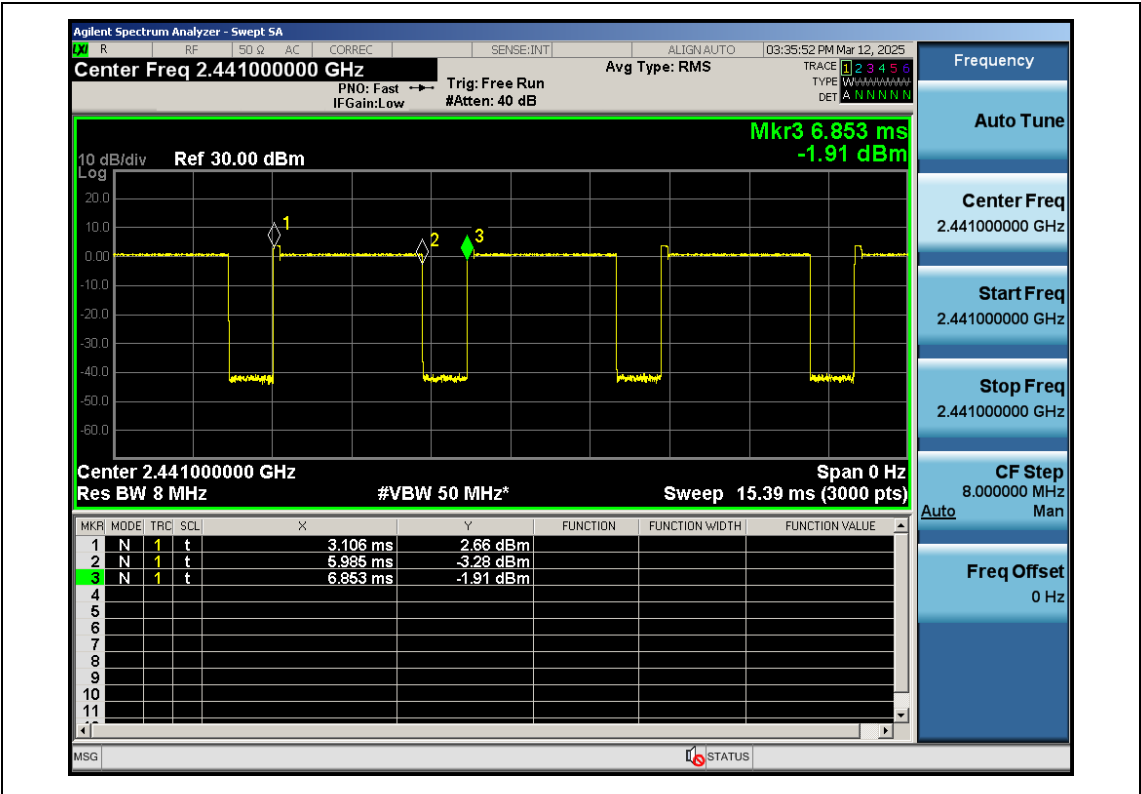
EDR- \pi /4-DQPSK-ANT1-2441
