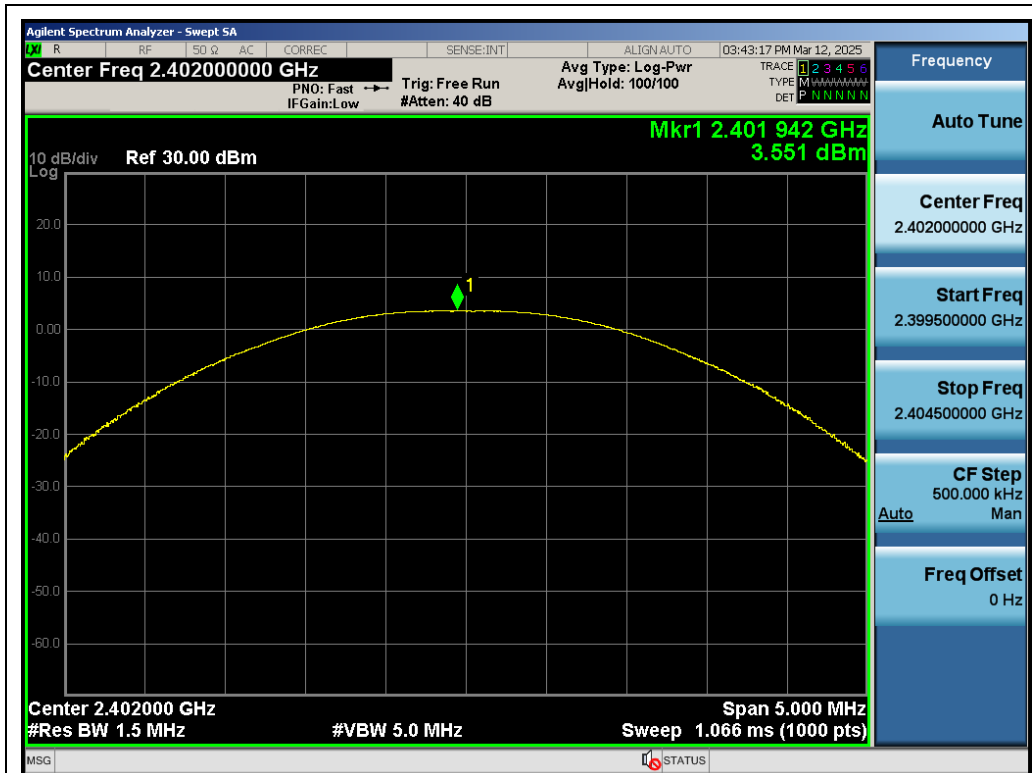
Test_Graph_EDR_ANT1_2402_3Mbps_Peak Power
