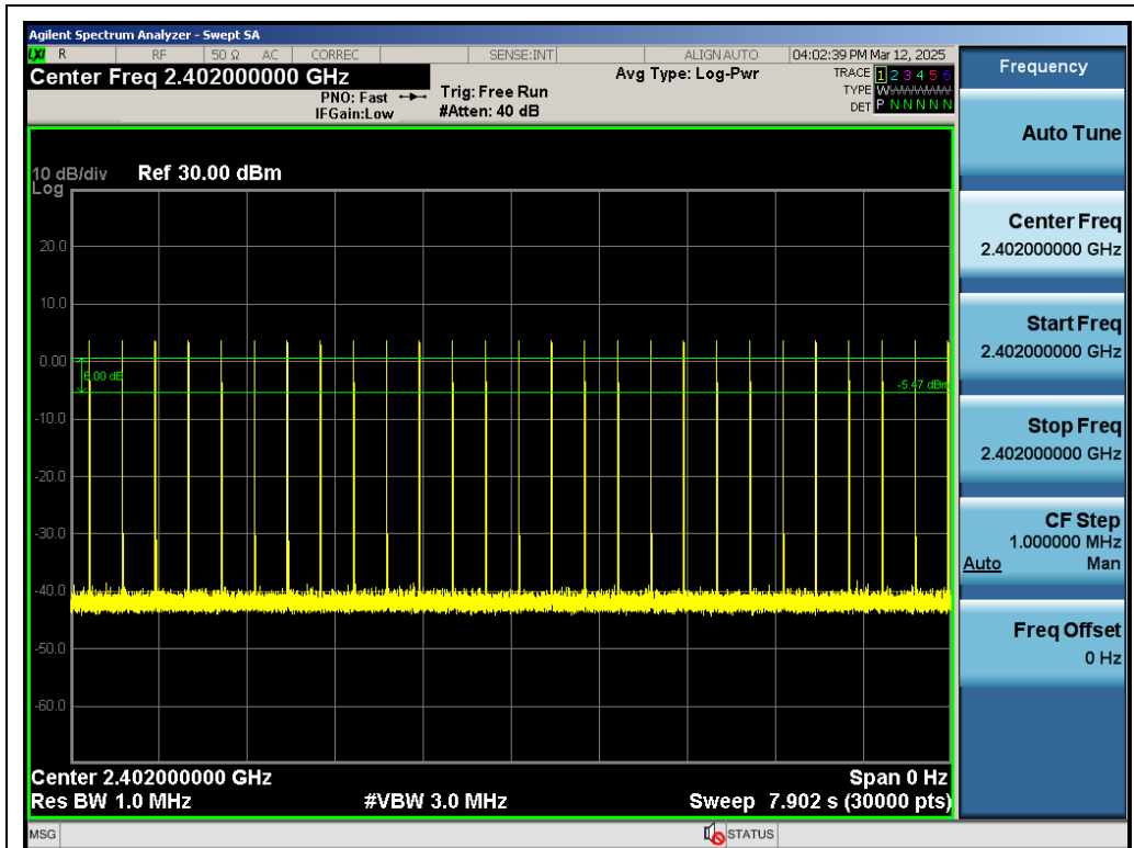
Test_Graph_EDR_HOP_ANT1_NA_3Mbps_2402_Number of Burst
