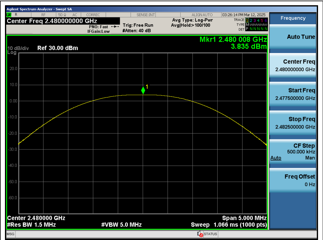
Test_Graph_BR_ANT1_2480_1Mbps_Peak Power
