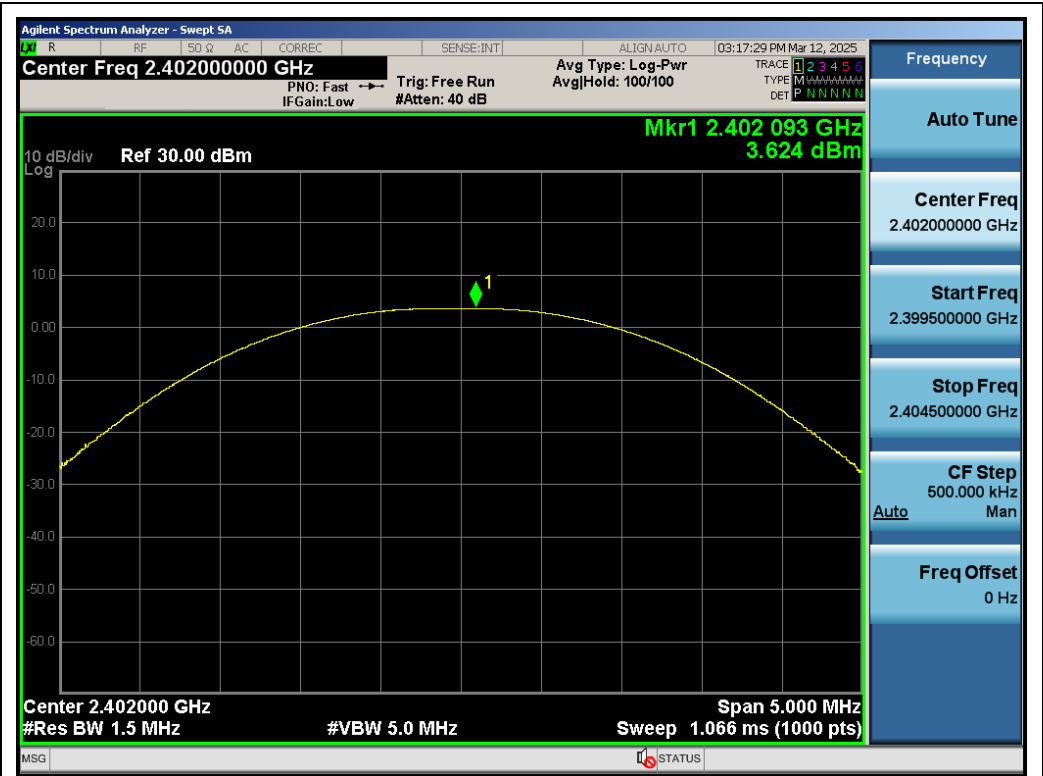
Test_Graph_BR_ANT1_2402_1Mbps_Peak Power
