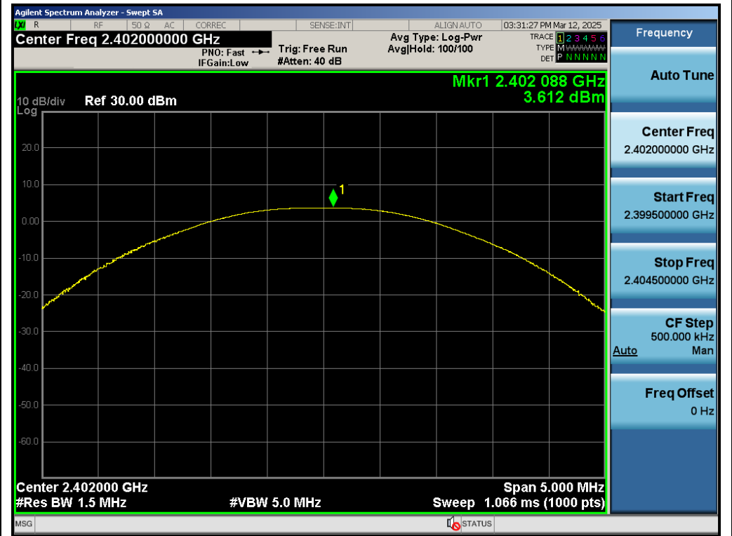
Test_Graph_EDR_ANT1_2402_2Mbps_Peak Power
