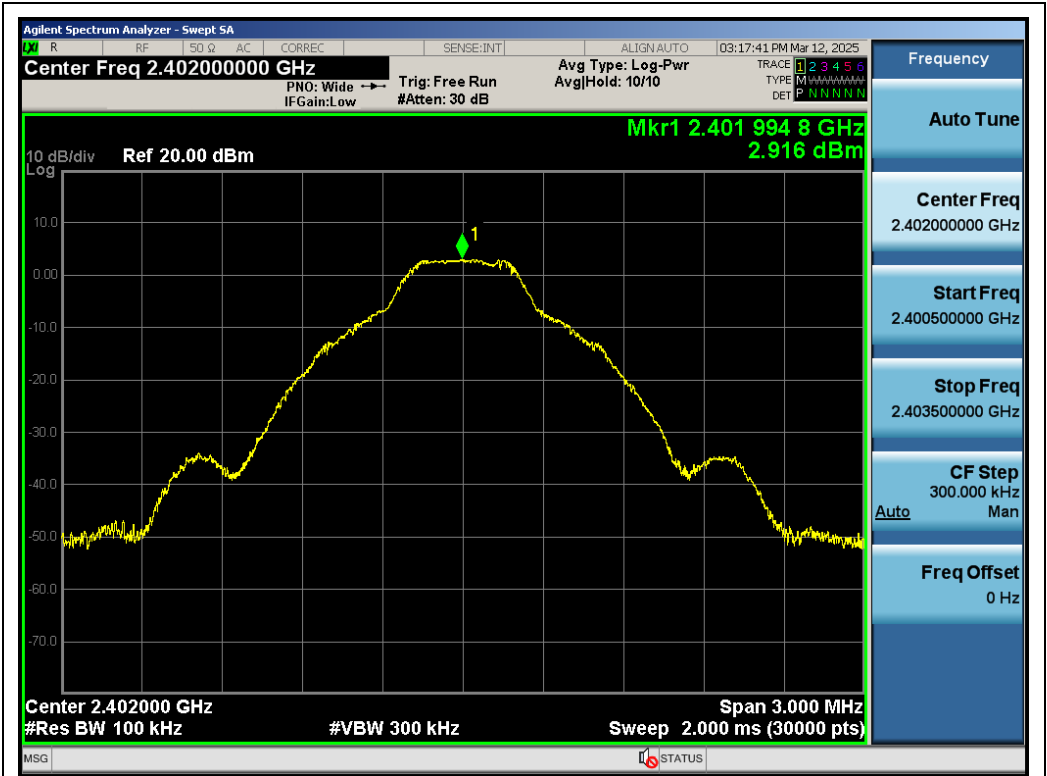
Test_Graph_BR_ANT1_2402_1Mbps_Reference Level
