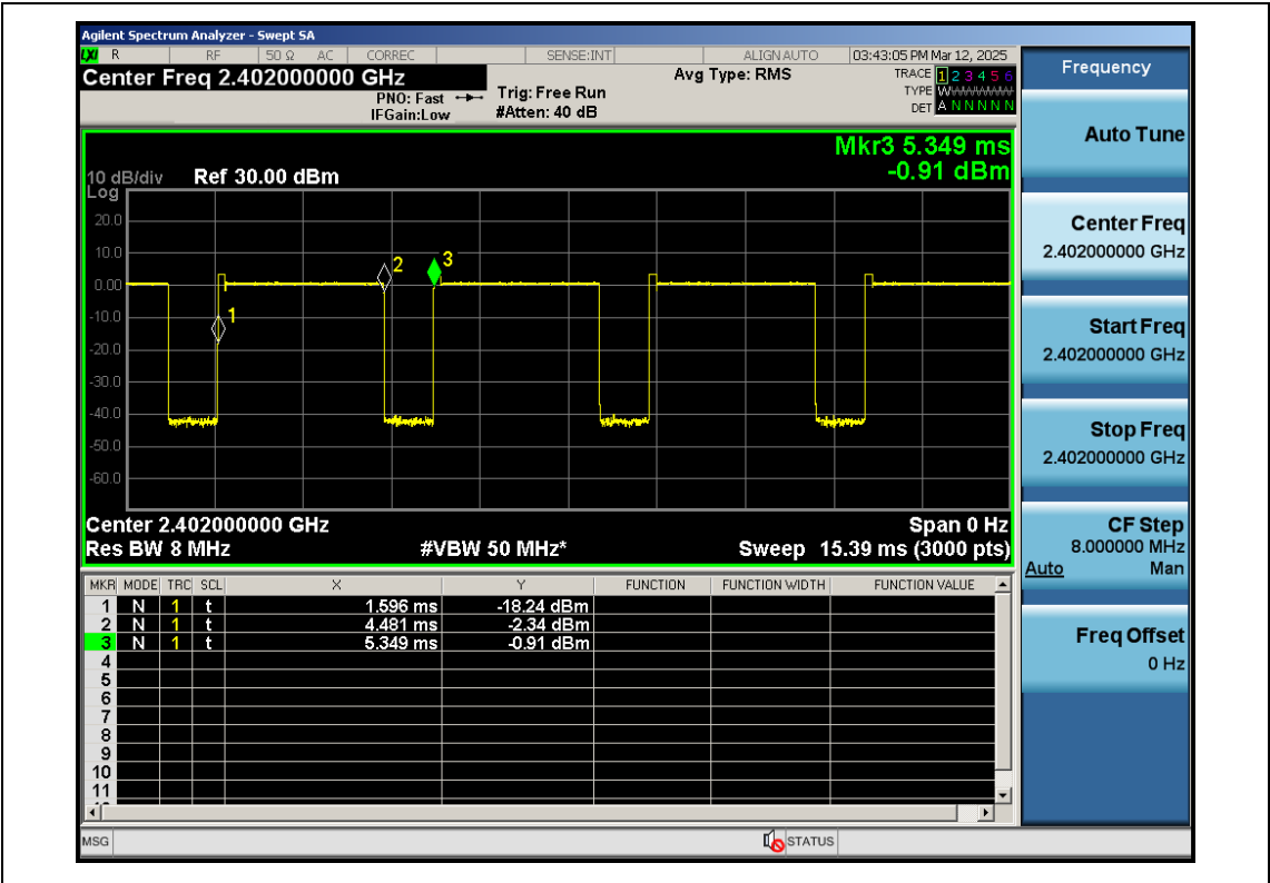
EDR--8DPSK-ANT1-2402
