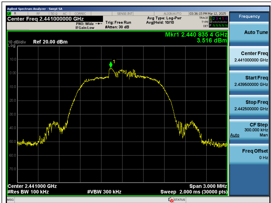
Test_Graph_EDR_ANT1_2441_2Mbps_Reference Level
