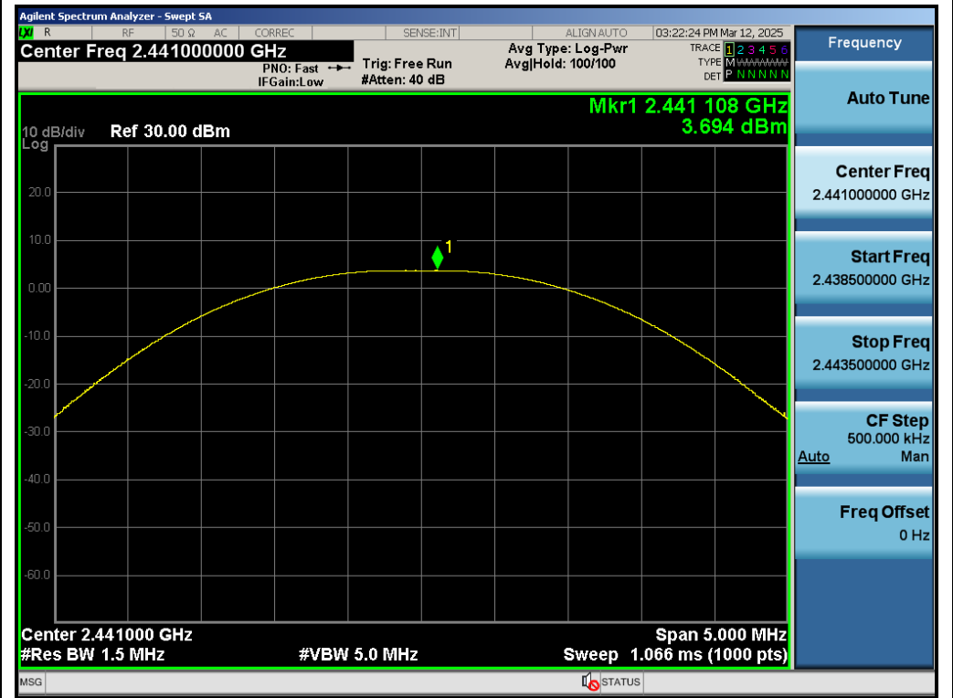
Test_Graph_BR_ANT1_2441_1Mbps_Peak Power
