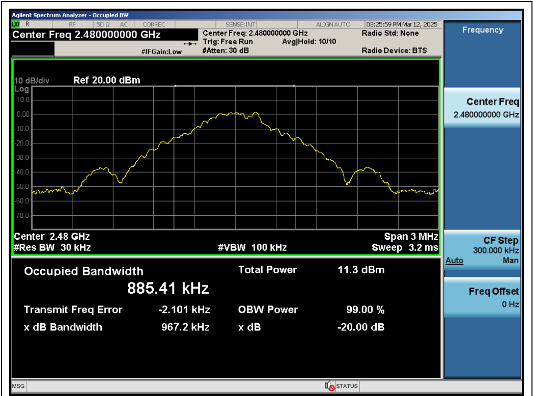
Test_Graph_BR_ANT1_2480_1Mbps_OBW
