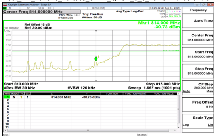
Cat M1_Band26_Part90s_3MHz_QPSK_6_0_LowCH26705-815.5
