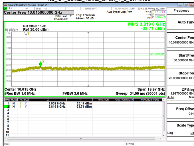
NB_IoT_Band2_15kHz_QPSK_1_0_CH19199
