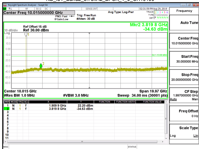
NB_IoT_Band2_3.75kHz_BPSK_1_0_CH19199
