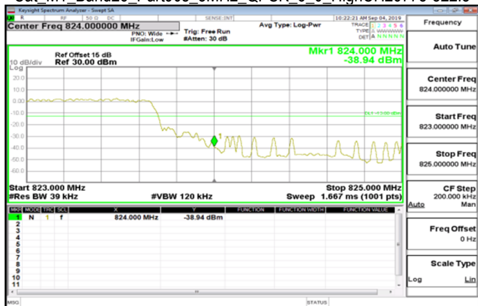
Cat M1_Band26_Part90s_3MHz_QPSK_6_0_HighCH26775-822.5
