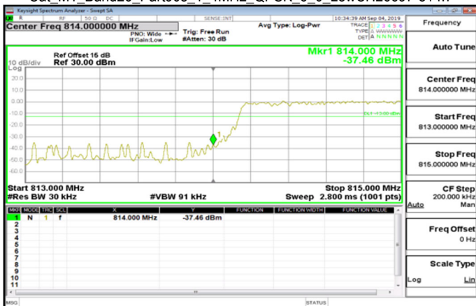
Cat_M1_Band26_Part90s_1_4MHz_QPSK_6_0_LowCH26697-814.7
