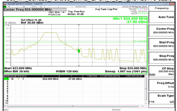
Cat_M1_Band26_Part90s_3MHz_QPSK_1_5_HighCH26775-822.5
