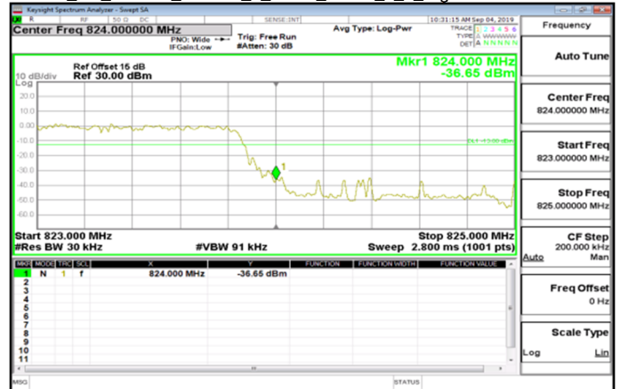
Cat_M1_Band26_Part90s_1_4MHz_QPSK_6_0_HighCH26783-823.3
