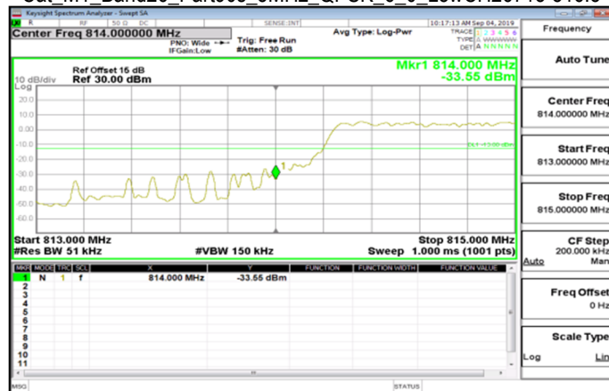
Cat M1_Band26_Part90s_5MHz_QPSK_6_0_LowCH26715-816.5
