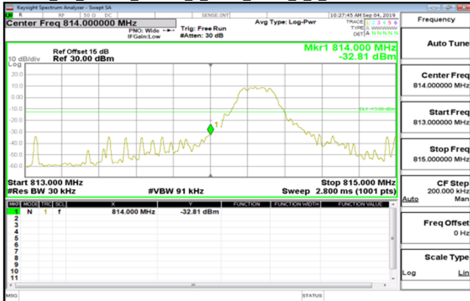
Cat_M1_Band26_Part90s_1_4MHz_QPSK_1_0_LowCH26697-814.7
