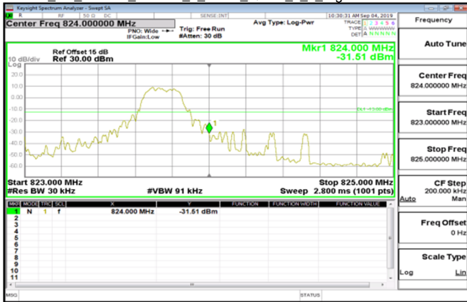
Cat_M1_Band26_Part90s_1_4MHz_QPSK_1_5_HighCH26783-823.3
