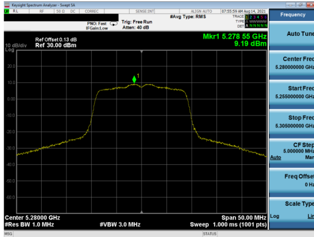
Plot 7-403. PSD Antenna 1b (20MHz BW 802.11n – Ch. 56, MCS2)
