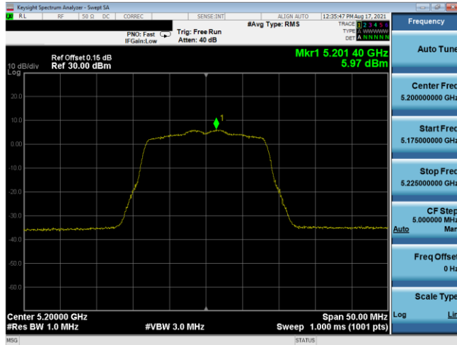
Plot 7-379. ISCED PSD Antenna 3b (20MHz BW 11n – Ch.40, MCS2)
