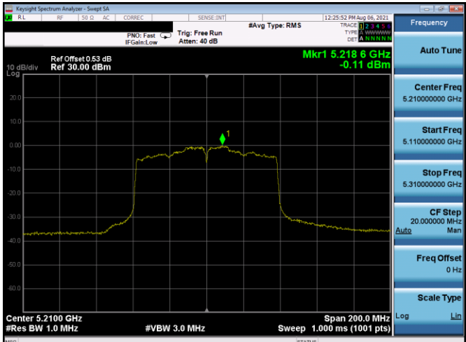
Plot 7-383. ISCED PSD Antenna 3b (80MHz BW 11ac – Ch.42, MCS2)
