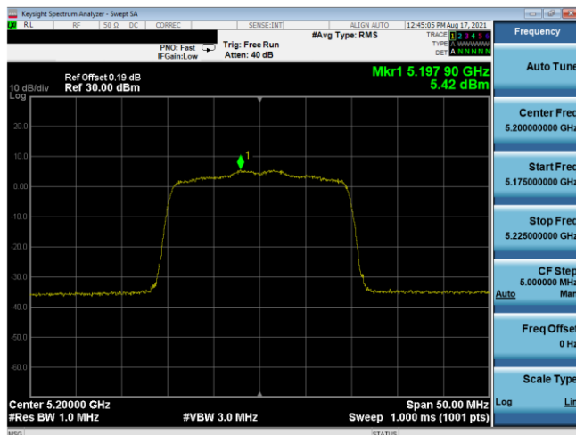
Plot 7-380. ISCED PSD Antenna 3b (20MHz BW 11ax(SU) – Ch.40, MCS2)
