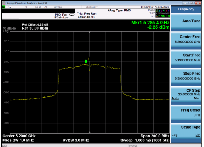
Plot 7-407. PSD Antenna 1b (80MHz BW 802.11ac – Ch. 58, MCS2)
