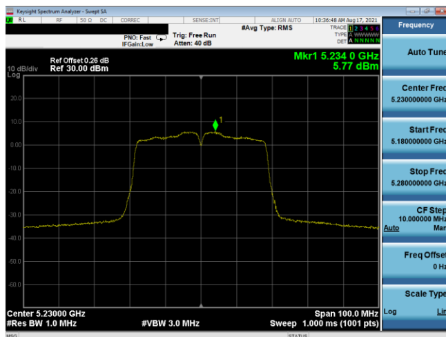
Plot 7-381. ISCED PSD Antenna 3b (40MHz BW 11n – Ch.46, MCS2)
