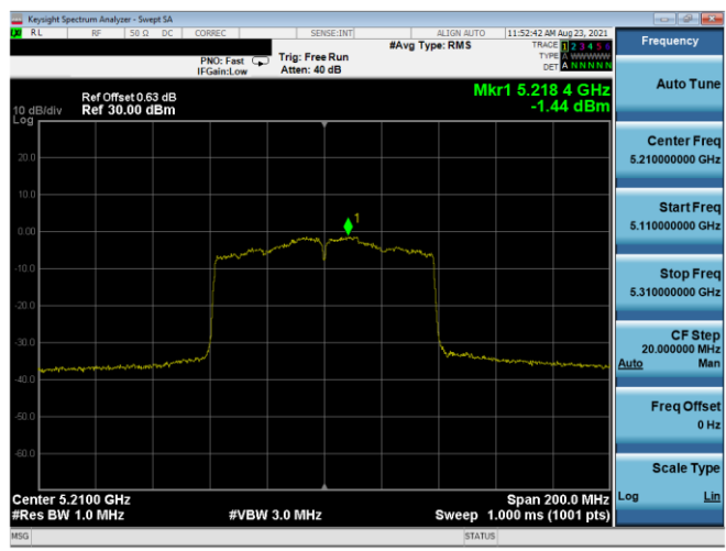
Plot 7-389. ISED PSD Antenna 3b (80MHz BW 11ac – Ch.42, MCS3)
