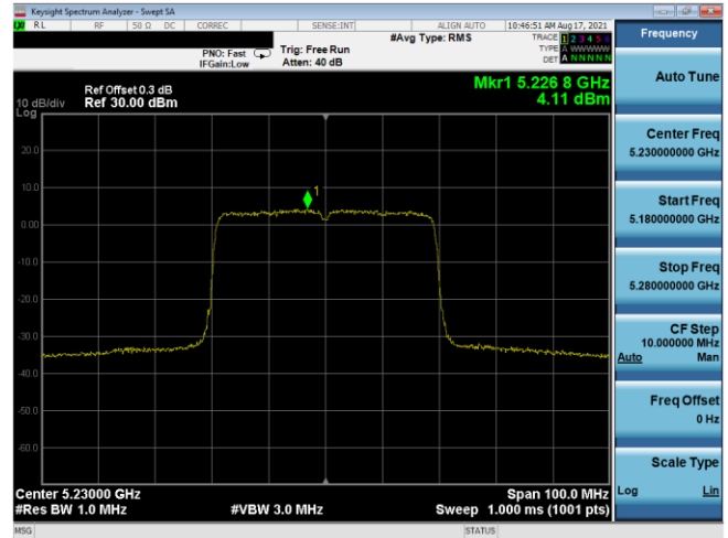
Plot 7-382. ISCED PSD Antenna 3b (40MHz BW 11ax(SU) – Ch.46, MCS2)
