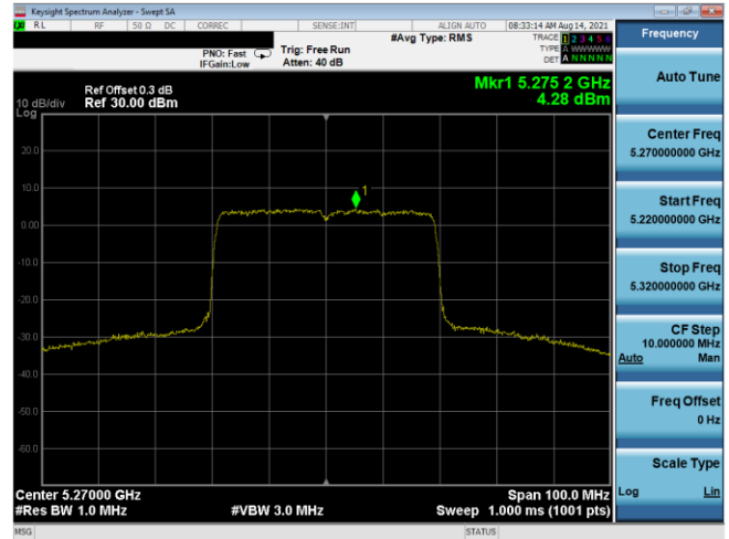
Plot 7-406. PSD Antenna 1b (40MHz BW 802.11ax(SU) – Ch. 54, MCS2)
