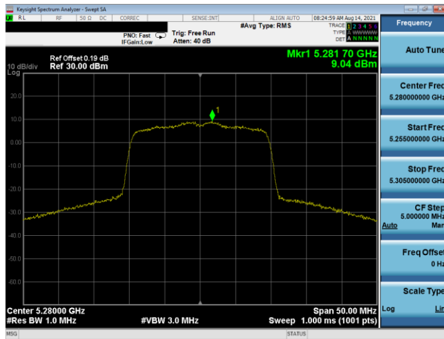
Plot 7-404. PSD Antenna 1b (20MHz BW 802.11ax(SU) – Ch. 56, MCS2)
