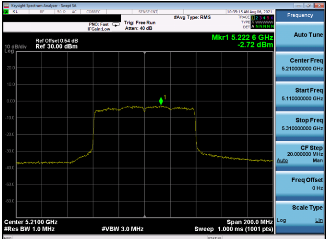
Plot 7-384. ISCED PSD Antenna 3b (80MHz BW 11ax (SU) – Ch.42, MCS2)
