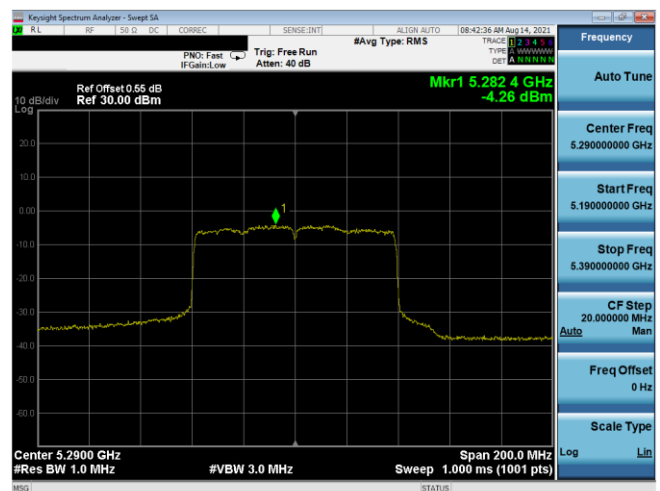
Plot 7-408. PSD Antenna 1b (80MHz BW 802.11ax(SU) – Ch. 58, MCS2)
