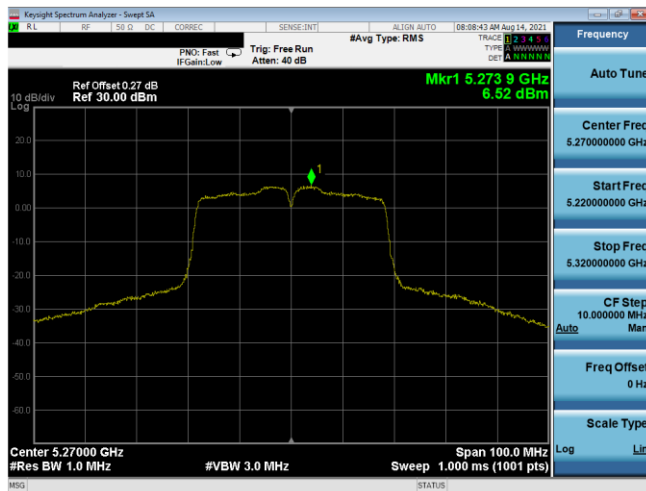
Plot 7-405. PSD Antenna 1b (40MHz BW 802.11n – Ch. 54, MCS2)
