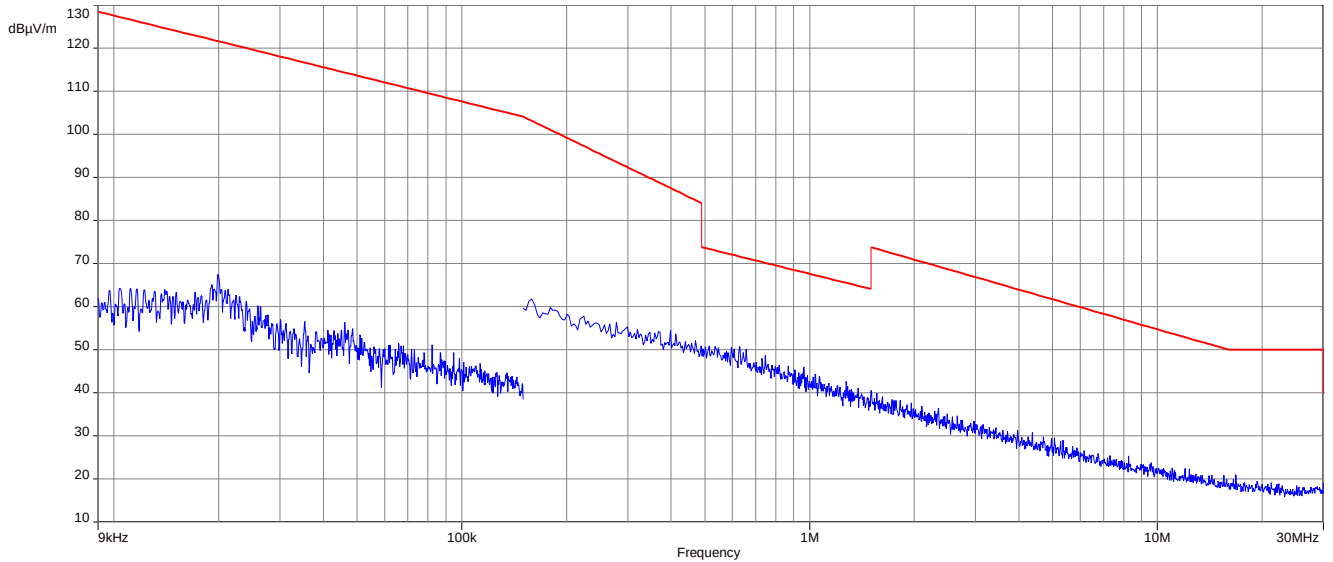
Plot 1: 9 kHz to 30 MHz, 2402 MHz, transmit mode, valid for 1 Msps and 2 Msps
