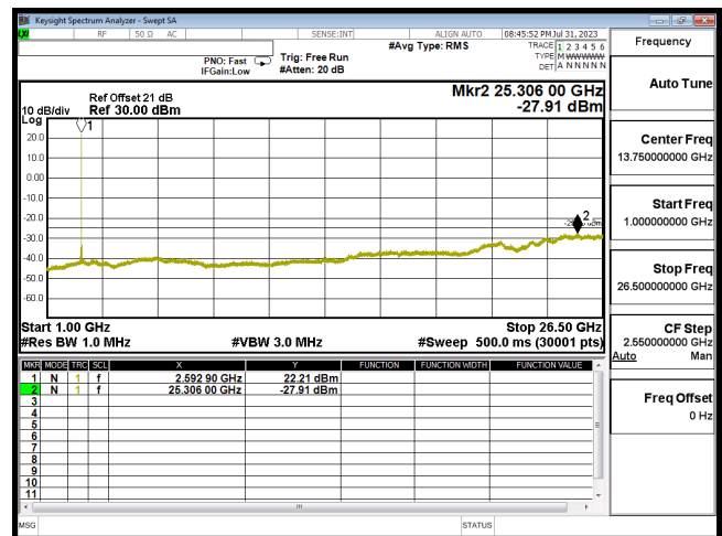
CSE B41 20M CH40620 QPSK(1,50) 1G-26.5G
