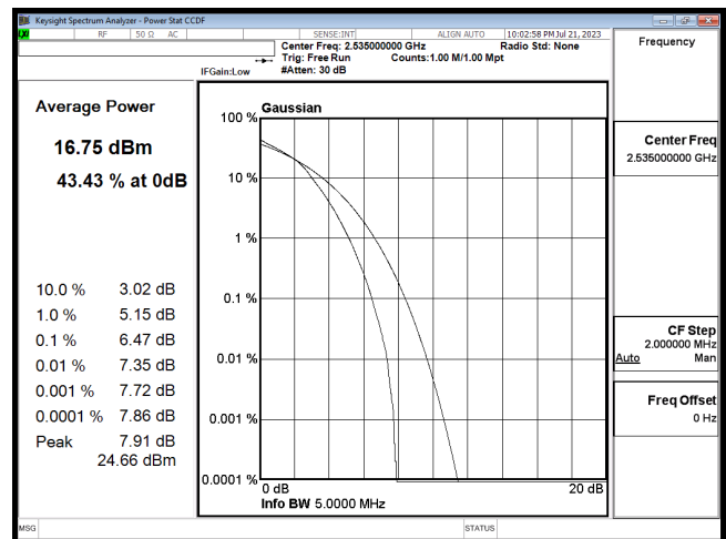
PTAR B7 5M CH21100 16QAM
