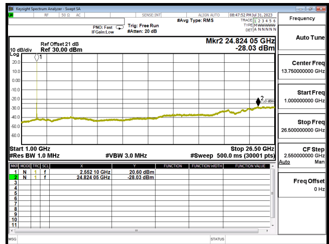
CSE B41 15M CH40215 QPSK(1,37) 1G-26.5G
