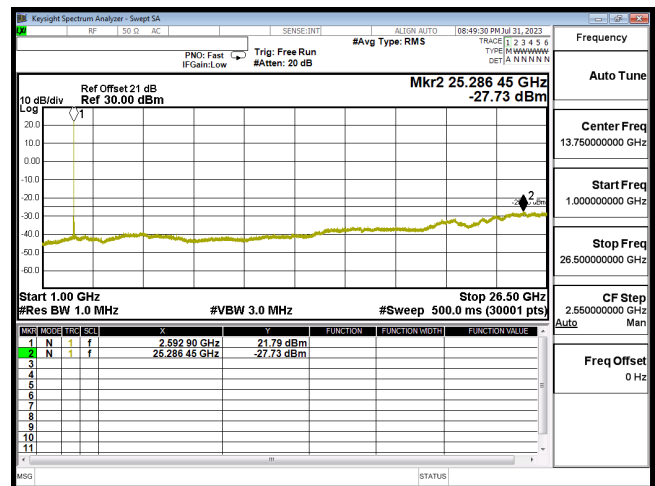
CSE B41 15M CH40620 QPSK(1,37) 1G-26.5G
