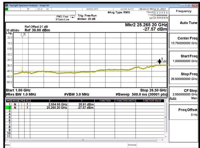
CSE B41 20M CH40240 QPSK(1,50) 1G-26.5G
