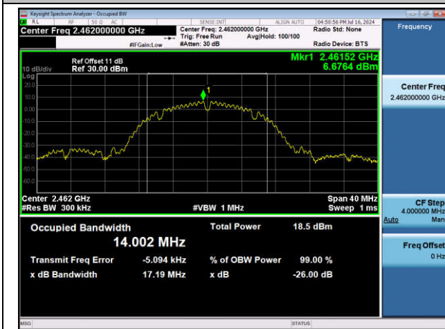
11B-Ant1-2462
