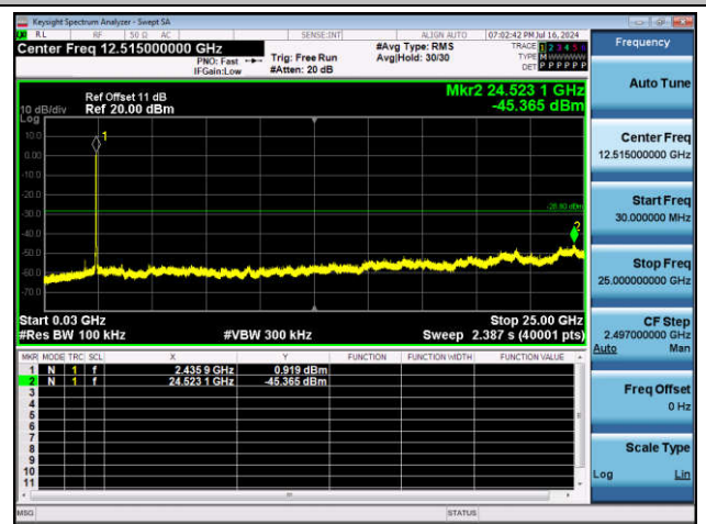
11N20SISO-Ant1-2437-30~25000-PASS
