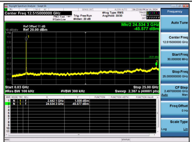
11G-Ant1-2437-30~25000-PASS
