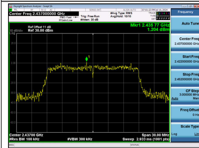
11N20SISO-Ant1-2437-0~Reference-PASS
