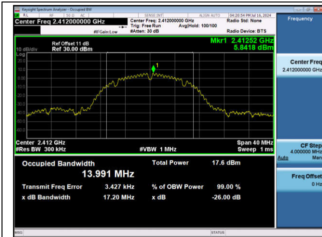
11B-Ant1-2412
