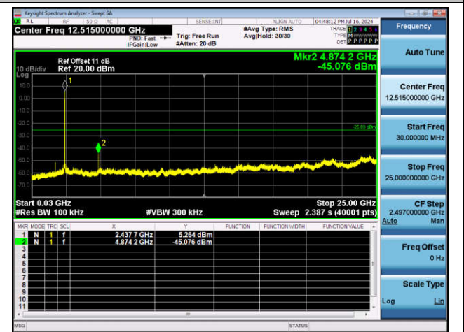
11B-Ant1-2437-30~25000-PASS
