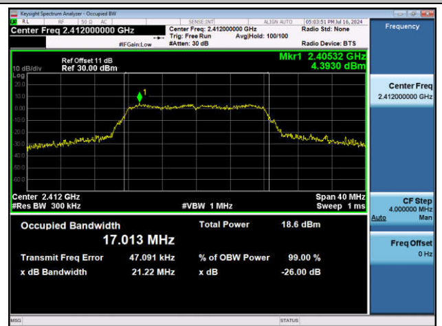
11G-Ant1-2412
