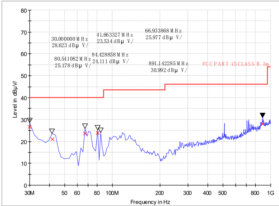
EMI Sweep-3M(30-1G)
