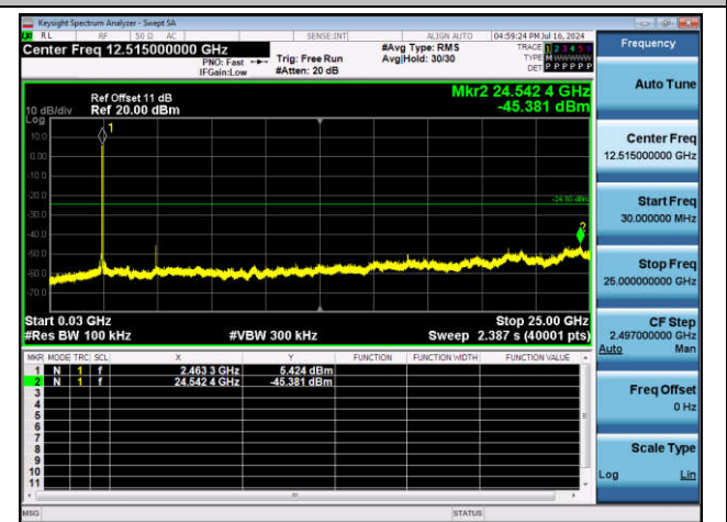
11B-Ant1-2462-30~25000-PASS
