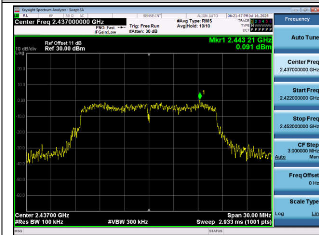
11G-Ant1-2437-0~Reference-PASS
