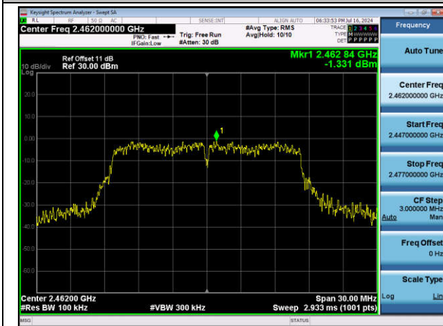
11G-Ant1-2462-0~Reference-PASS
