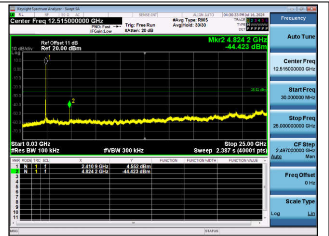
11B-Ant1-2412-30~25000-PASS
