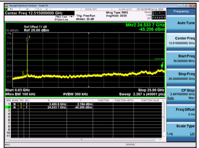
11N20SISO-Ant1-2462-30~25000-PASS
