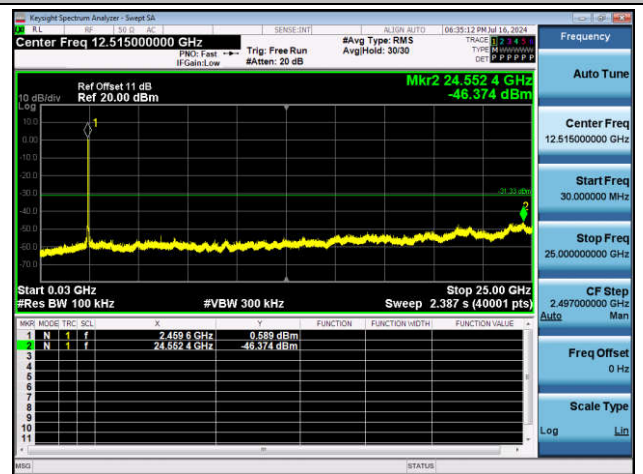
11G-Ant1-2462-30~25000-PASS
