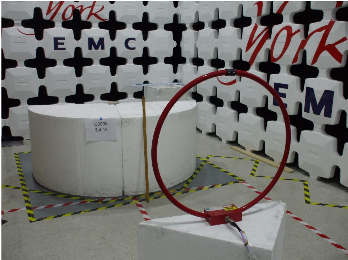
Radiated emissions 9kHz to 30MHz
