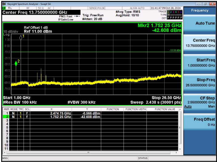
2.4G-Ant1-2475-1000~26500-PASS
