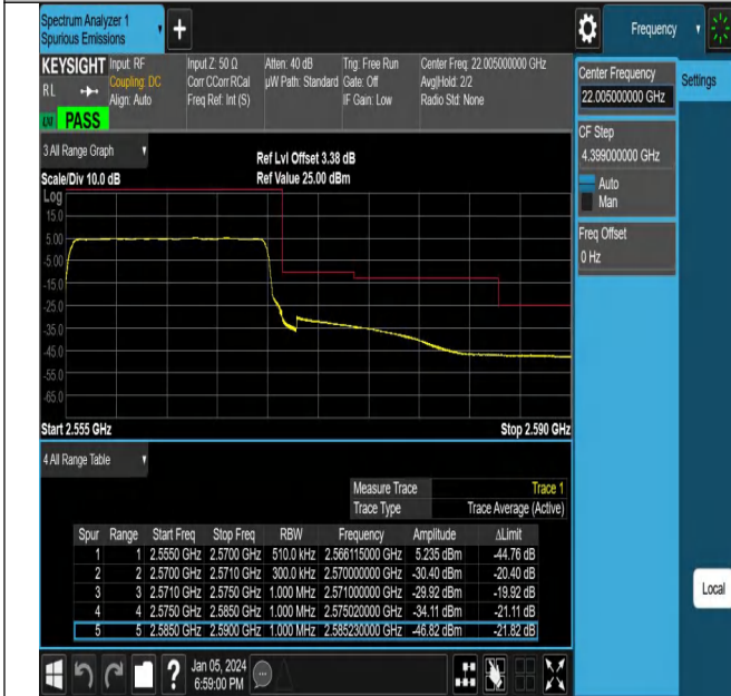
NTNV_N7_PC3_15_15_H_TID13_#1
