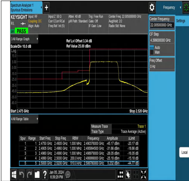
NTNV_N7_PC3_15_10_L_TID25_#1
