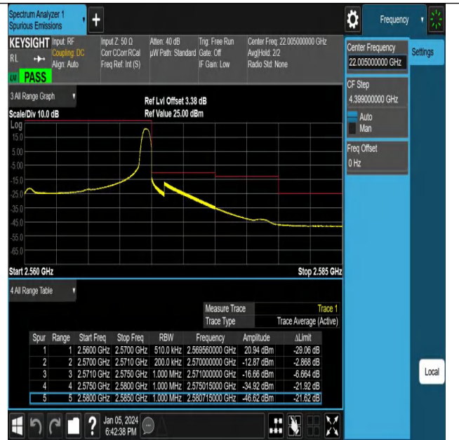
NTNV_N7_PC3_15_10_H_TID12_#1
