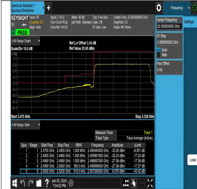
NTNV_N7_PC3_15_20_L_TID4_#1
