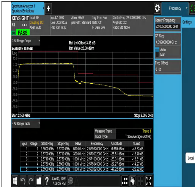
NTNV_N7_PC3_15_20_H_TID4_#1
