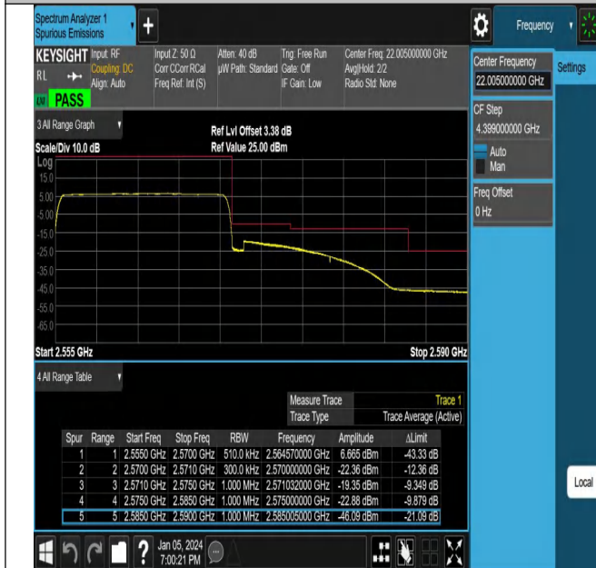
NTNV_N7_PC3_15_15_H_TID19_#1
