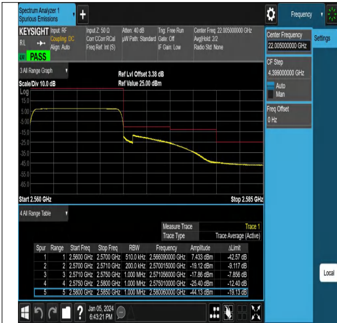
NTNV_N7_PC3_15_10_H_TID16_#1
