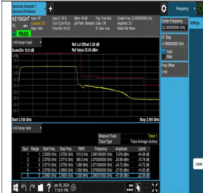
NTNV_N7_PC3_15_20_H_TID7_#1
