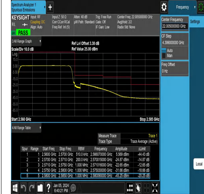
NTNV_N7_PC3_15_10_H_TID1_#1
