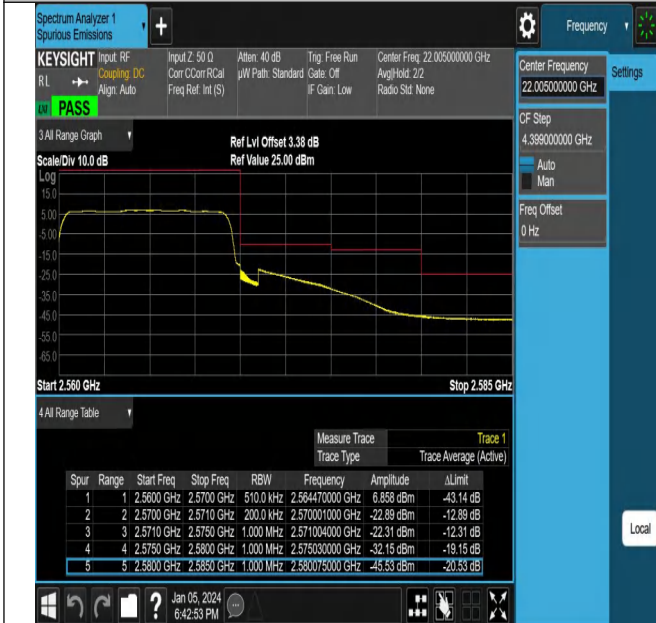
NTNV_N7_PC3_15_10_H_TID13_#1
