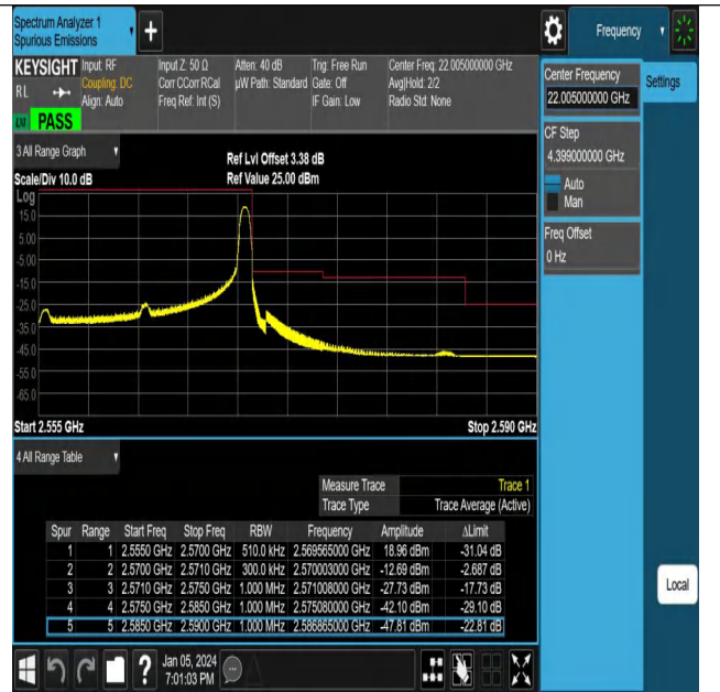
NTNV_N7_PC3_15_15_H_TID24_#1
