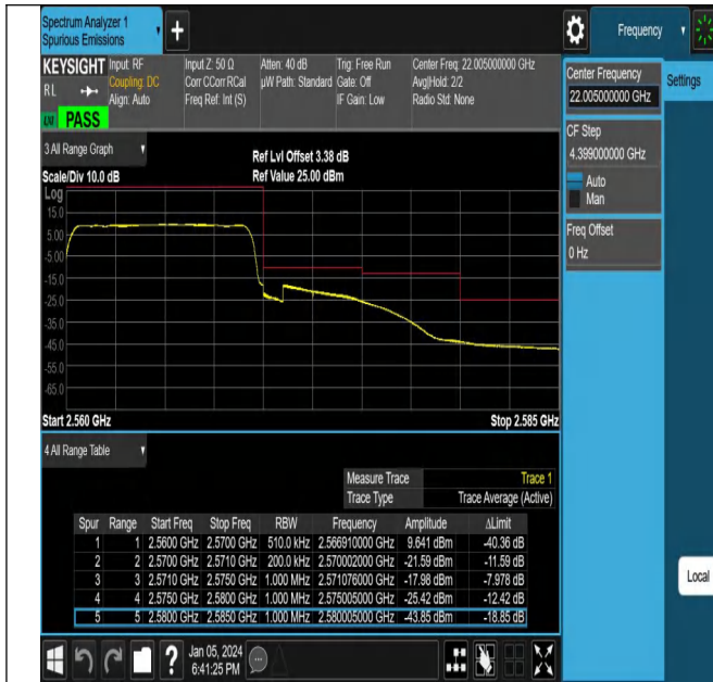
NTNV_N7_PC3_15_10_H_TID4_#1
