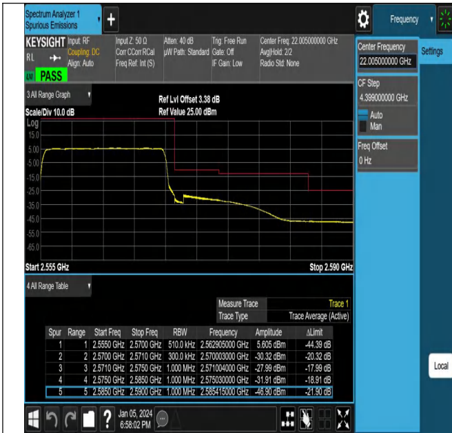
NTNV_N7_PC3_15_15_H_TID10_#1
