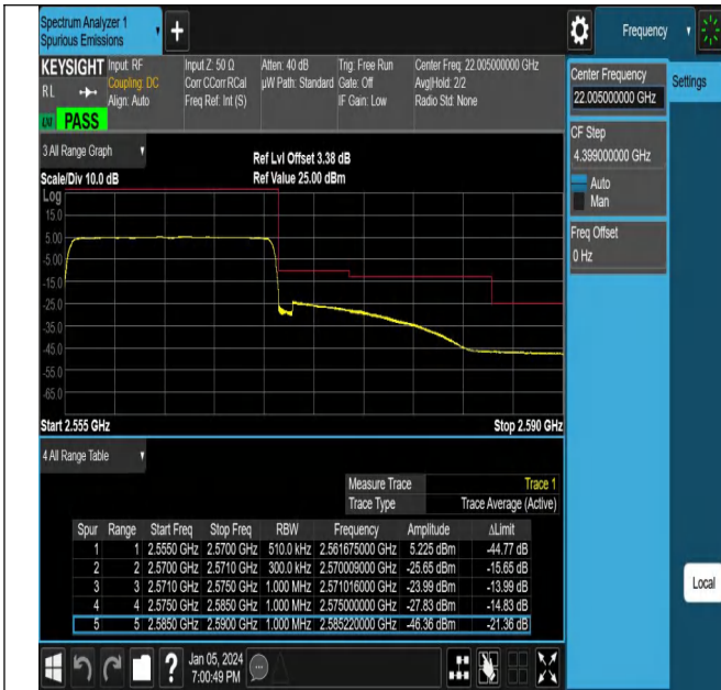
NTNV_N7_PC3_15_15_H_TID22_#1
