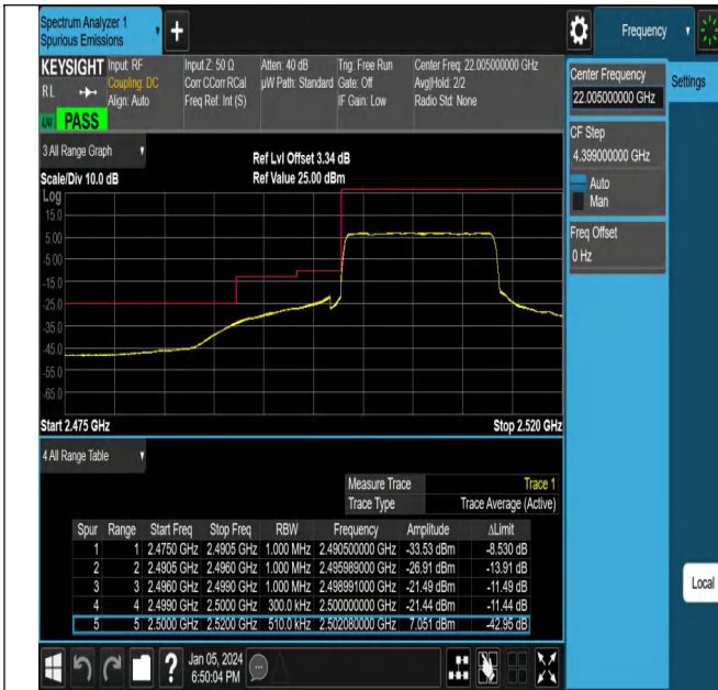
NTNV_N7_PC3_15_15_L_TID7_#1
