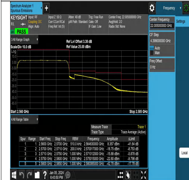
NTNV_N7_PC3_15_10_H_TID19_#1
