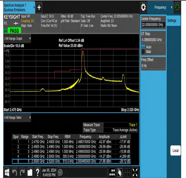
NTNV_N7_PC3_15_15_L_TID5_#1
