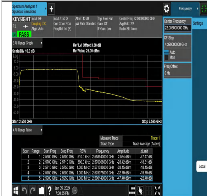
NTNV_N7_PC3_15_20_H_TID1_#1
