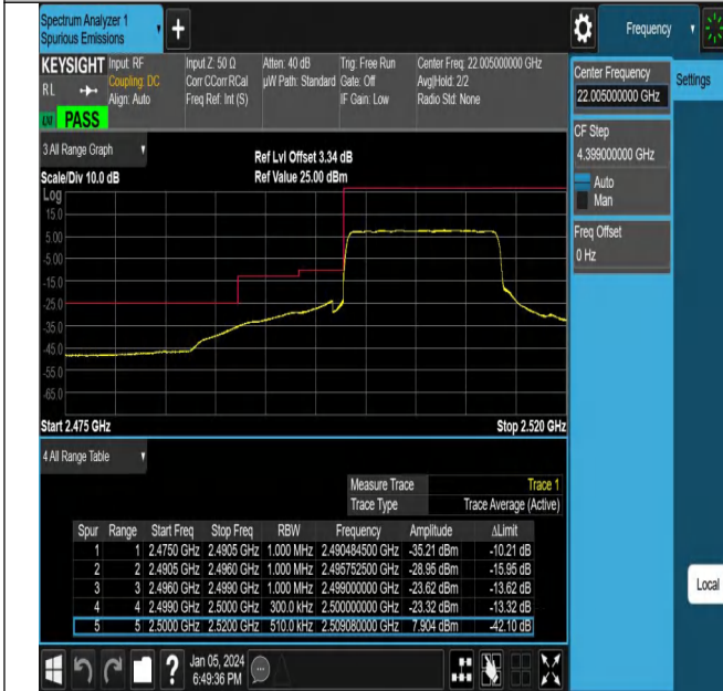
NTNV_N7_PC3_15_15_L_TID4_#1
