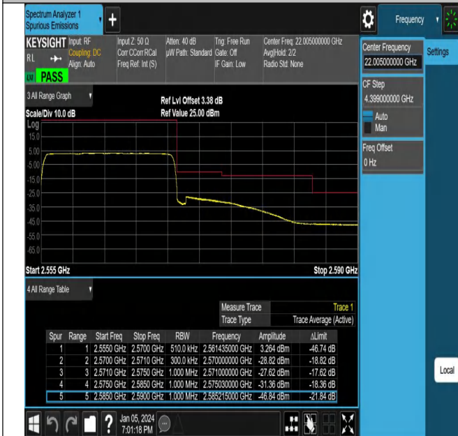
NTNV_N7_PC3_15_15_H_TID25_#1
