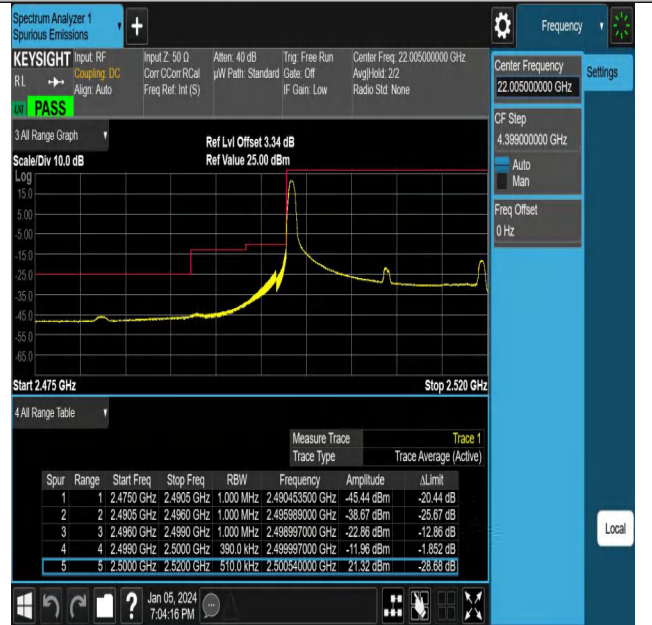
NTNV_N7_PC3_15_20_L_TID5_#1
