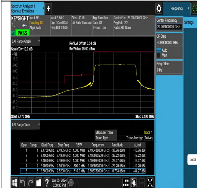
NTNV_N7_PC3_15_15_L_TID10_#1
