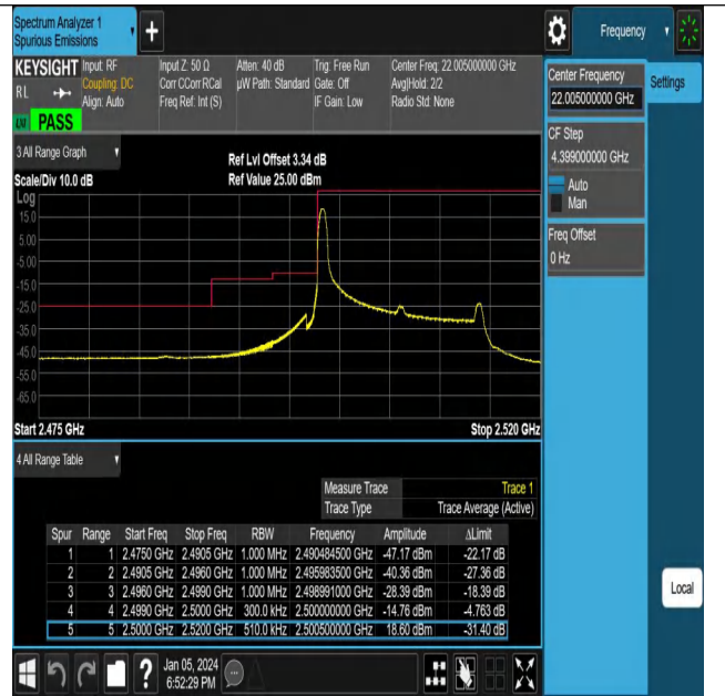
NTNV_N7_PC3_15_15_L_TID14_#1
