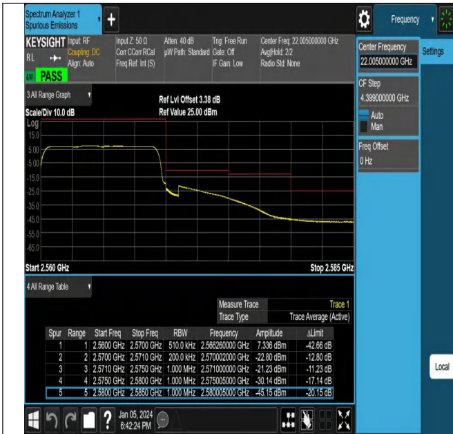
NTNV_N7_PC3_15_10_H_TID10_#1
