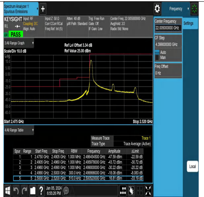
NTNV_N7_PC3_15_15_L_TID26_#1
