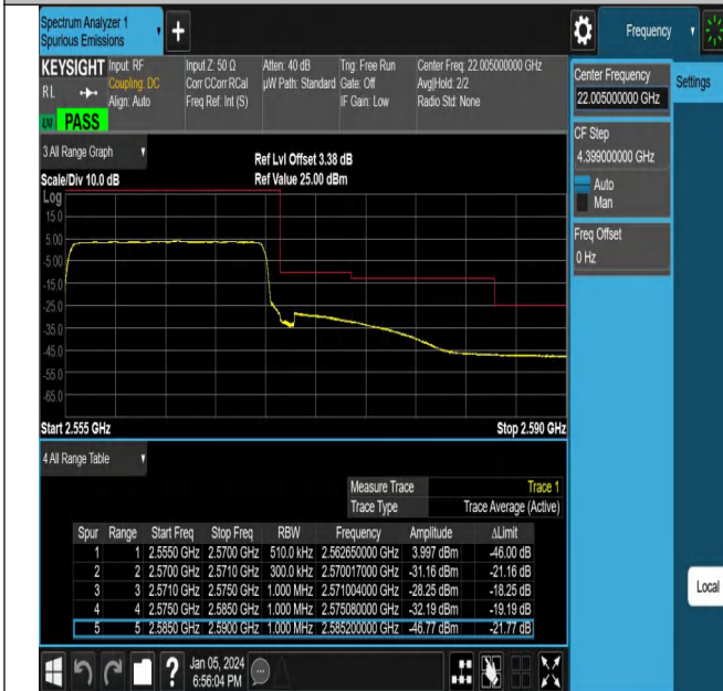
NTNV_N7_PC3_15_15_H_TID1_#1
