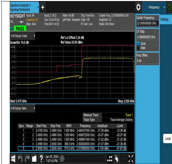
NTNV_N7_PC3_15_20_L_TID25_#1
