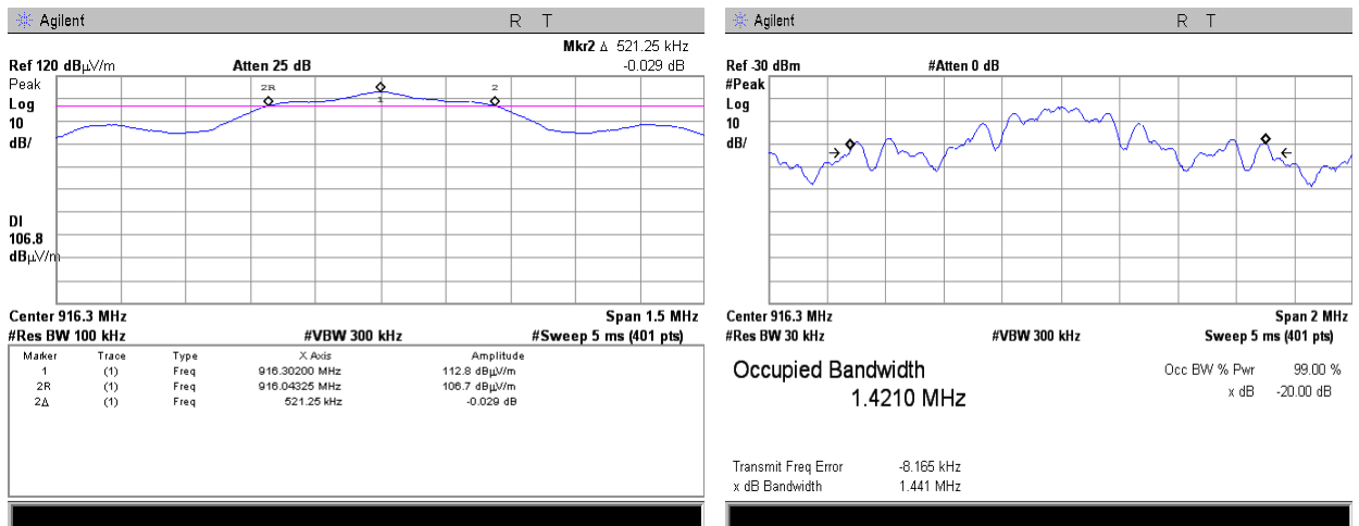
Plot 7.1.3 The 6 dB bandwidth and 99% occupied bandwidth test results at mid frequency, BPSK modulation
