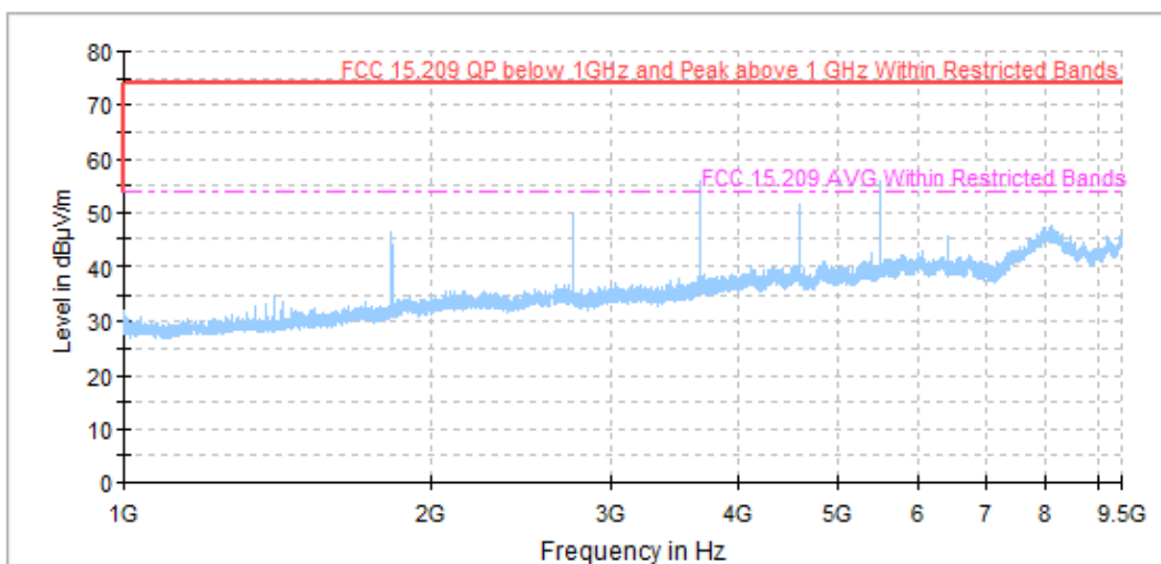
Plot 7.3.12 Radiated emission measurements from 1000 to 9500 MHz at the high carrier frequency, BPSK modulation
