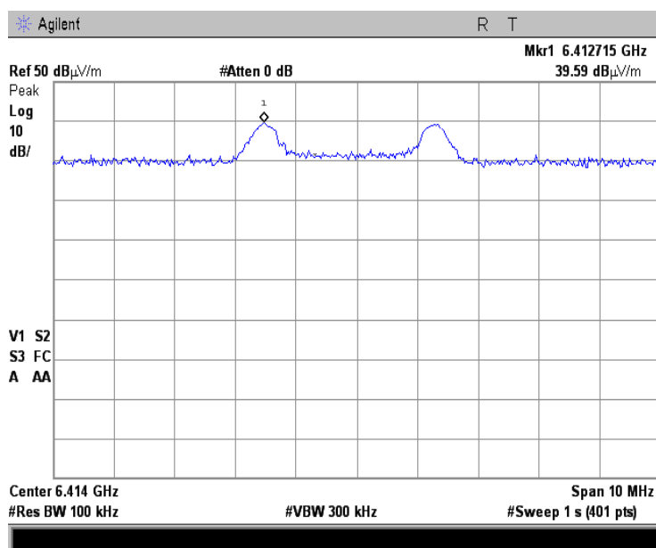
Plot 7.3.34 Radiated emission measurements at the seventh harmonic of low carrier frequency, BPSK modulation
