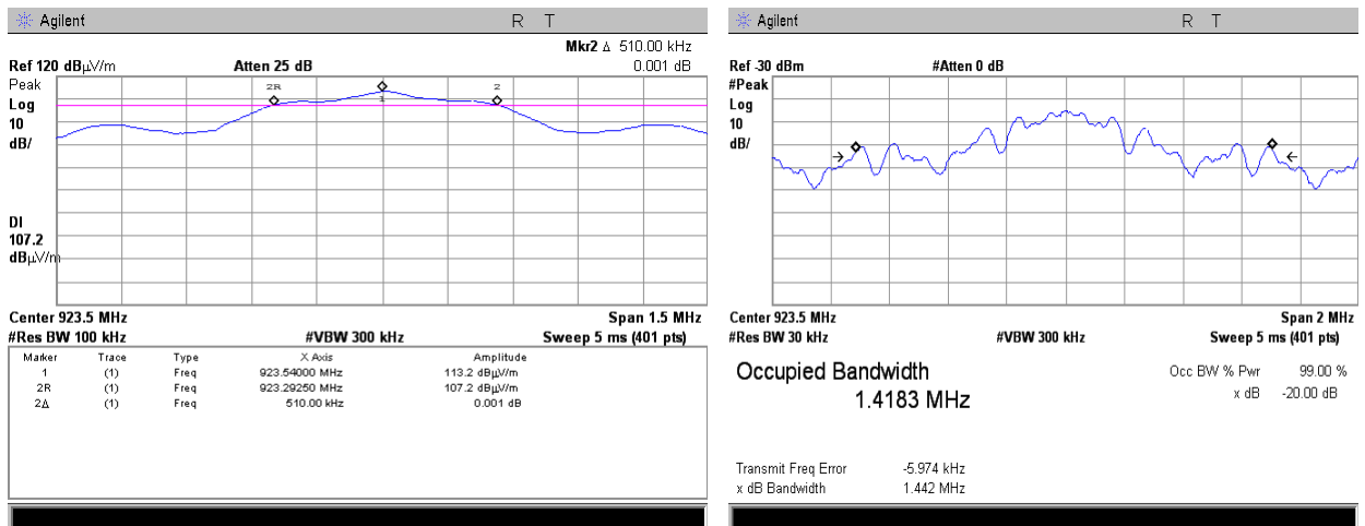
Plot 7.1.4 The 6 dB bandwidth and 99% occupied bandwidth test results at high frequency, BPSK modulation
