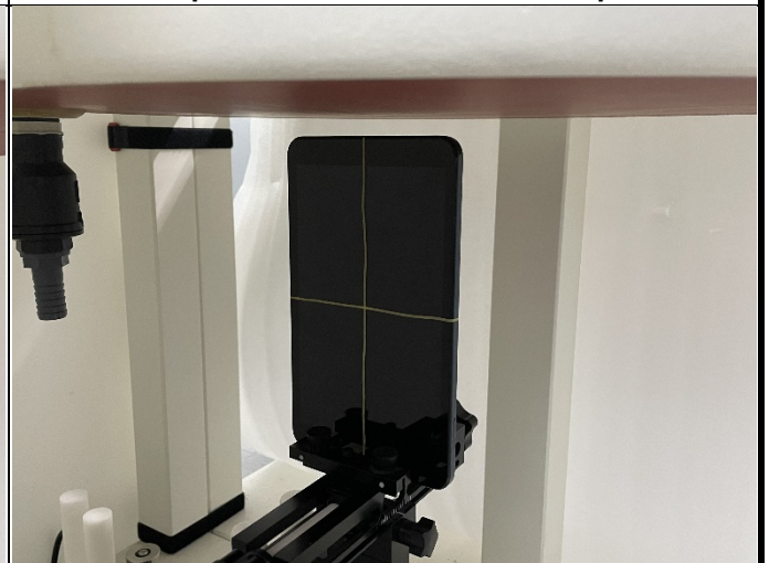
Bottom Side of EUT with 1.2 cm Gap
