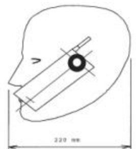
Fig. 10 Cheek/Touch Position
