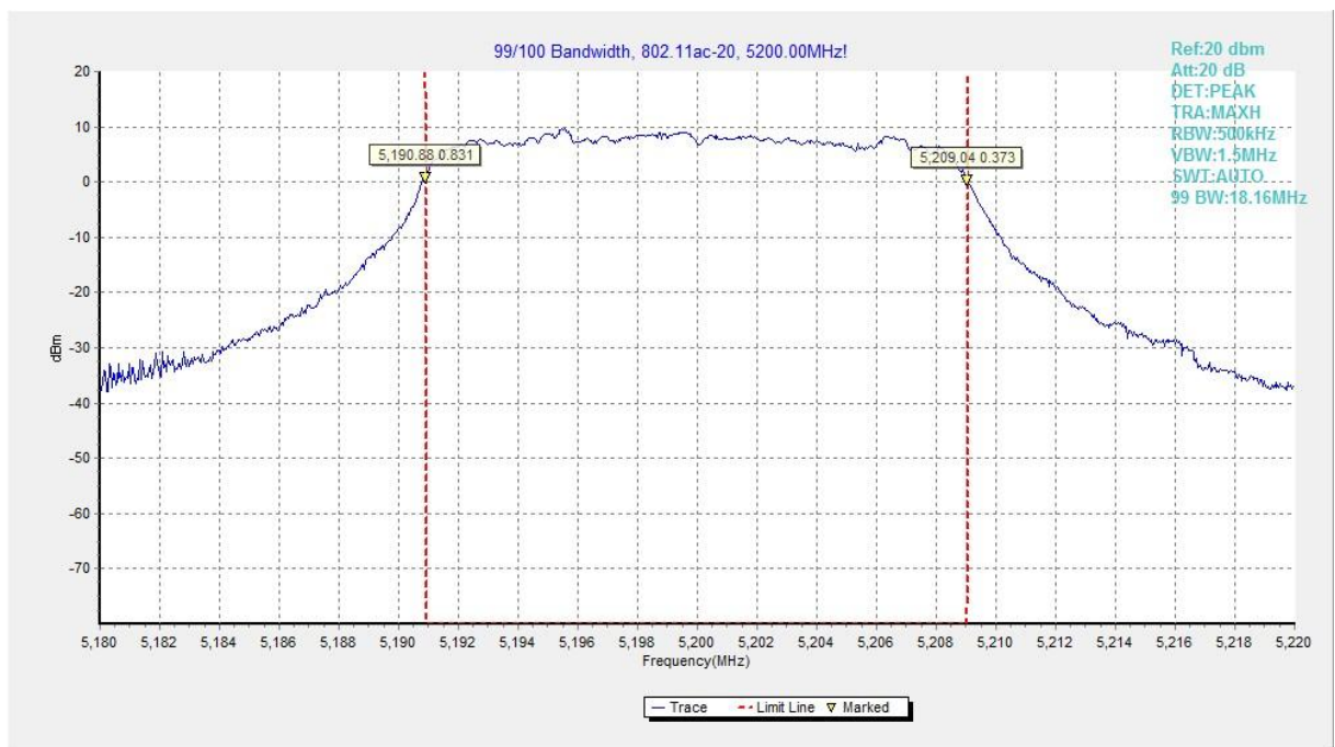
Fig. 78 99% Occupied bandwidth (802.11ac-HT20, 5200MHz)
