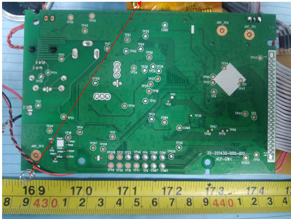
Bluetooth Antenna
