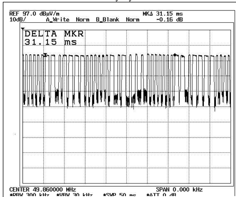
Duty Cycle
