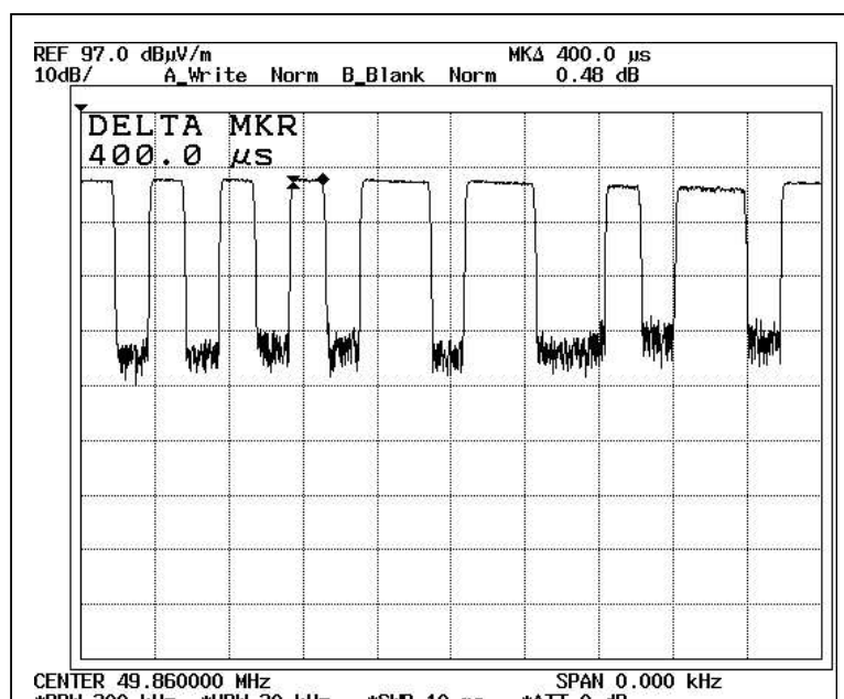
Duty Cycle 3
