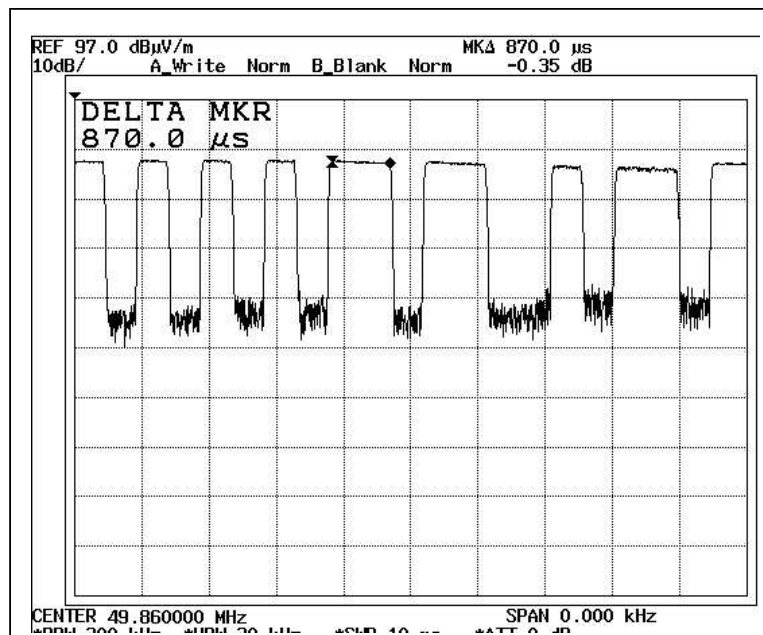
Duty Cycle 2
