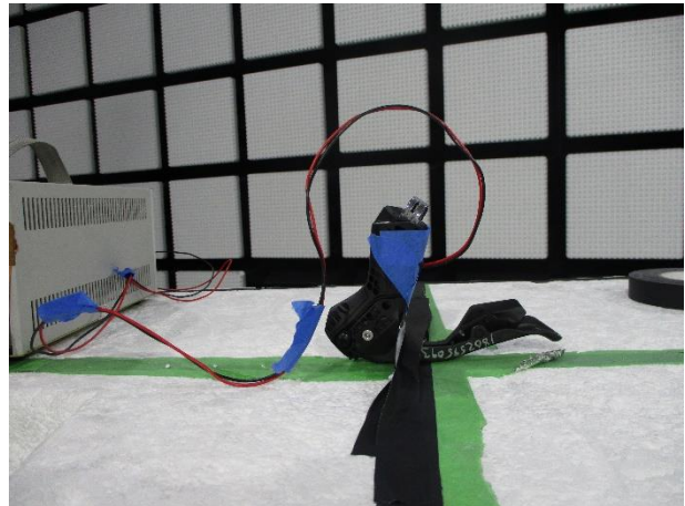
Y-ORIENTATION (Worst-case)
