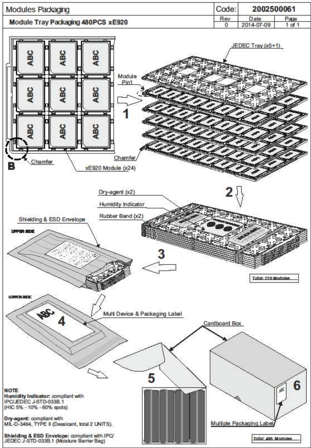
Figure 30: Tray Packing
