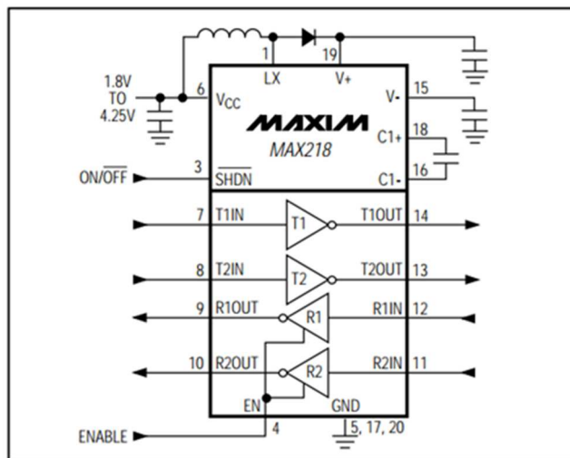
Figure 15: RS232 Level Adaption Circuitry Example
