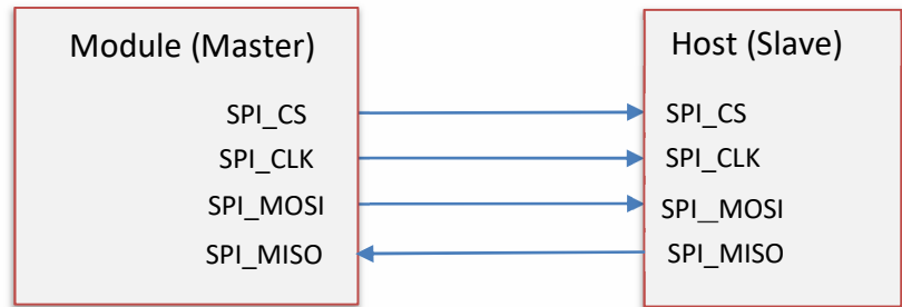
Figure 17: SPI Signal Connectivity
