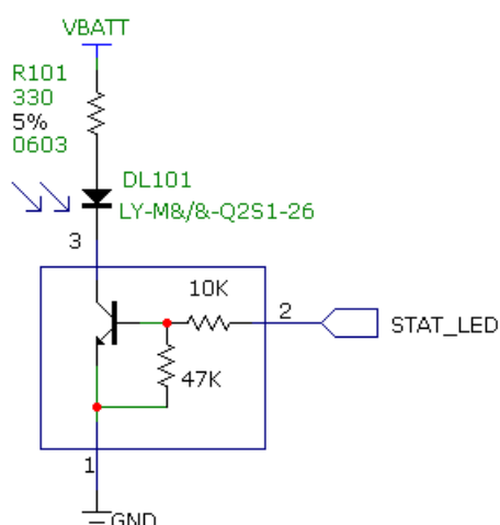
Figure 22: Status LED Reference Circuit
