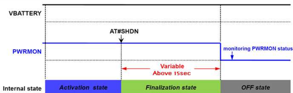
Figure 5: Shutdown by Software Command
