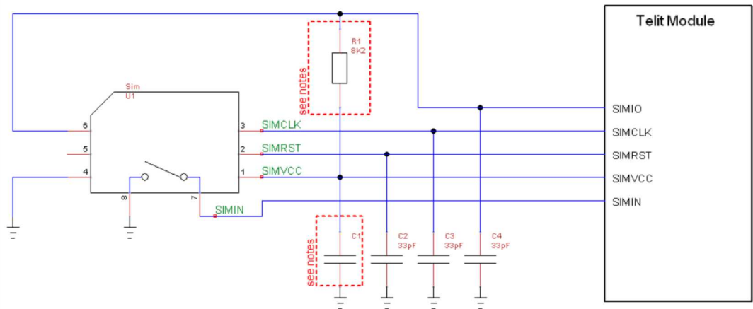
Figure 29: SIM Schematics
