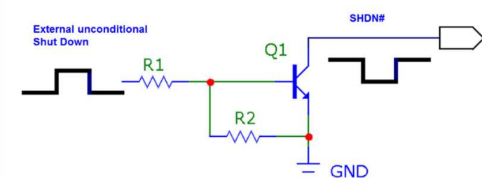
Figure 9: Circuit for Unconditional Hardware Shutdown
