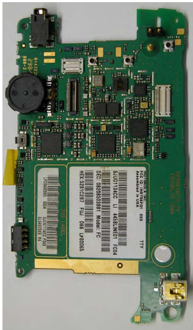
Rear View without shields
