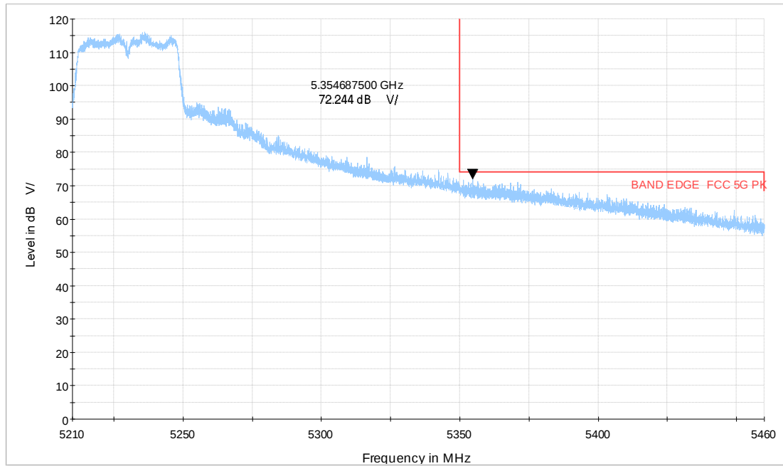
Wi-Fi 5G_n40 CH46_5.21-5.46GHz_MCS0_MIMO_V_TP24_PK
