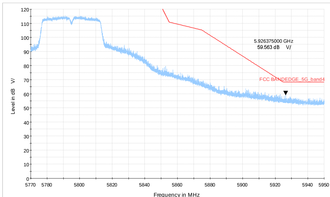
Wi-Fi 5G_n40 CH159_5.77-5.95GHz_MCS0_MIMO_V_TP24
