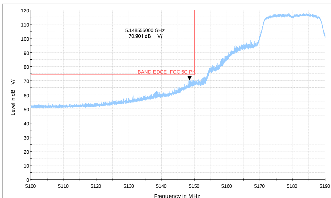
Wi-Fi 5G_n20 CH36_5.1-5.19GHz_MCS0_MIMO_V_TP23_PK
