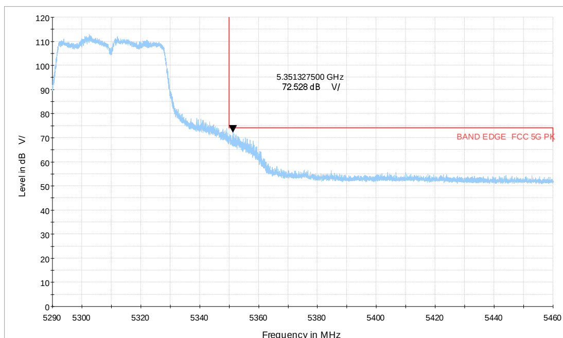
Wi-Fi 5G_n40 CH62_5.29-5.46GHz_MCS0_MIMO_V_TP19_PK
