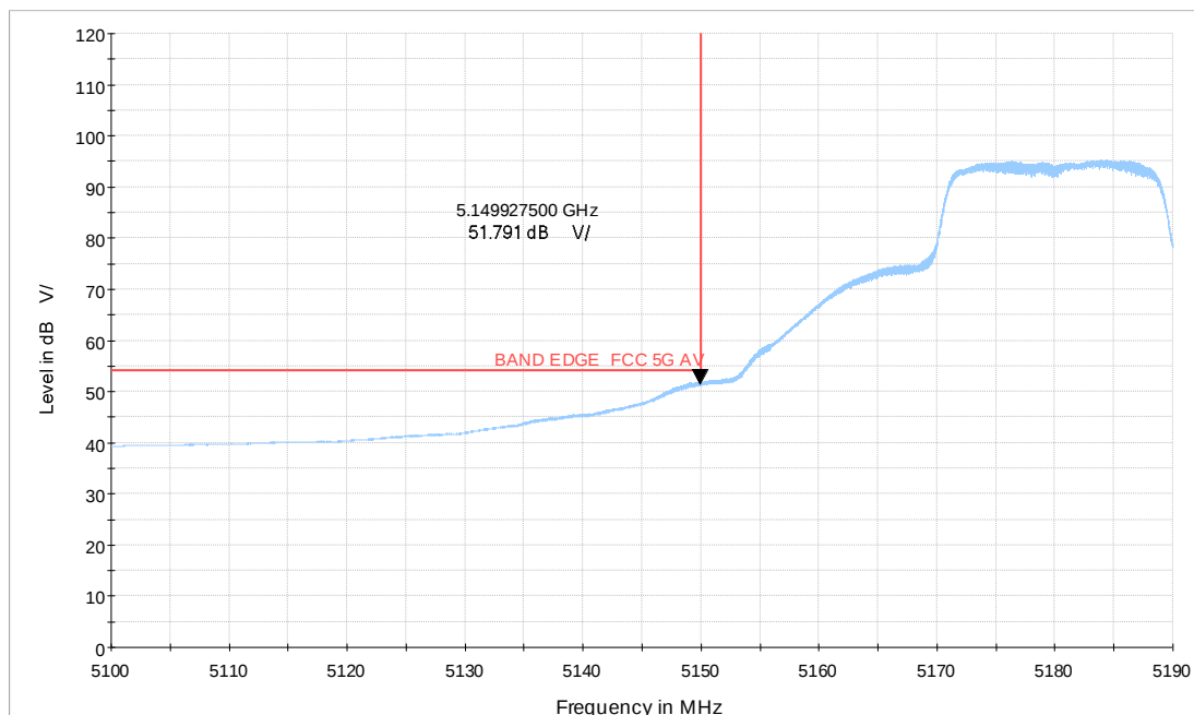
Wi-Fi 5G_n20 CH36_5.1-5.19GHz_MCS0_MIMO_V_TP23_AV
