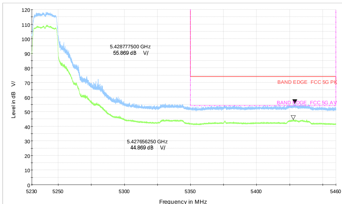
Wi-Fi 5G_n20 CH48_5.23-5.46GHz_MCS0_MIMO_V_TP24
