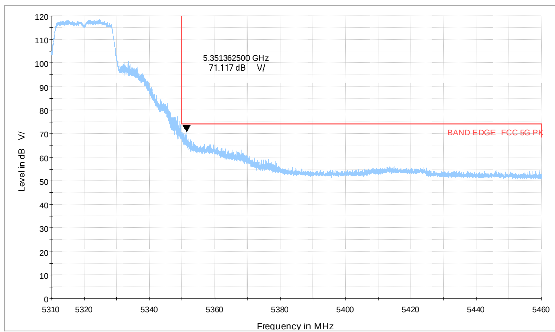
Wi-Fi 5G_n20 CH64_5.31-5.46GHz_MCS0_MIMO_V_TP24_PK
