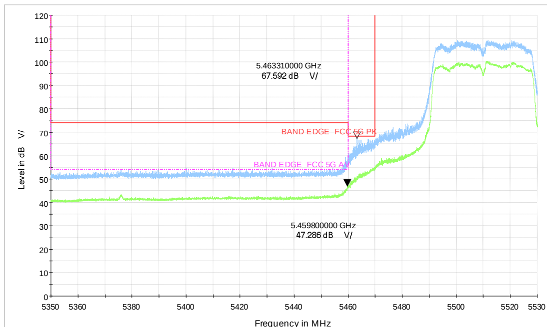
Wi-Fi 5G_n40 CH102_5.35-5.53GHz_MCS0_MIMO_V_TP15
