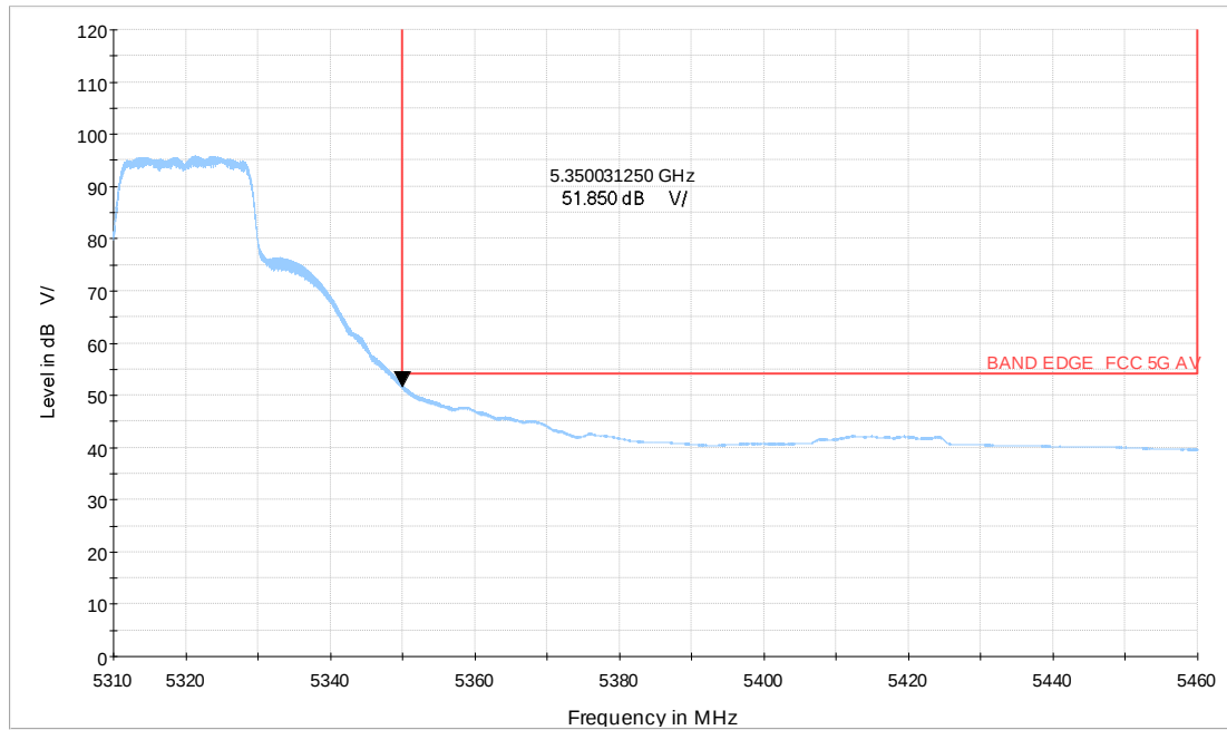
Wi-Fi 5G_n20 CH64_5.31-5.46GHz_MCS0_MIMO_V_TP24_AV
