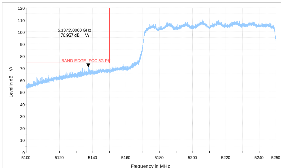
Wi-Fi 5G_ax80 CH42_5.1-5.25GHz_MCS0_MIMO_V_TP17_PK
