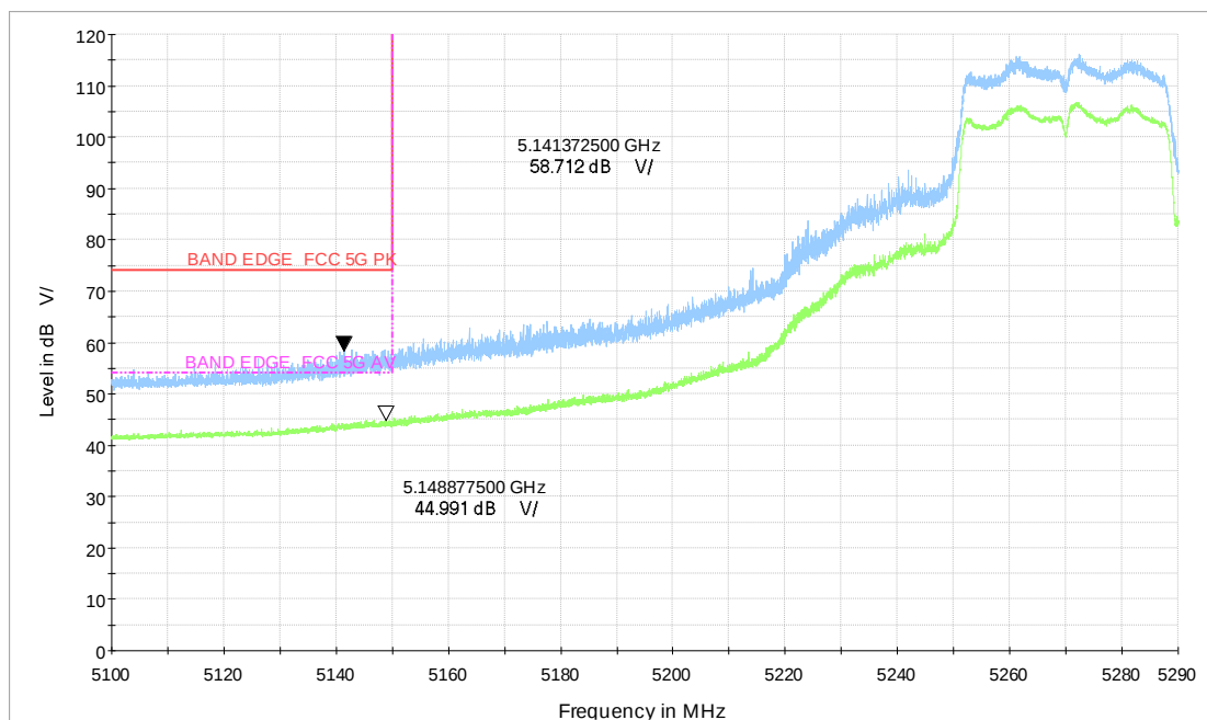
Wi-Fi 5G_n40 CH54_5.1-5.29GHz_MCS0_MIMO_V_TP24
