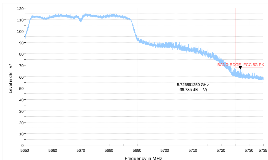
Wi-Fi 5G_n40 CH134_5.65-5.735GHz_MCS0_MIMO_V_TP23
