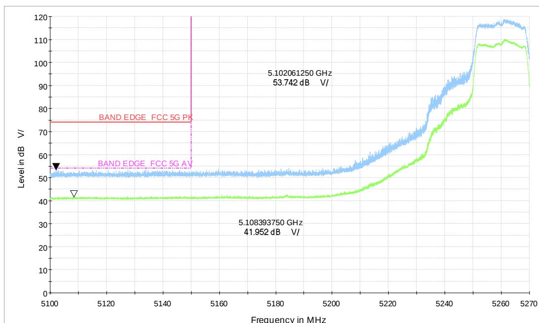
Wi-Fi 5G_n20 CH52_5.1-5.27GHz_MCS0_MIMO_V_TP24
