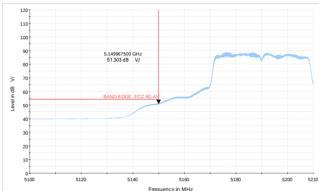
Wi-Fi 5G_n40 CH38_5.1-5.21GHz_MCS0_MIMO_V_TP18_AV
