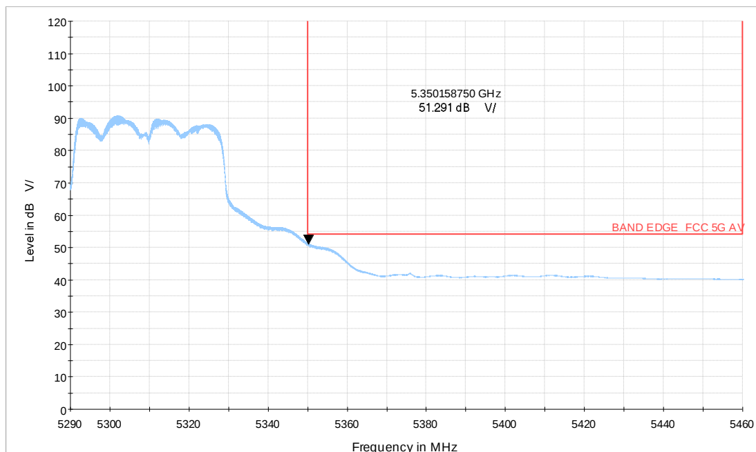
Wi-Fi 5G_n40 CH62_5.29-5.46GHz_MCS0_MIMO_V_TP19_AV
