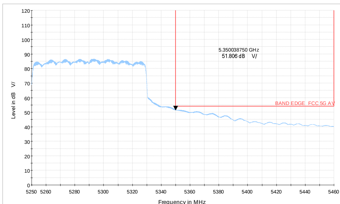
Wi-Fi 5G_ax80 CH58_5.25-5.46GHz_MCS0_MIMO_V_TP17_AV
