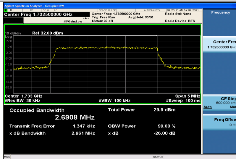
Band4-3MHz-QPSK-20175-15RB#0-2.6908
