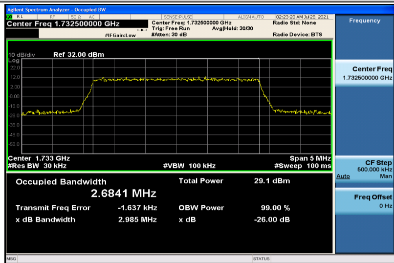
Band4-3MHz-16QAM-20175-15RB#0-2.6841
