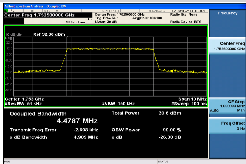
Band4-5MHz-QPSK-20375-25RB#0-4.4787
