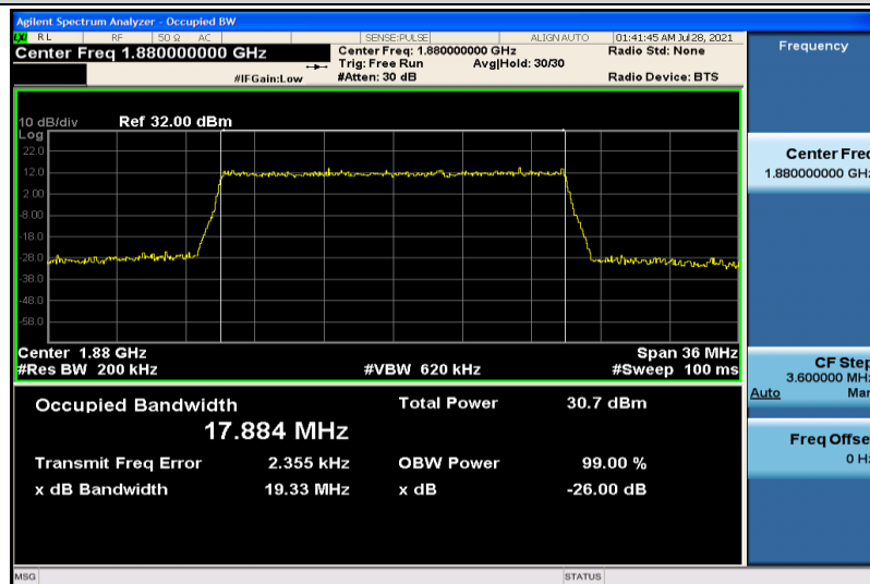
Band2-20MHz-QPSK-18900-100RB#0-17.884
