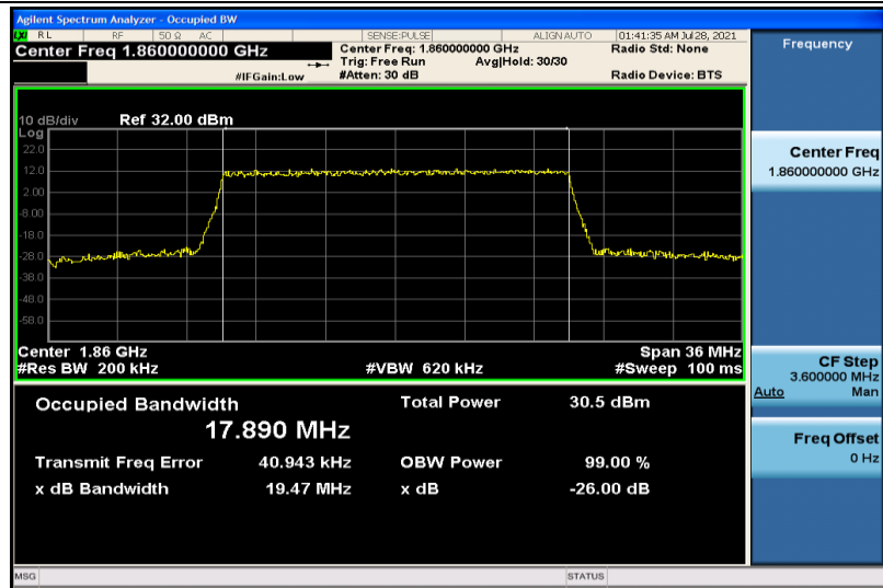
Band2-20MHz-16QAM-18700-100RB#0-17.890
