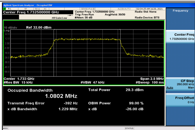
Band4-1.4MHz-QPSK-20175-6RB#0-1.0802
