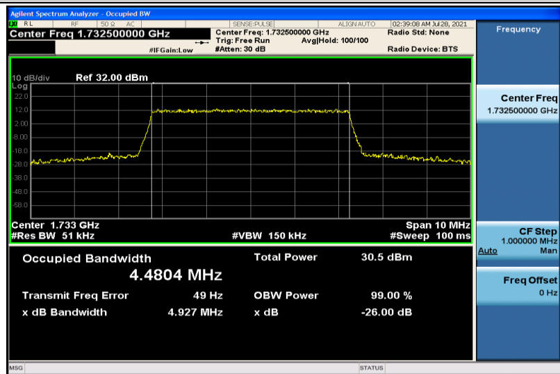
Band4-5MHz-QPSK-20175-25RB#0-4.4804
