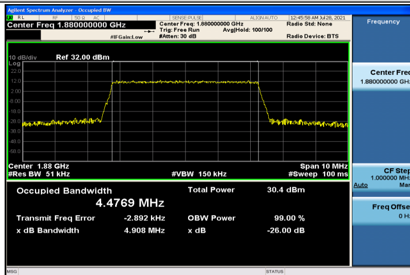
Band2-5MHz-QPSK-18900-25RB#0-4.4769
