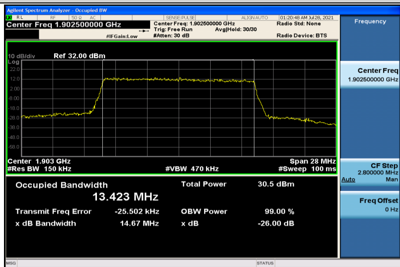
Band2-15MHz-QPSK-19125-75RB#0-13.423
