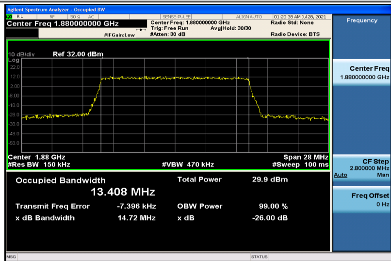
Band2-15MHz-16QAM-18900-75RB#0-13.408
