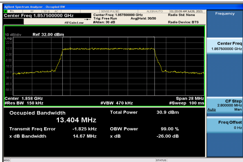
Band2-15MHz-QPSK-18675-75RB#0-13.404
