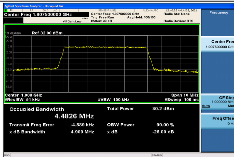
Band2-5MHz-QPSK-19175-25RB#0-4.4826
