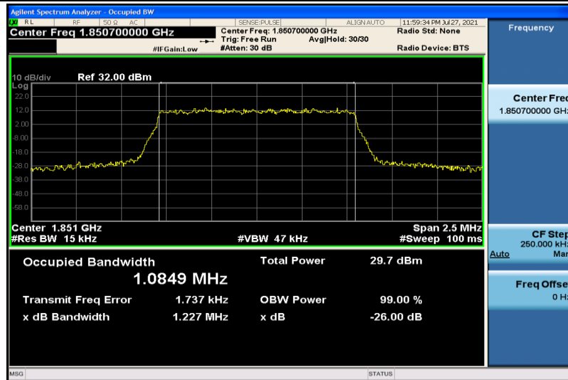
Band2-1.4MHz-QPSK-18607-6RB#0-1.0849
