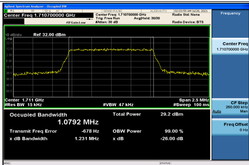
Band4-1.4MHz-QPSK-19957-6RB#0-1.0792
