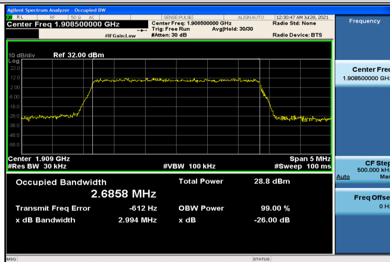
Band2-3MHz-16QAM-19185-15RB#0-2.6858
