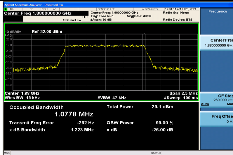
Band2-1.4MHz-QPSK-18900-6RB#0-1.0778
