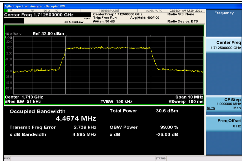
Band4-5MHz-QPSK-19975-25RB#0-4.4674
