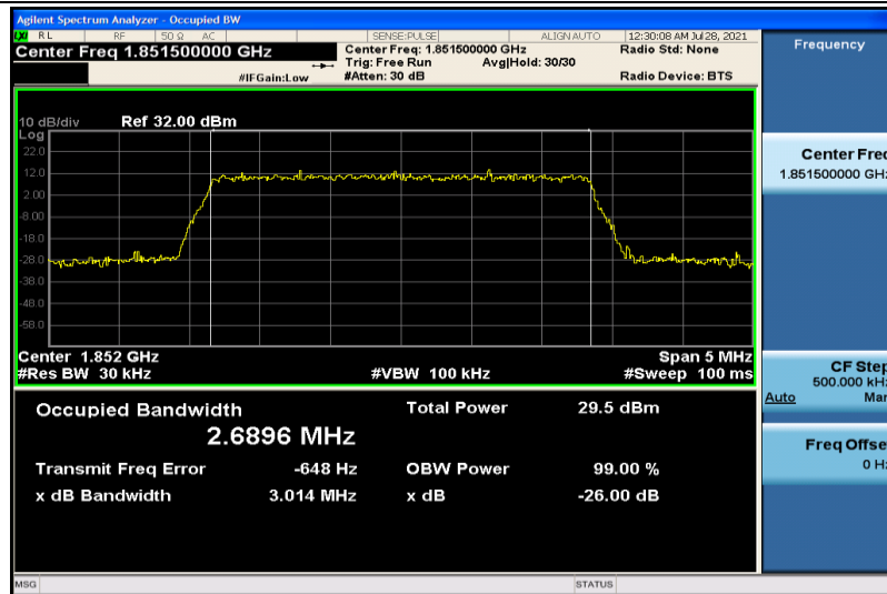
Band2-3MHz-16QAM-18615-15RB#0-2.6896
