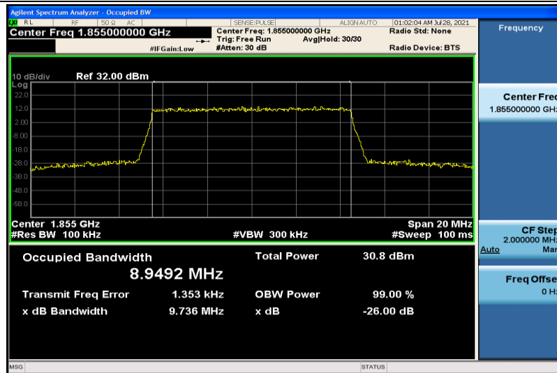
Band2-10MHz-QPSK-18650-50RB#0-8.9492
