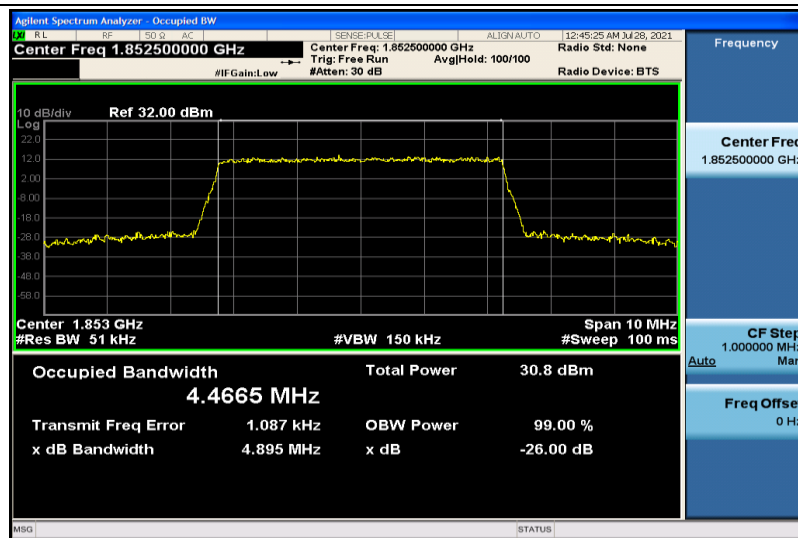
Band2-5MHz-QPSK-18625-25RB#0-4.4665
