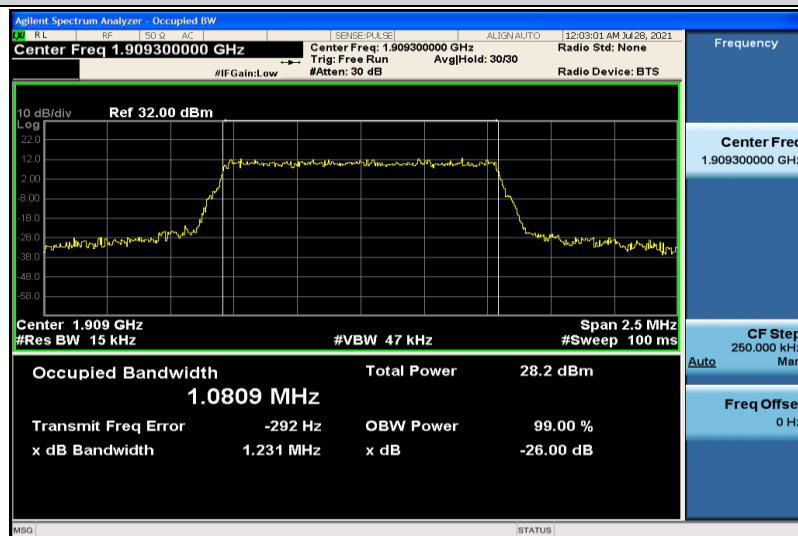
Band2-1.4MHz-16QAM-19193-6RB#0-1.0809
