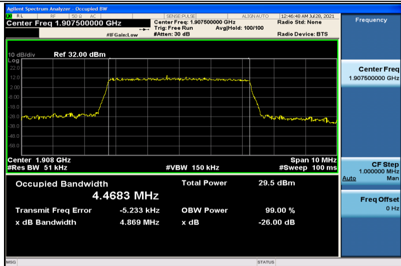
Band2-5MHz-16QAM-19175-25RB#0-4.4683
