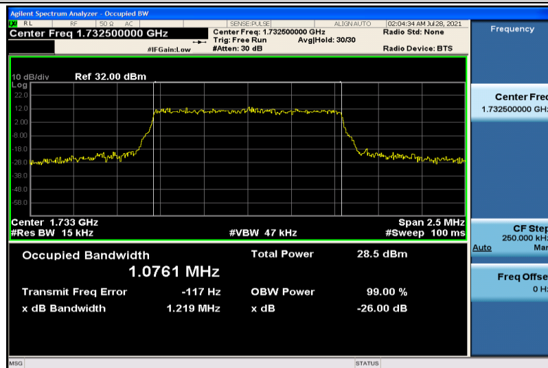
Band4-1.4MHz-16QAM-20175-6RB#0-1.0761
