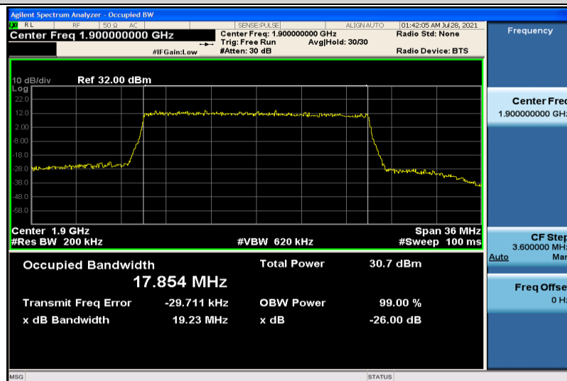
Band2-20MHz-QPSK-19100-100RB#0-17.854
