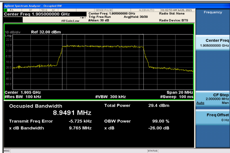
Band2-10MHz-16QAM-19150-50RB#0-8.9491
