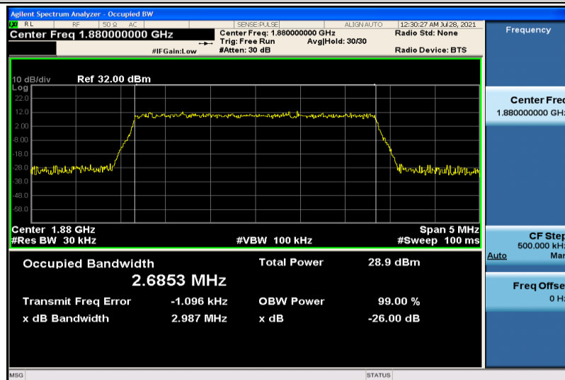
Band2-3MHz-16QAM-18900-15RB#0-2.6853
