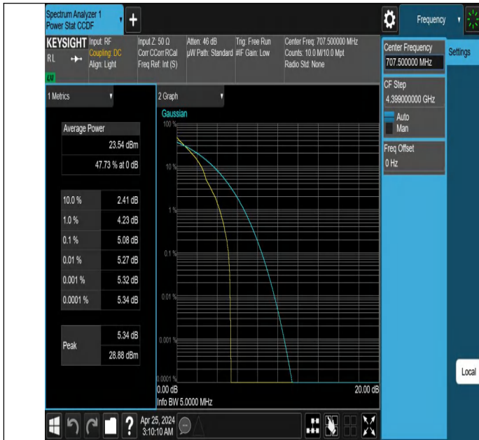
Band12-5MHz-QPSK-23095-1RB#0-PASS
