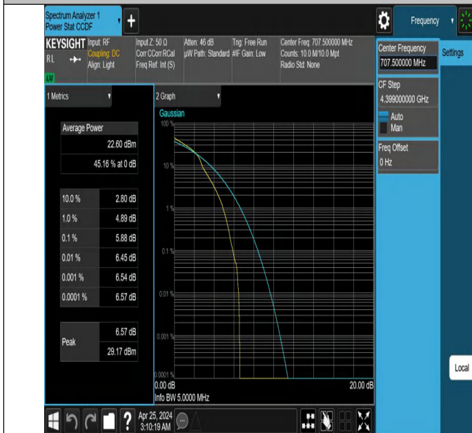
Band12-5MHz-16QAM-23095-1RB#0-PASS
