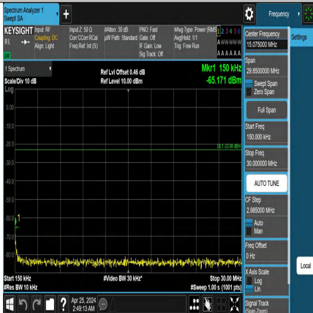
Band12_1.4MHz_QPSK_23017_1RB#5_0.15~30_0.15~30
