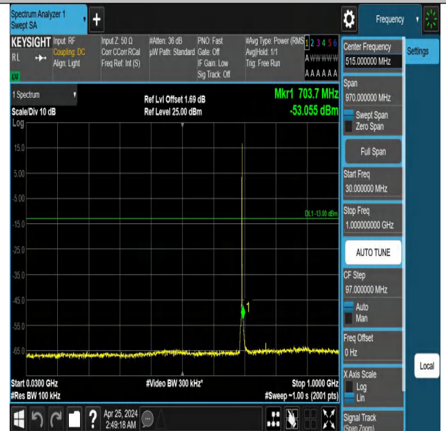
Band12_1.4MHz_QPSK_23017_1RB#5_30~1000_30~1000
