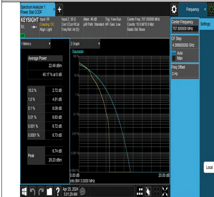
Band12-3MHz-16QAM-23095-1RB#0-PASS
