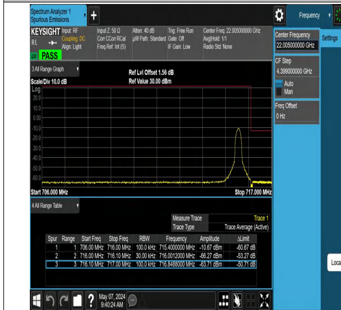
Band12_10MHz_QPSK_23130_1RB#49
