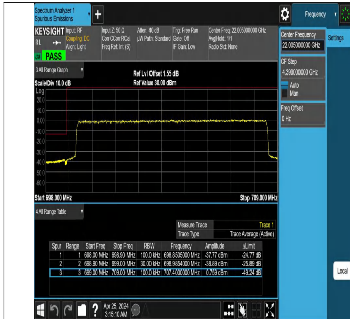
Band12_10MHz_QPSK_23060_50RB#0
