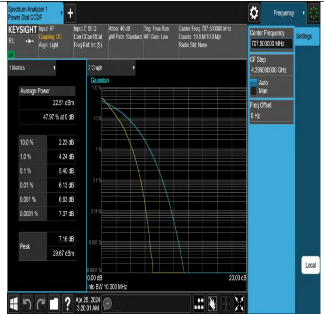
Band12-10MHz-QPSK-23095-50RB#0-PASS
