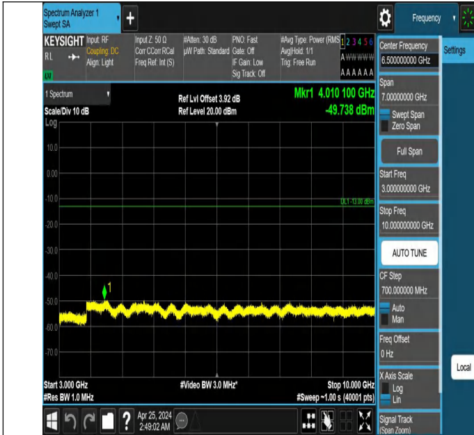
Band12_1.4MHz_QPSK_23017_1RB#0_3000~10000_3000~1000
