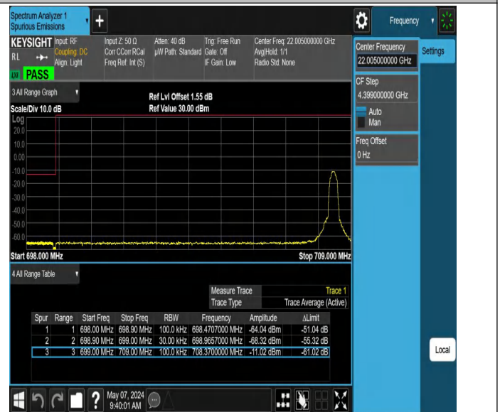
Band12_10MHz_QPSK_23060_1RB#49
