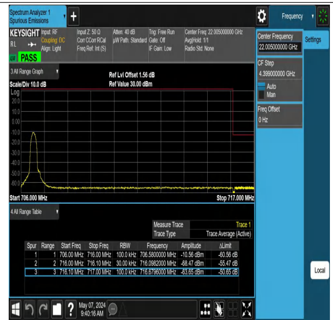
Band12_10MHz_QPSK_23130_1RB#0
