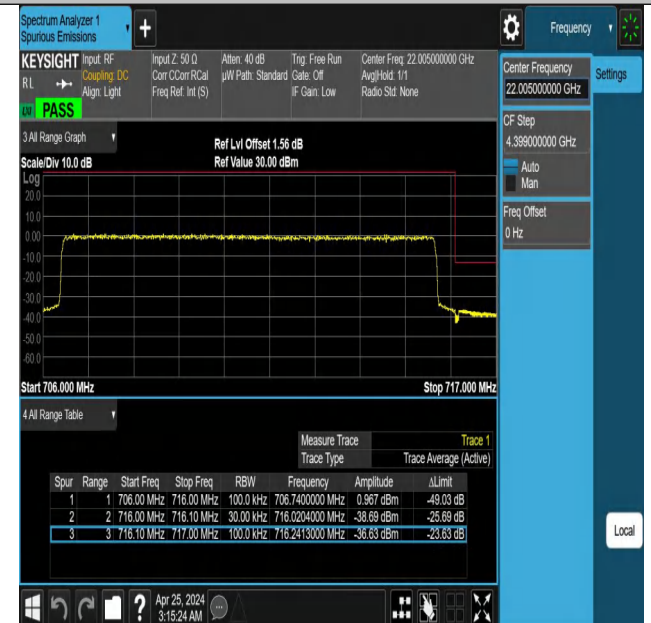
Band12_10MHz_QPSK_23130_50RB#0
