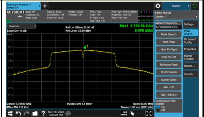
Channel 159 (5795MHz)
