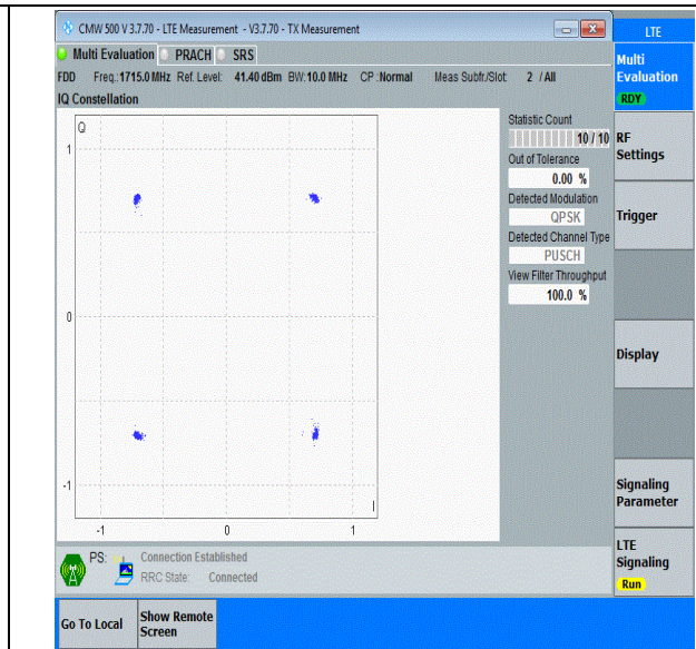
Band66-10MHz-QPSK-132022-50RB#0-PASS
