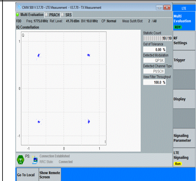
Band66-10MHz-QPSK-132622-50RB#0-PASS
