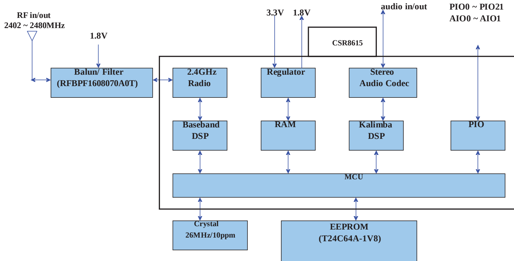
JS-BTM8615 Block Diagram
