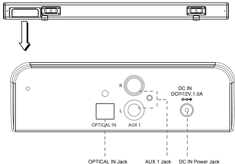
CONTROL PANEL
