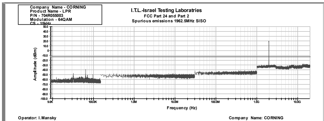
Figure 353: Spurious Emissions at Antenna Terminal 64QAM, 1962.5MHz, B.W. 15MHz, Sub Carrier 15 kHz
