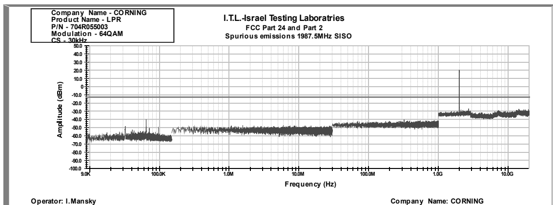
Figure 357: Spurious Emissions at Antenna Terminal 64QAM, 1987.5MHz, B.W. 15MHz, Sub Carrier 30 kHz
