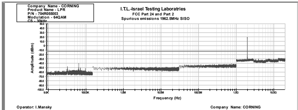
Figure 356: Spurious Emissions at Antenna Terminal 64QAM, 1962.5MHz, B.W. 15MHz, Sub Carrier 30 kHz
