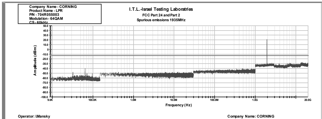
Figure 349: Spurious Emissions at Antenna Terminal 64QAM, 1935.0MHz, B.W. 10MHz, Sub Carrier 60 kHz
