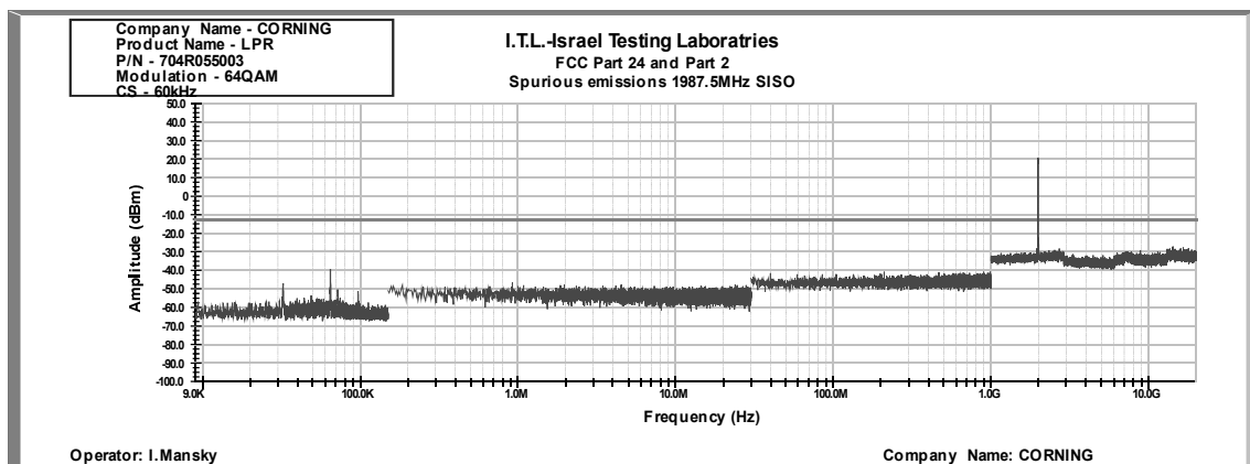
Figure 360: Spurious Emissions at Antenna Terminal 64QAM, 1987.5MHz, B.W. 15MHz, Sub Carrier 60 kHz
