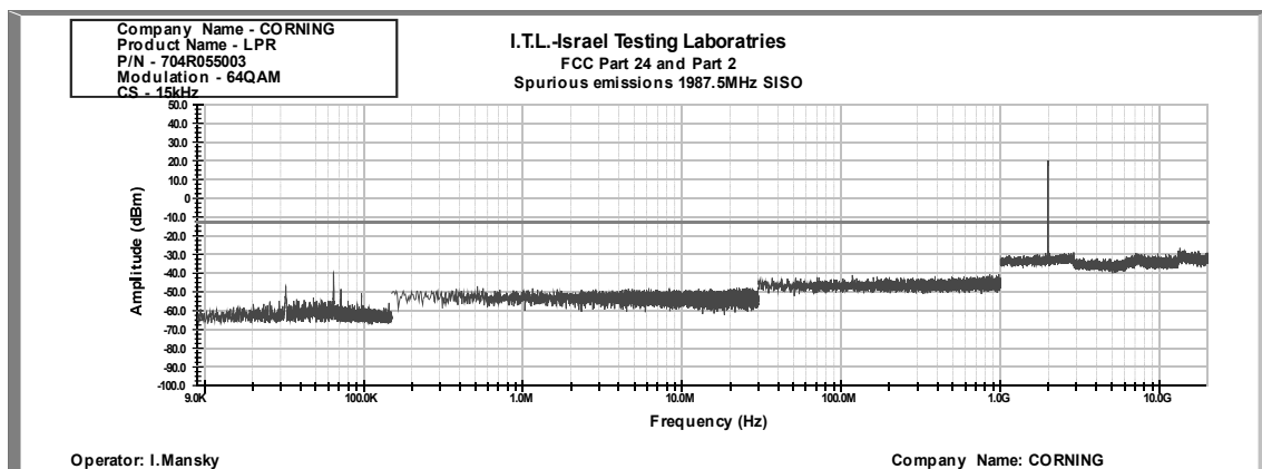
Figure 354: Spurious Emissions at Antenna Terminal 64QAM, 1987.5MHz, B.W. 15MHz, Sub Carrier 15 kHz
