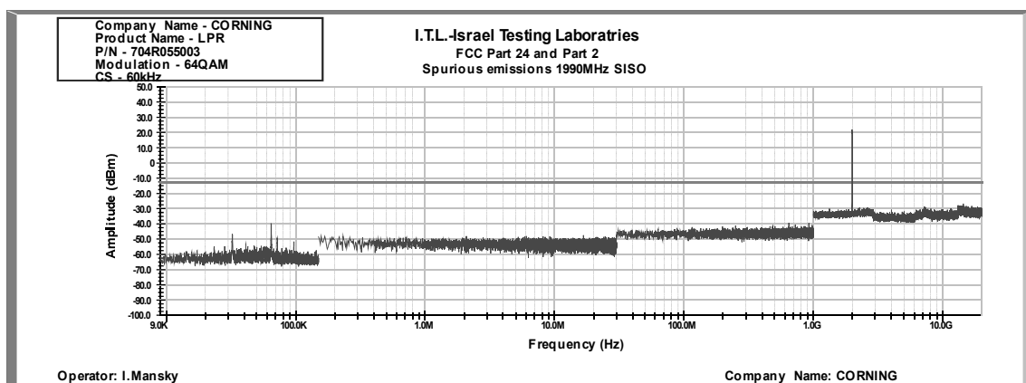
Figure 351: Spurious Emissions at Antenna Terminal 64QAM, 1990.0MHz, B.W. 10MHz, Sub Carrier 60 kHz
