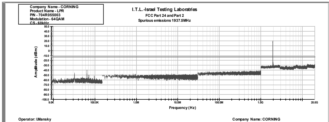
Figure 358: Spurious Emissions at Antenna Terminal 64QAM, 1937.5MHz, B.W. 15MHz, Sub Carrier 60 kHz
