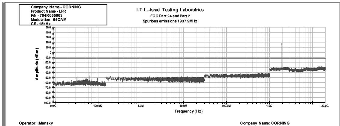
Figure 352: Spurious Emissions at Antenna Terminal 64QAM, 1937.5MHz, B.W. 15MHz, Sub Carrier 15 kHz
