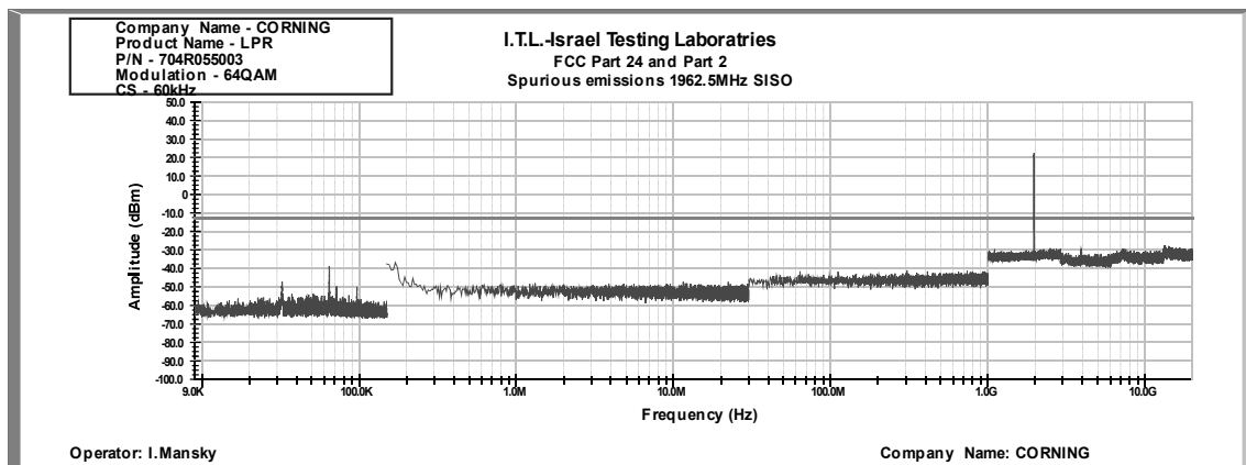
Figure 350: Spurious Emissions at Antenna Terminal 64QAM, 1962.5MHz, B.W. 10MHz, Sub Carrier 60 kHz
