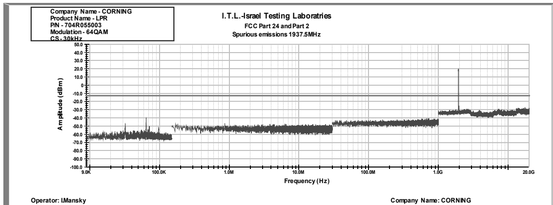
Figure 355: Spurious Emissions at Antenna Terminal 64QAM, 1937.5MHz, B.W. 15MHz, Sub Carrier 30 kHz
