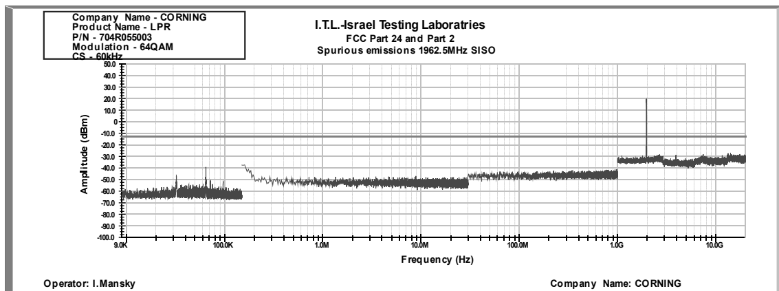
Figure 359: Spurious Emissions at Antenna Terminal 64QAM, 1962.5MHz, B.W. 15MHz, Sub Carrier 60 kHz
