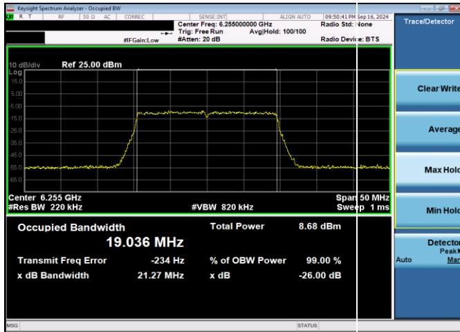
Plot 7-32. 26dB & 99% Bandwidth Plot Antenna 5T VLP (20MHz 802.11ax (UNII Band 5) – Ch. 61, MCS11)
