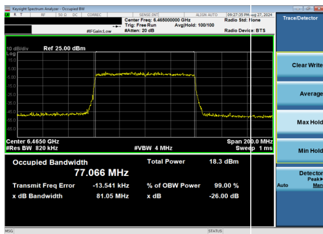
Plot 7-19. 26dB & 99% Bandwidth Plot Antenna 5T LPI (80MHz 802.11ax (UNII Band 6) – Ch. 103, MCS11)
