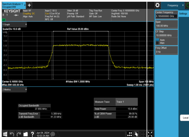
Plot 7-13. 26dB & 99% Bandwidth Plot Antenna 5T LPI (40MHz 802.11ax (UNII Band 5) – Ch. 43, MCS11)
