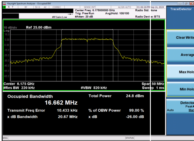
Plot 7-1. 26dB & 99% Bandwidth Plot Antenna 5T SP (20MHz 802.11a (UNII Band 5) – Ch. 45, 54Mbps)
