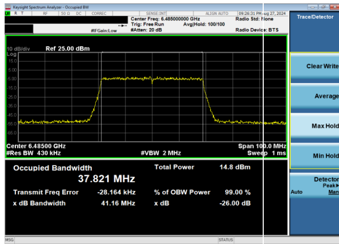
Plot 7-18. 26dB & 99% Bandwidth Plot Antenna 5T LPI (40MHz 802.11ax (UNII Band 6) – Ch. 107, MCS11)
