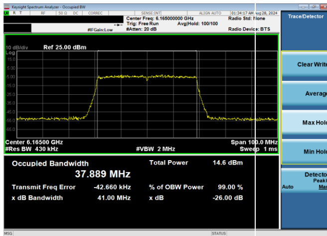
Plot 7-53. 26dB & 99% Bandwidth Plot Antenna 3b LPI (40MHz 802.11ax (UNII Band 5) – Ch. 43, MCS11)
