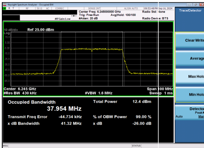
Plot 7-33. 26dB & 99% Bandwidth Plot Antenna 5T VLP (40MHz 802.11ax (UNII Band 5) – Ch. 59, MCS11)
