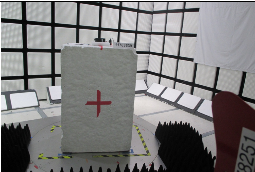
RADIATED FRONT PHOTO (ABOVE 1 GHz)
