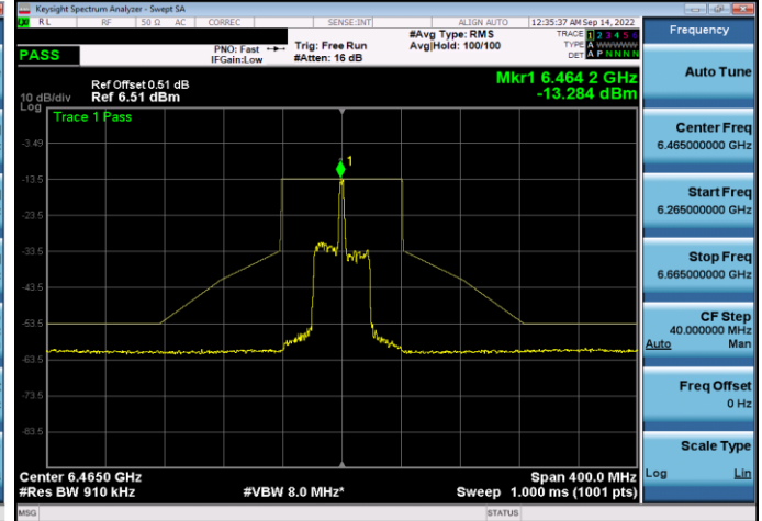
Plot 7-563. In-Band Emission Plot SDM Antenna WF5b (80MHz 802.11ax RU26 (UNII Band 6) - Ch. 103)
