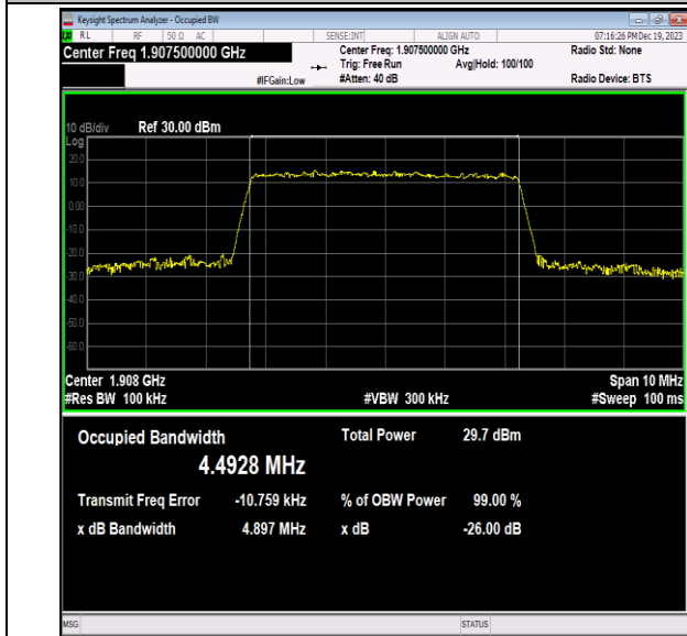
Band2-5MHz-64QAM-19175-25RB#0-PASS
