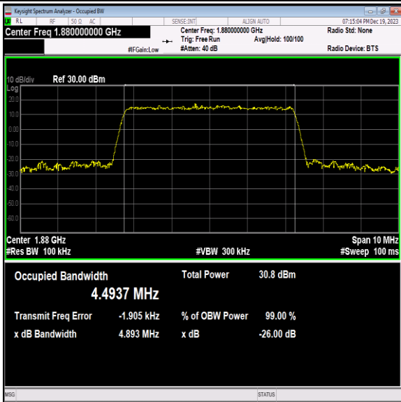
Band2-5MHz-16QAM-18900-25RB#0-PASS
