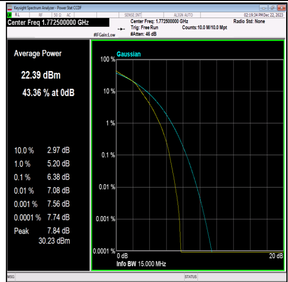
Band66-15MHz-16QAM-132597-75RB#0-PASS
