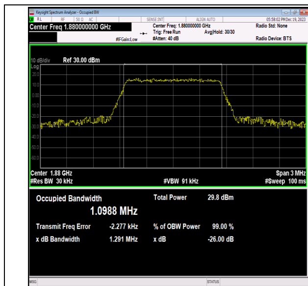
Band2-1.4MHz-16QAM-18900-6RB#0-PASS
