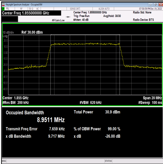
Band2-10MHz-16QAM-18650-50RB#0-PASS
