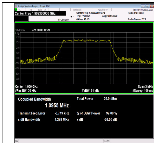
Band2-1.4MHz-64QAM-19193-6RB#0-PASS
