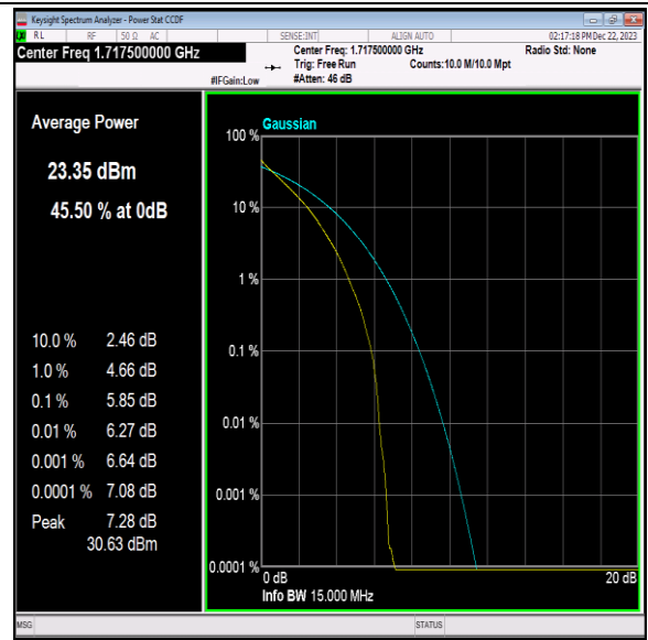
Band66-15MHz-64QAM-132047-75RB#0-PASS
