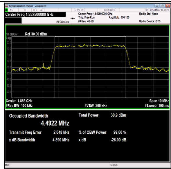
Band2-5MHz-16QAM-18625-25RB#0-PASS
