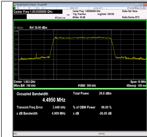
Band2-5MHz-64QAM-18625-25RB#0-PASS
