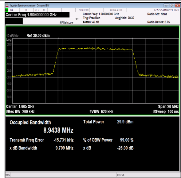
Band2-10MHz-64QAM-19150-50RB#0-PASS
