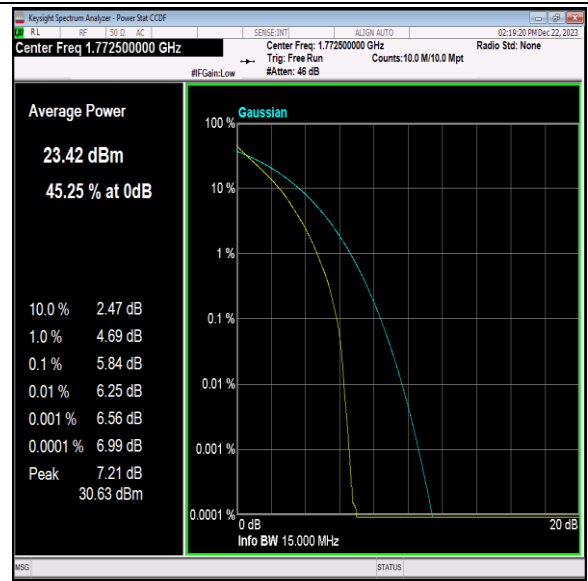
Band66-15MHz-QPSK-132597-75RB#0-PASS
