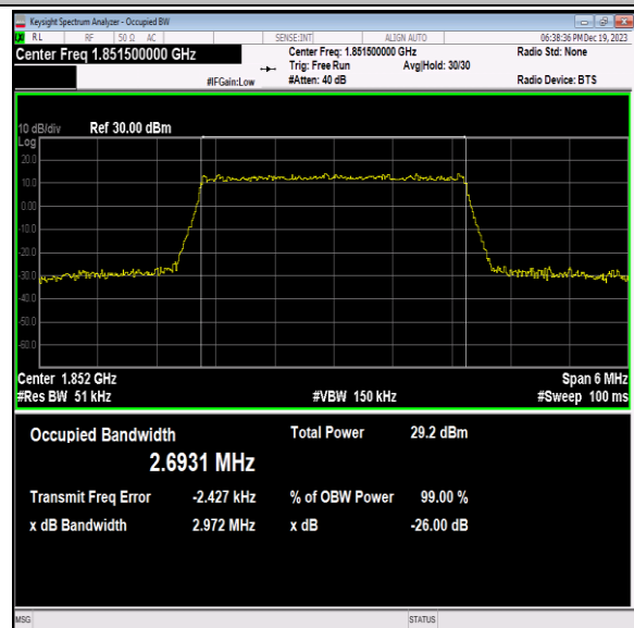
Band2-3MHz-64QAM-18615-15RB#0-PASS
