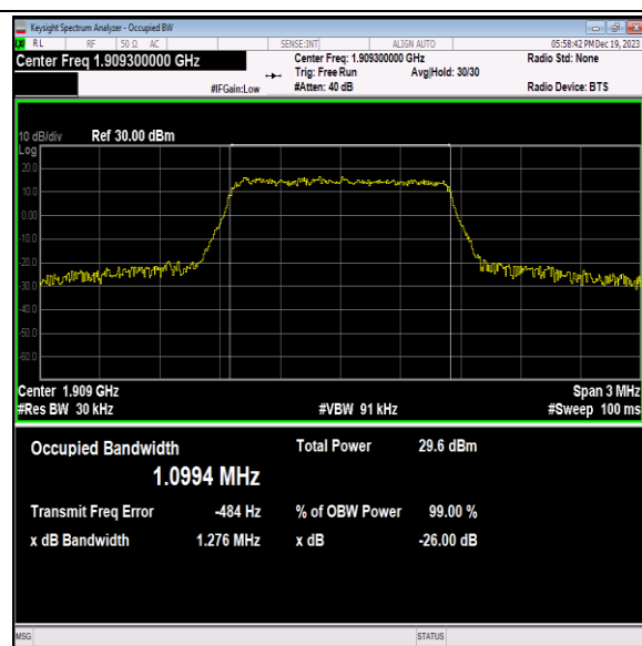
Band2-1.4MHz-16QAM-19193-6RB#0-PASS
