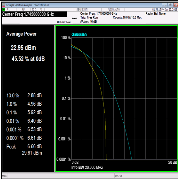
Band66-20MHz-16QAM-132322-1RB#0-PASS
