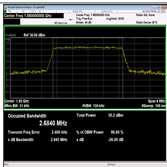
Band2-3MHz-16QAM-18900-15RB#0-PASS
