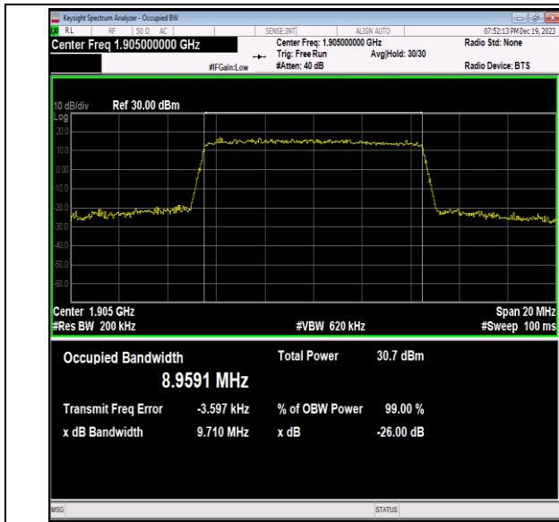
Band2-10MHz-16QAM-19150-50RB#0-PASS
