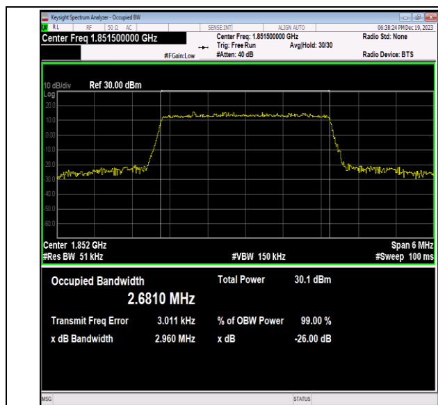
Band2-3MHz-16QAM-18615-15RB#0-PASS
