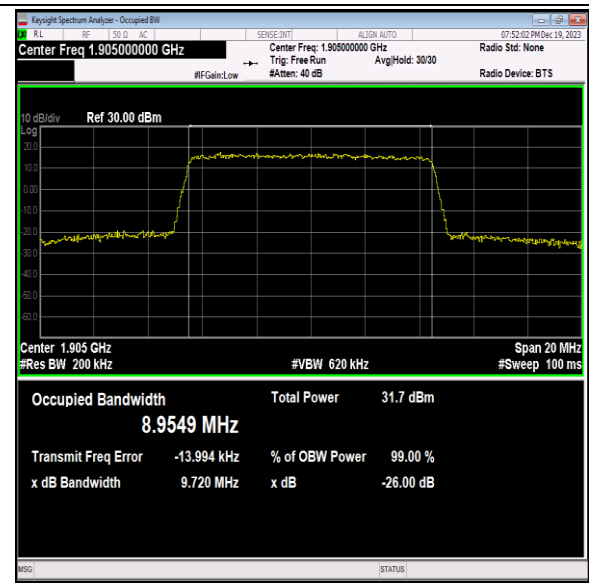
Band2-10MHz-QPSK-19150-50RB#0-PASS
