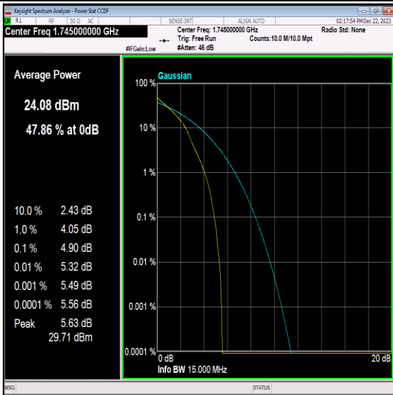
Band66-15MHz-64QAM-132322-1RB#0-PASS
