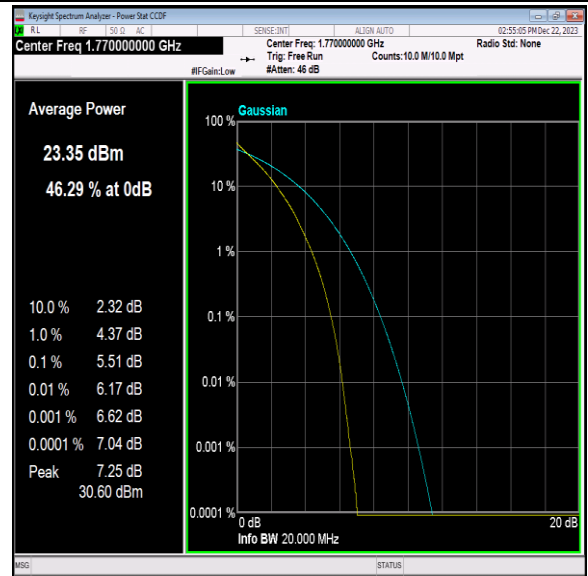
Band66-20MHz-64QAM-132572-100RB#0-PASS
