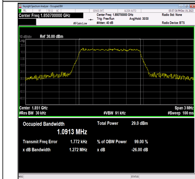
Band2-1.4MHz-64QAM-18607-6RB#0-PASS
