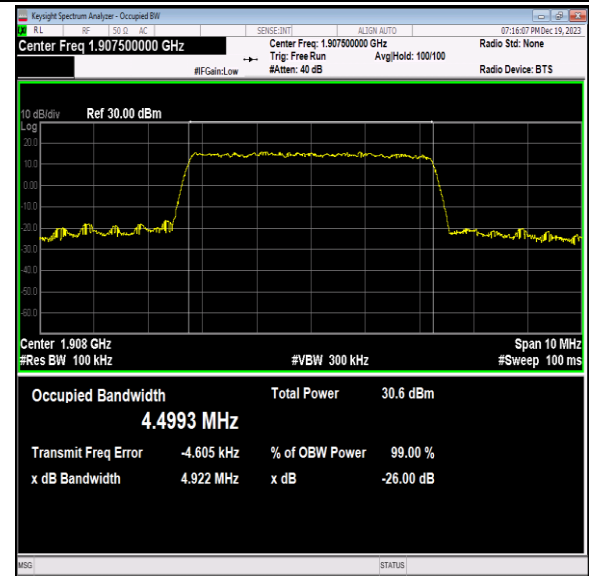
Band2-5MHz-16QAM-19175-25RB#0-PASS
