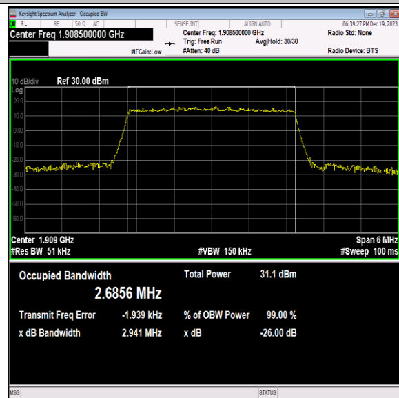
Band2-3MHz-QPSK-19185-15RB#0-PASS
