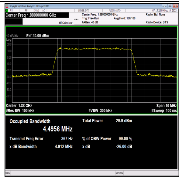
Band2-5MHz-64QAM-18900-25RB#0-PASS
