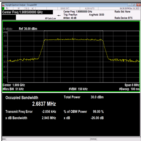
Band2-3MHz-16QAM-19185-15RB#0-PASS
