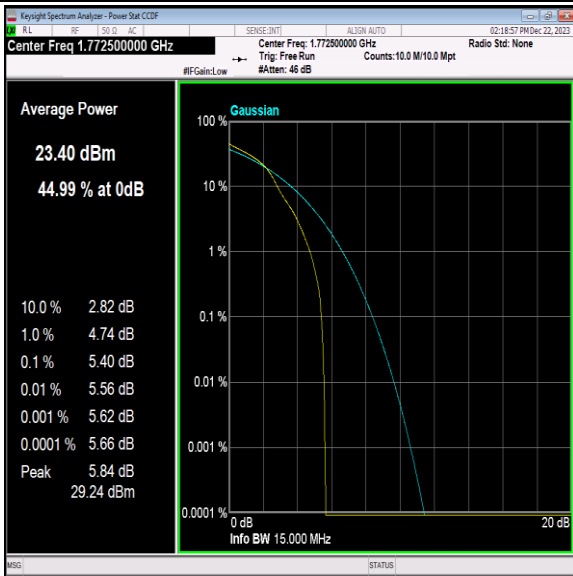
Band66-15MHz-16QAM-132597-1RB#0-PASS
