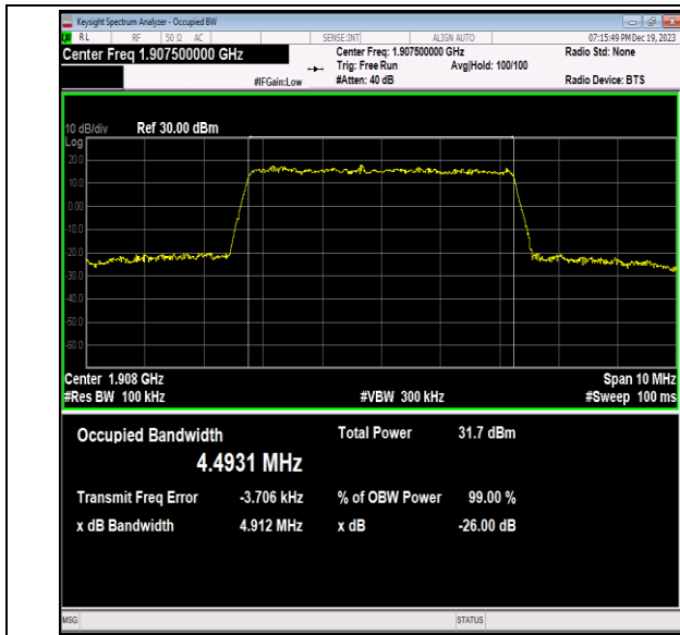
Band2-5MHz-QPSK-19175-25RB#0-PASS
