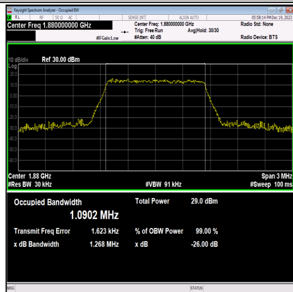
Band2-1.4MHz-64QAM-18900-6RB#0-PASS
