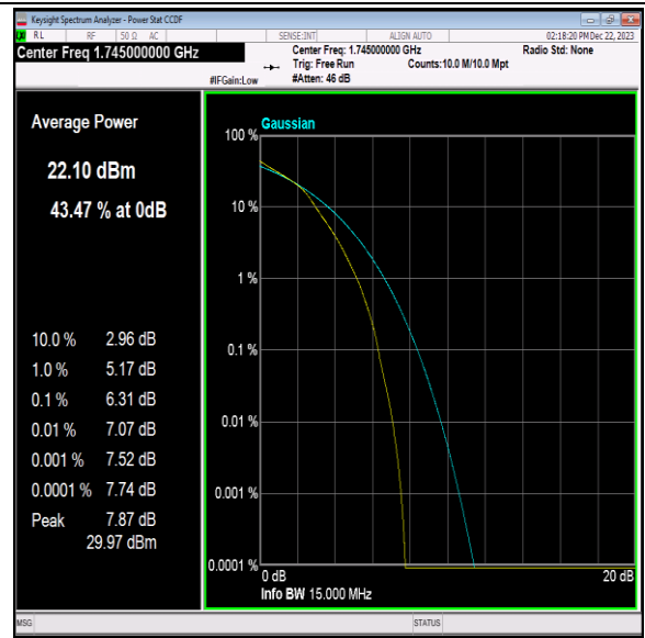
Band66-15MHz-16QAM-132322-75RB#0-PASS
