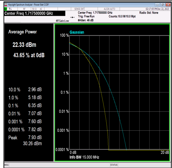
Band66-15MHz-16QAM-132047-75RB#0-PASS
