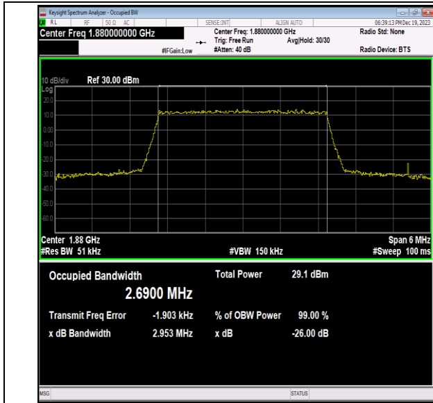
Band2-3MHz-64QAM-18900-15RB#0-PASS
