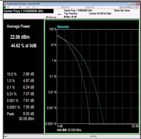
Band66-20MHz-16QAM-132322-100RB#0-PASS
