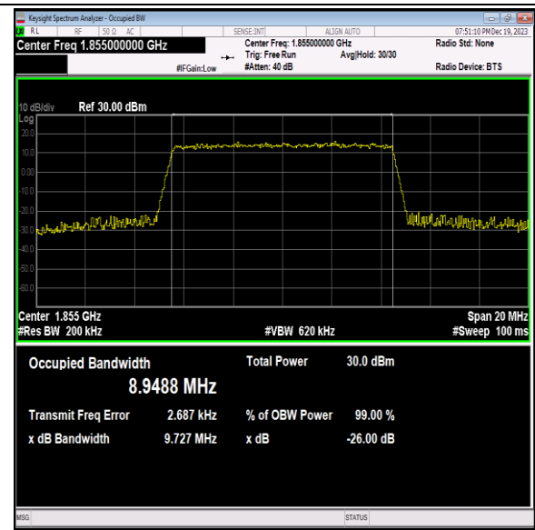
Band2-10MHz-64QAM-18650-50RB#0-PASS
